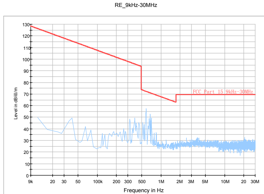
Fig.20. Radiated emission: GFSK, 2440MHz, 9 KHz - 30 MHz
