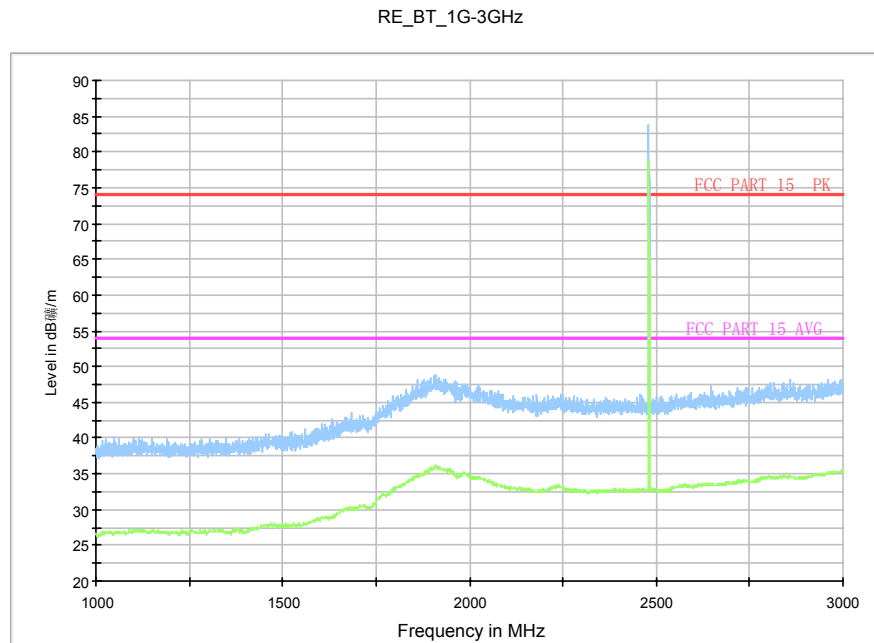
Fig.24. Radiated emission: GFSK, 2480MHz, 1 GHz - 3 GHz
