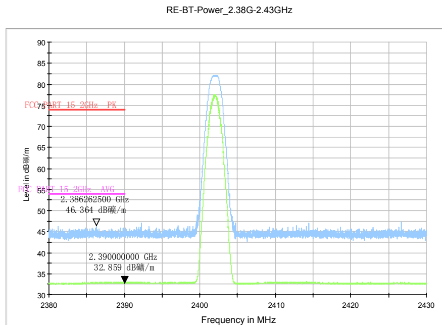
Fig.26. Radiated emission (Power): GFSK low channel
