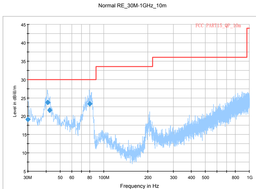
Fig.21. Radiated emission: GFSK, 2440MHz, 30 MHz - 1 GHz
