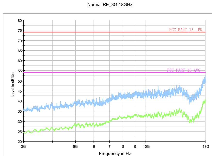
Fig.23. Radiated emission: GFSK, 2440MHz, 3 GHz - 18 GHz
