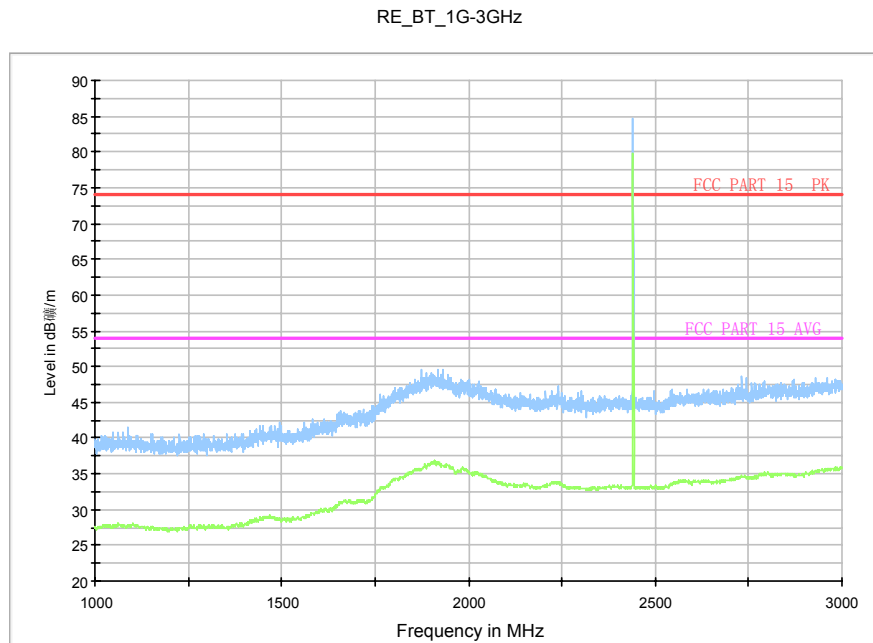
Fig.22. Radiated emission: GFSK, 2440MHz, 1 GHz - 3 GHz
