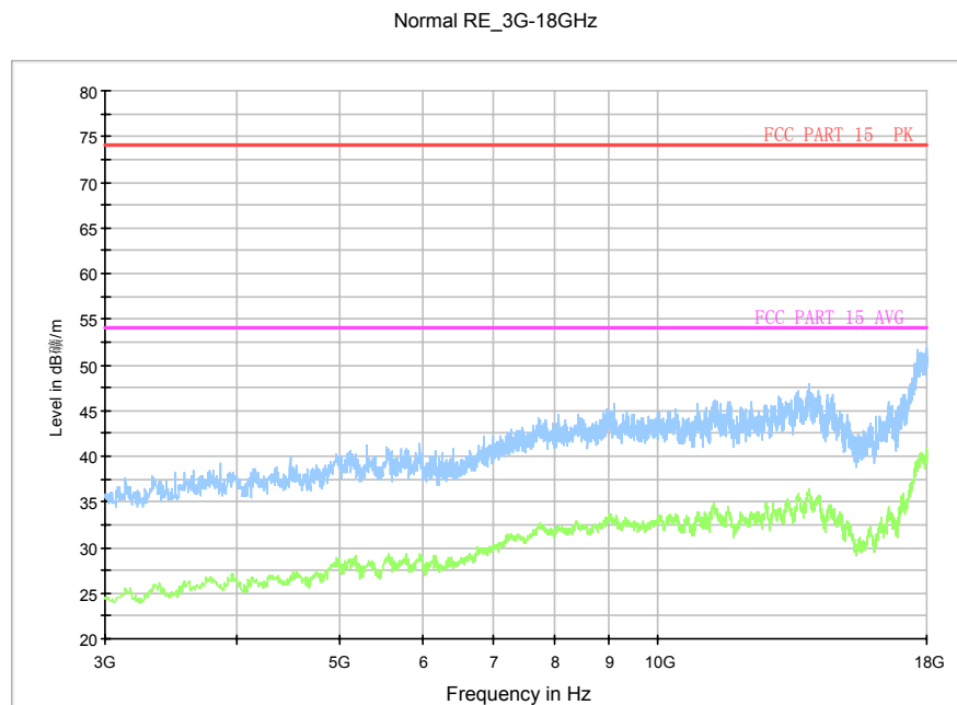
Fig.25. Radiated emission: GFSK, 2480MHz, 3 GHz - 18 GHz
