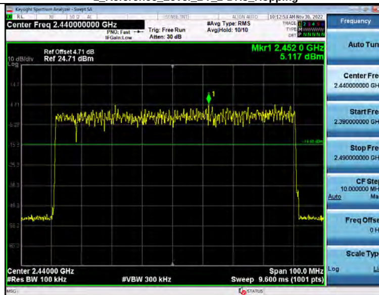
2_Band_Edge_(Hopping)_BT_2-DH5_Hopping
