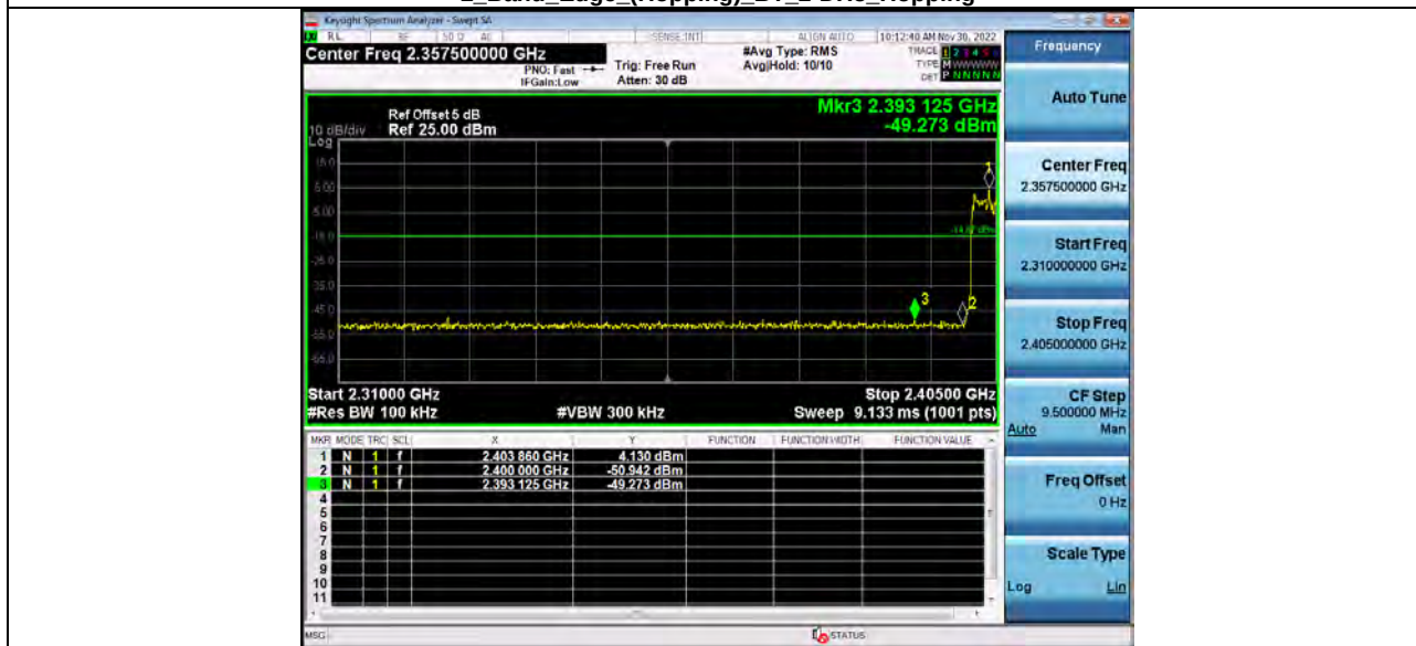
2 Band_Edge_(Hopping)_BT_2-DH5_Hopping
