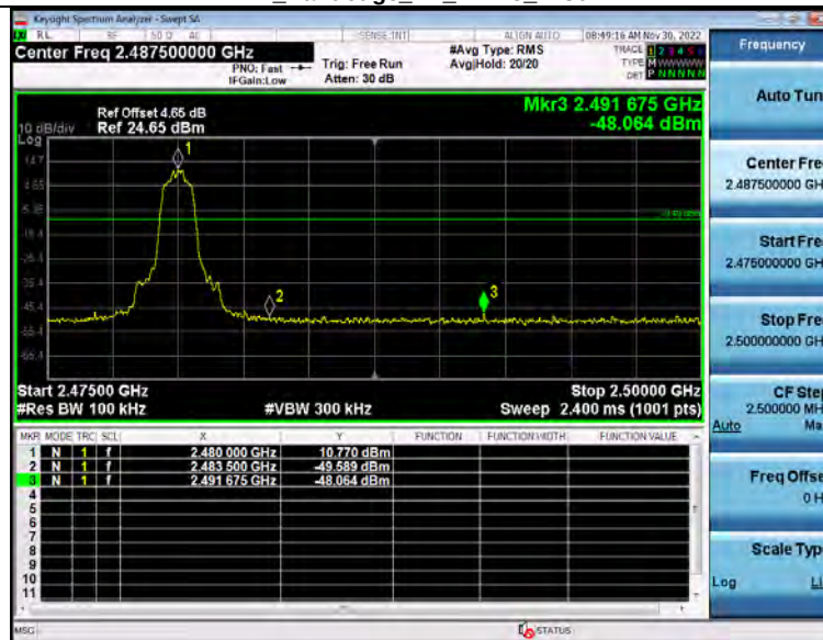
2_Bandedge_BT_2-DH5_2480
