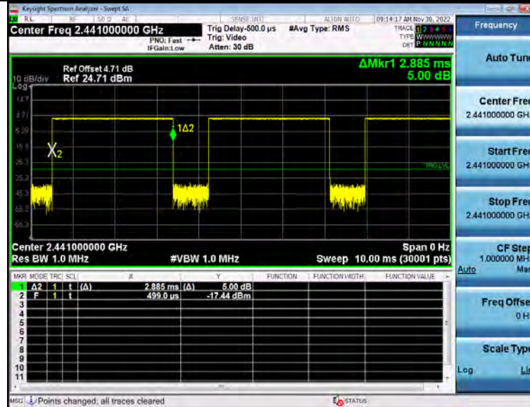
Dwell_Time (Hopping) BT_1-DH5_2441_One_Burst_Time
