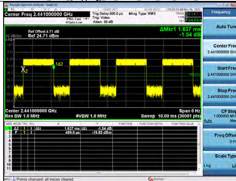
Dwell_Time (Hopping) BT_1-DH3_2441_One_Burst_Time
