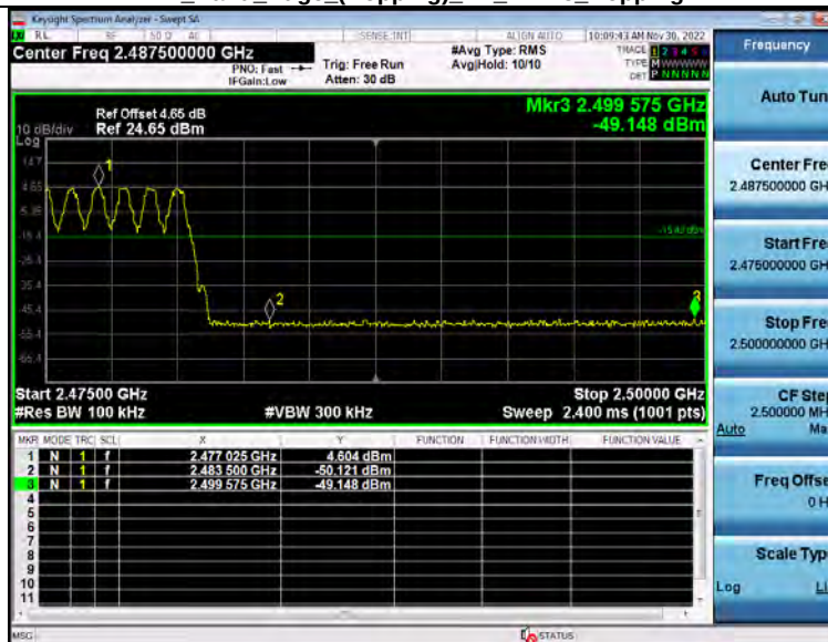
2_Band_Edge_(Hopping)_BT_1-DH5_Hopping
