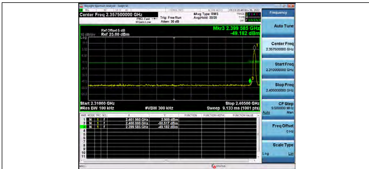
1 Reference_Level_BT_2-DH5_Hopping
