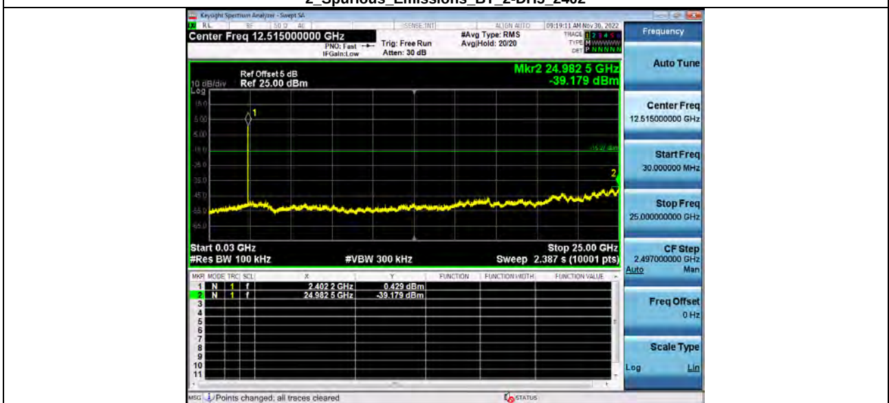
2 Spurious Emissions BT 2-DH5 2402
