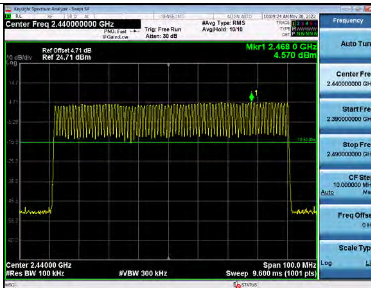
2_Band_Edge_(Hopping)_BT_1-DH5_Hopping
