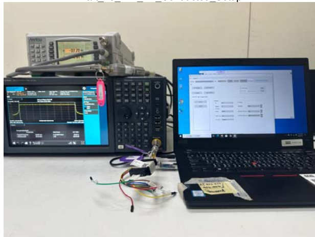
Part 15 247 BT Conduction Setup
