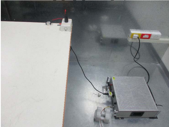
Part 15_247 LE Conduction Setup
