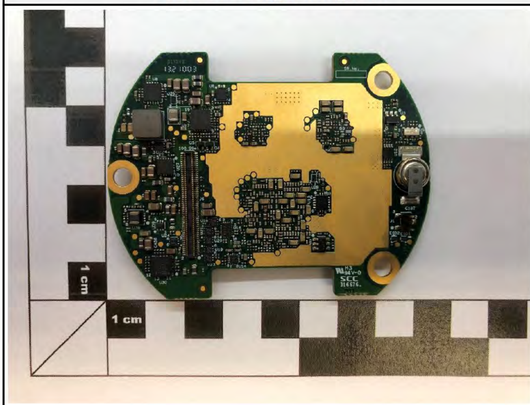
ProcessorPCBA_Bottom_Zoom
