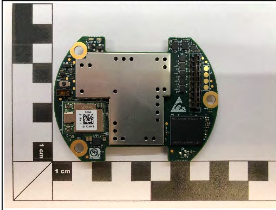
ProcessorPCBA_Top_withShielding_Zoom
