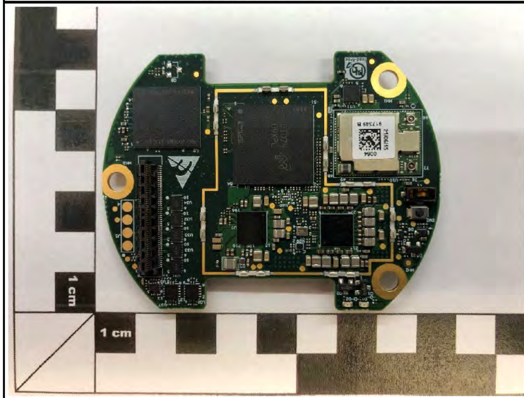
ProcessorPCBA_Top_withoutShielding_Zoom
