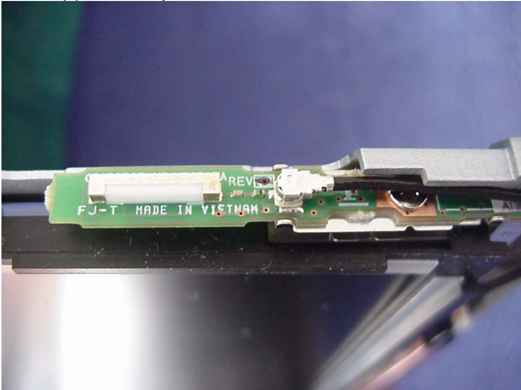
Antenna (R) location – exploded view
