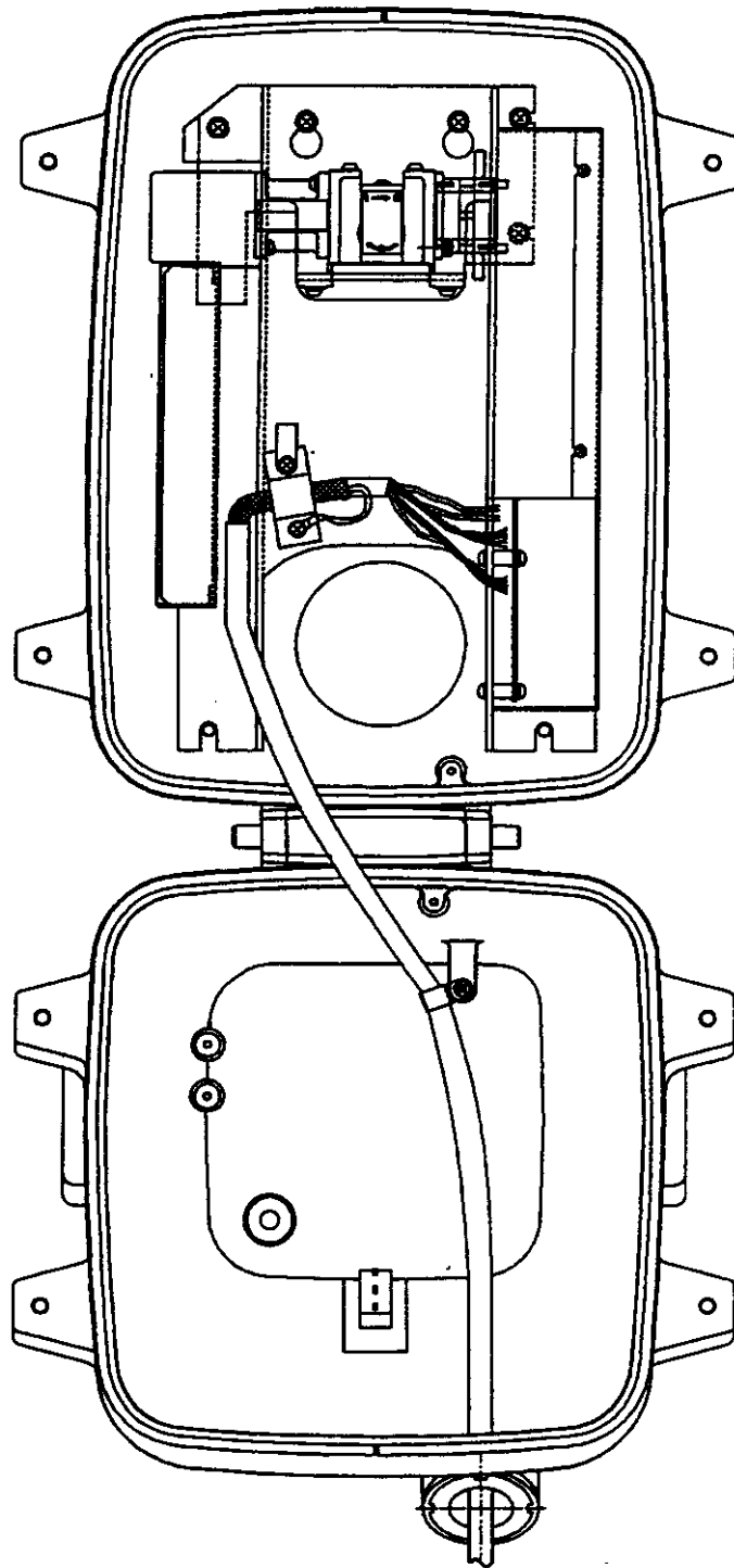
FIG. 4.3 ASSEMBLING PROCEDURE FOR CABLE
