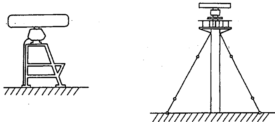
FIG. 2.2 SCANNER STAND
