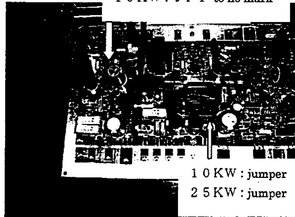
FIG. 6. 2 SETTING OF POWER SUPPLY
