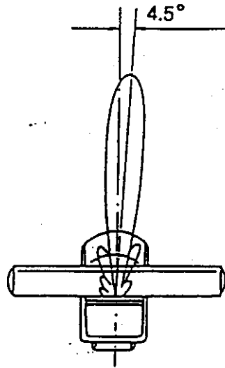
Fig. 4-1 RADIATOR
