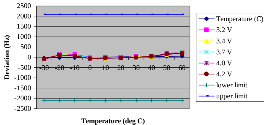
Transmitter Carrier Frequency Deviation (Hz)
