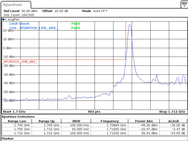
5MHz_15kHz_1712.5MHz_DFT-s-OFDM QPSK_RB1@0&-16.47 dBm
