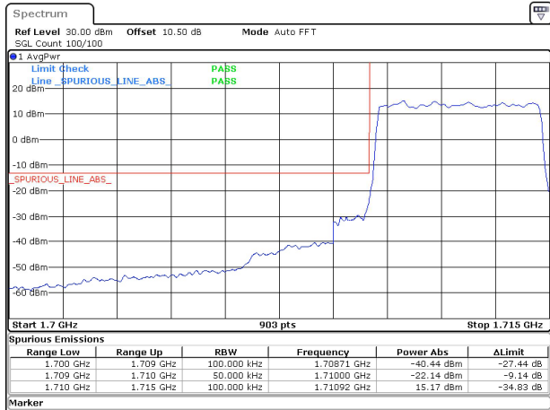
5MHz_15kHz_1712.5MHz_DFT-s-OFDM QPSK_RB25@0&-22.14 dBm
