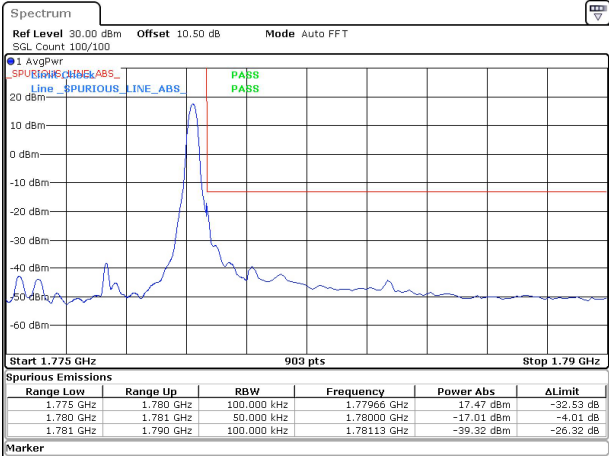
5MHz_15kHz_1777.5MHz_DFT-s-OFDM QPSK_RB1@24&-17.01 dBm
