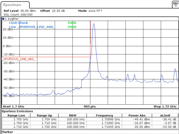
10MHz_15kHz_1715MHz_DFT-s-OFDM QPSK_RB1@0&-16.67 dBm
