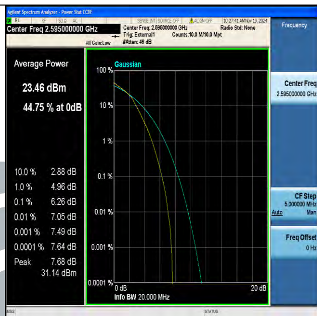
Band38-20MHz-16QAM-38000-100RB#0-PASS
