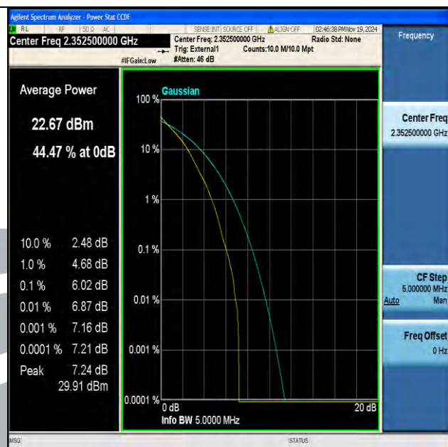
Band40(2350-2360)-5MHz-QPSK-39175-25RB#0-PASS
