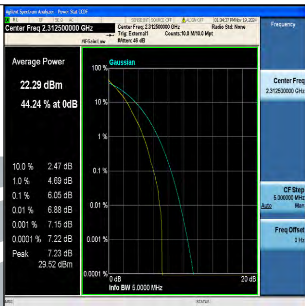
Band40(2305-2315)-5MHz-QPSK-38775-25RB#0-PASS
