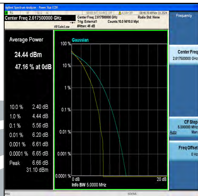
Band38-5MHz-QPSK-38225-25RB#0-PASS
