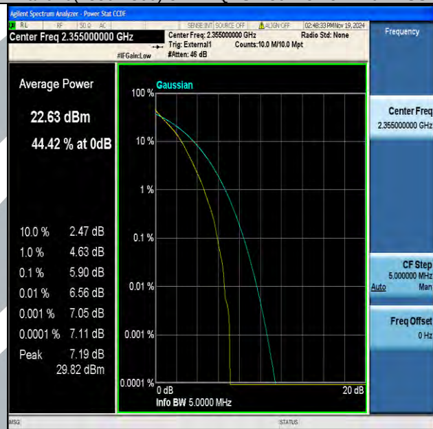
Band40(2350-2360)-5MHz-QPSK-39200-25RB#0-PASS
