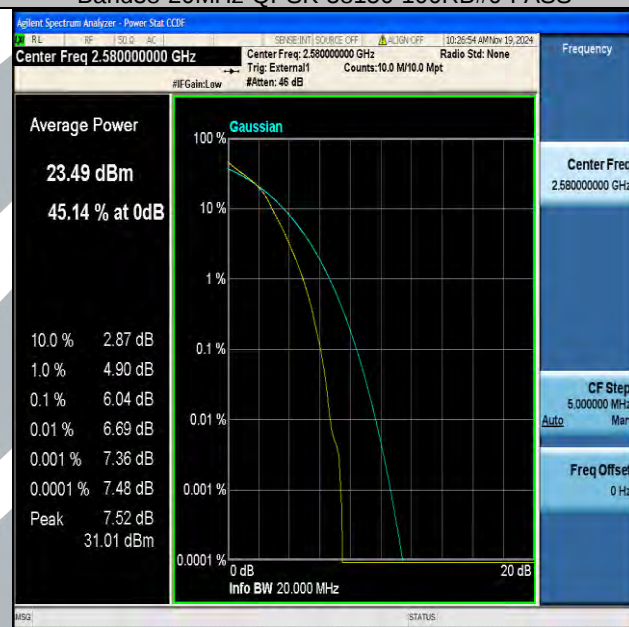
Band38-20MHz-16QAM-37850-100RB#0-PASS
