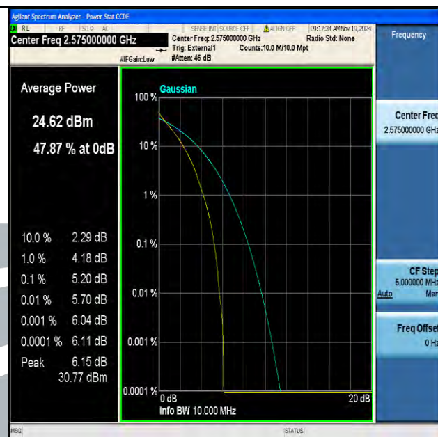
Band38-10MHz-QPSK-37800-50RB#0-PASS
