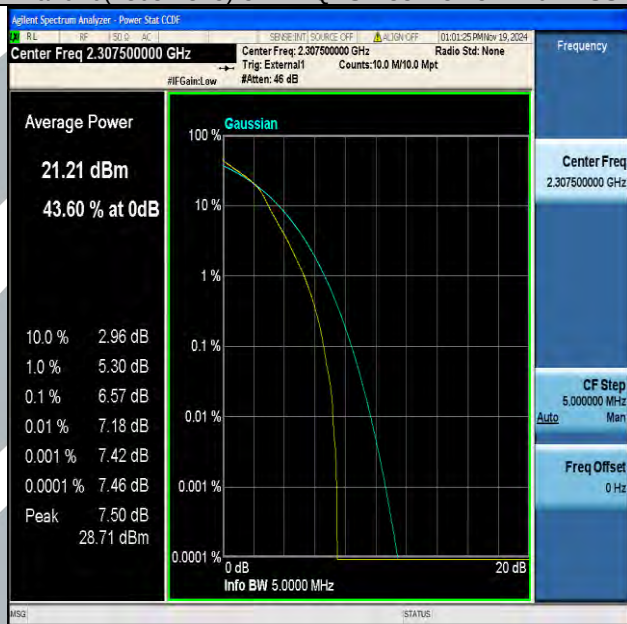
Band40(2305-2315)-5MHz-16QAM-38725-25RB#0-PASS
