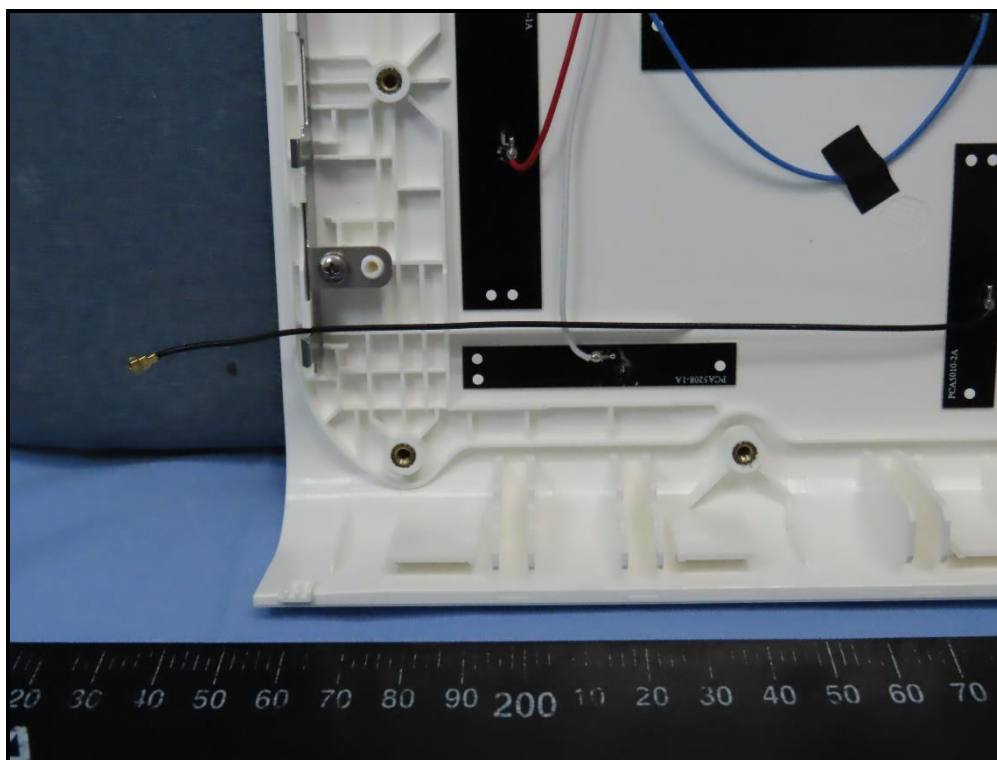
WiFi 1 Antenna
