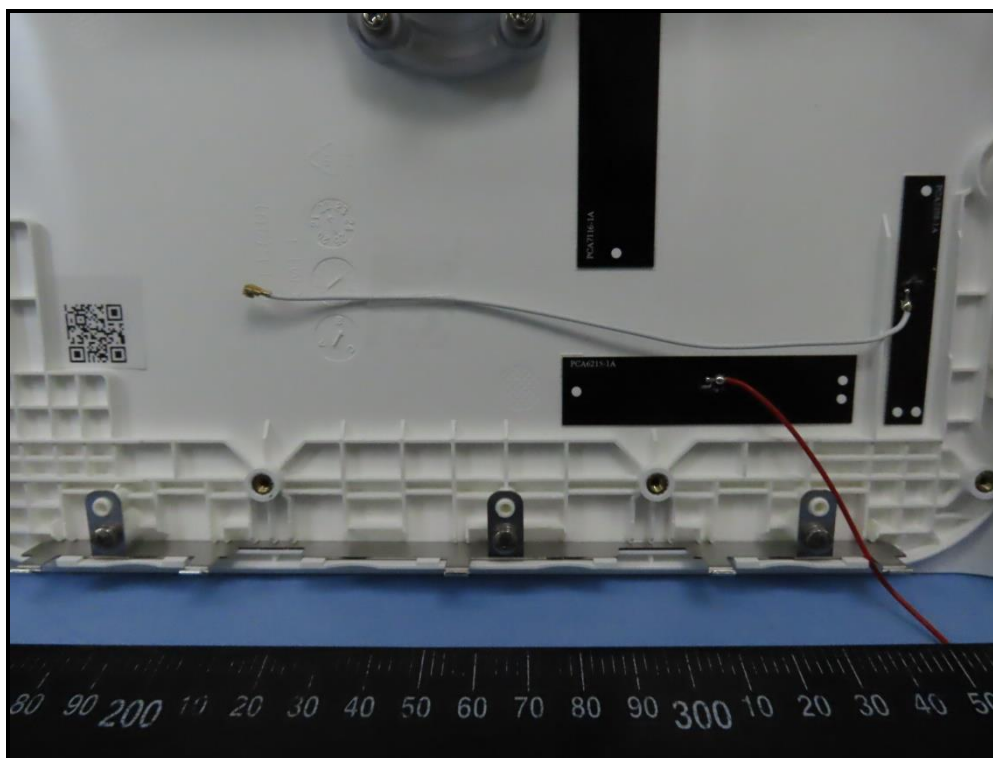
WiFi 0 Antenna
