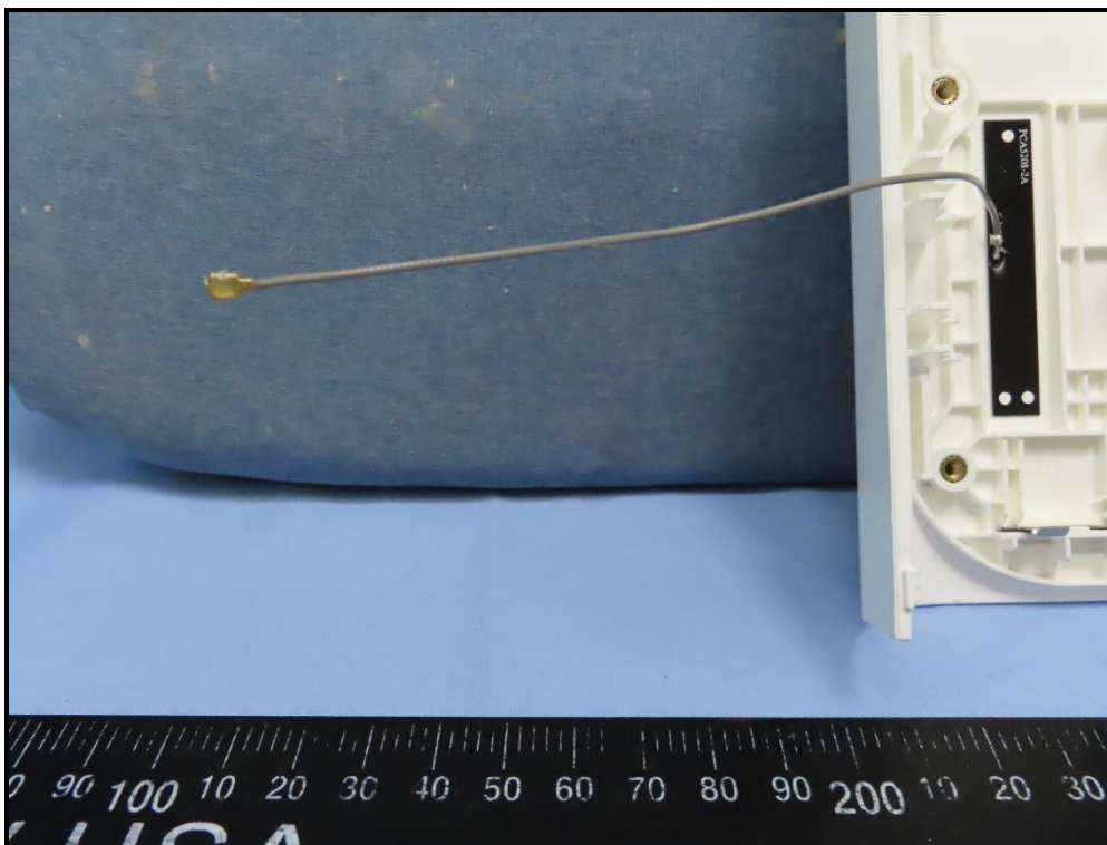
BT Antenna
