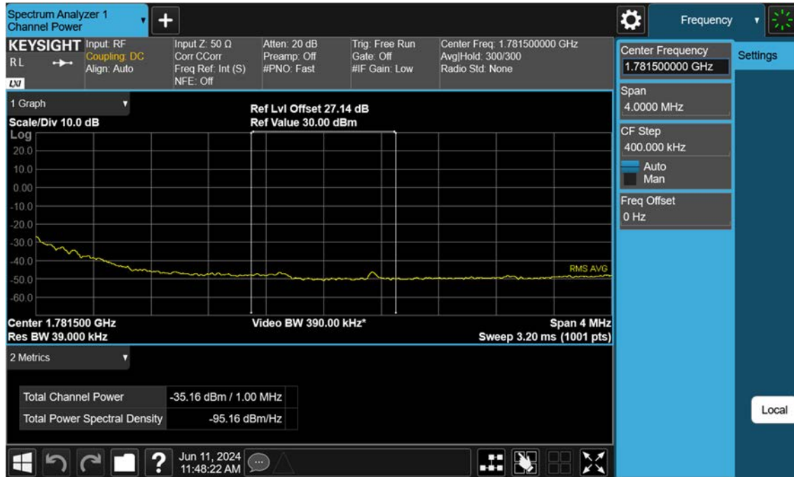
Sub6 n66_10 M_Extended Band Edge_High_BPSK_FullRB
