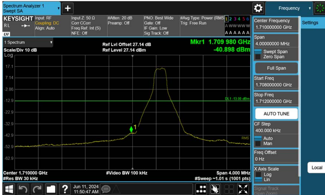
Sub6 n66_15 M_Band Edge_Low_BPSK_1RB
