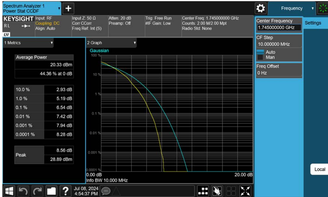
Sub6 n66_10 M_PAR_Mid_64QAM_FullRB
