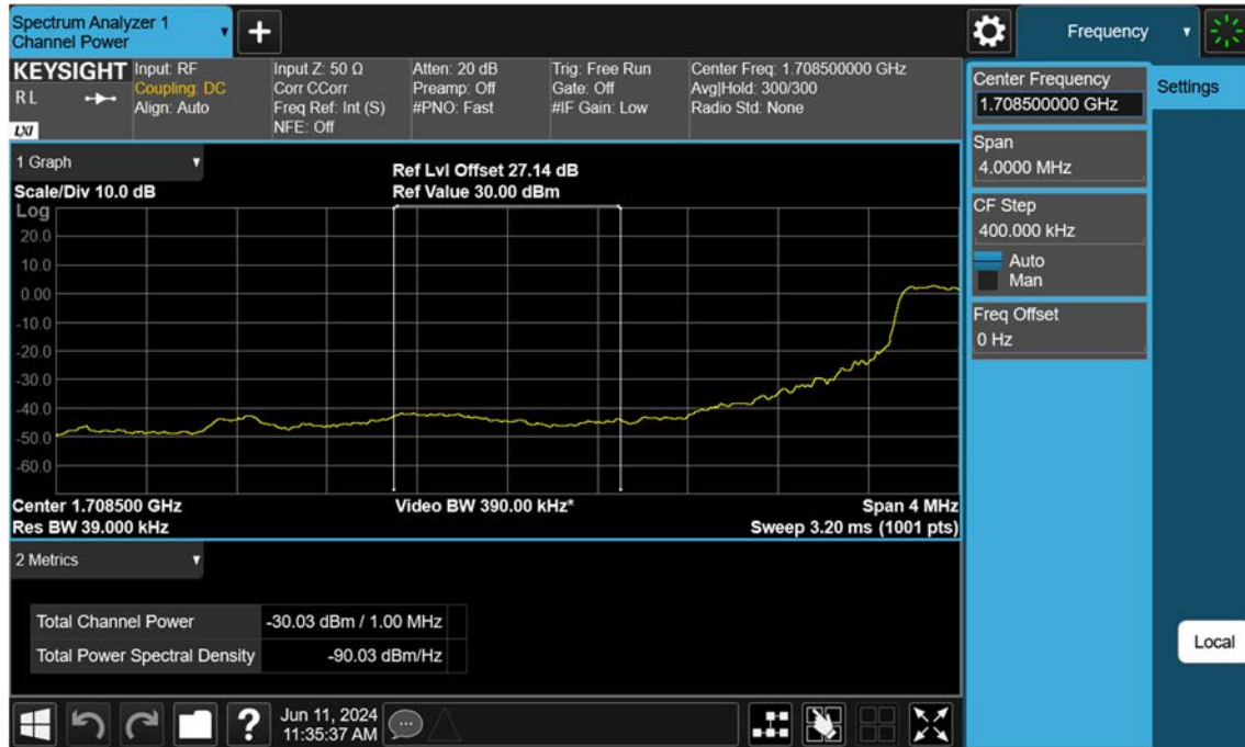
Sub6 n66_5 M_Extended Band Edge_Low_BPSK_FullIRB
