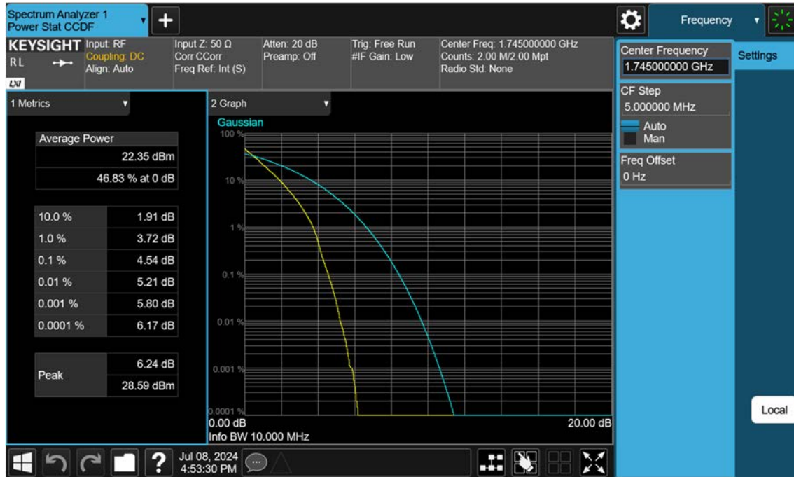
Sub6 n66_10 M_PAR_Mid_BPSK_FullRB
