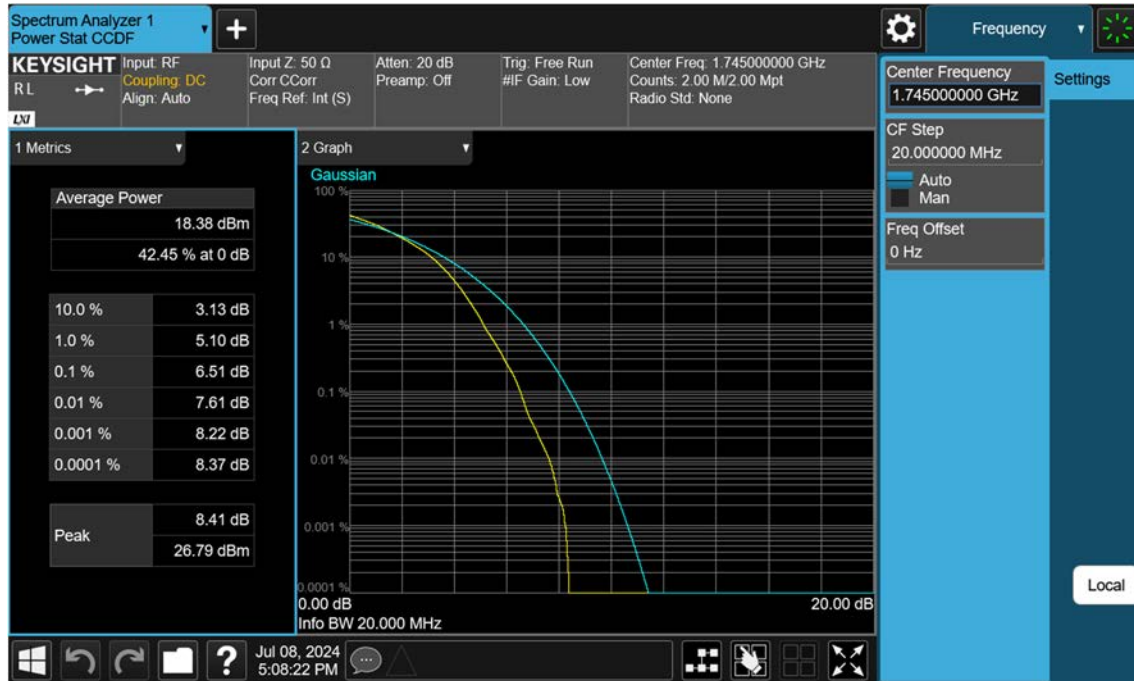
Sub6 n66_20 M_PAR_Mid_256QAM_FullRB
