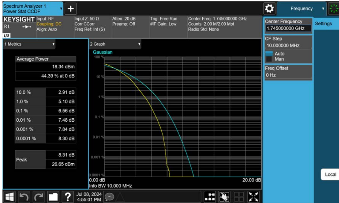
Sub6 n66_10 M_PAR_Mid_256QAM_FullRB
