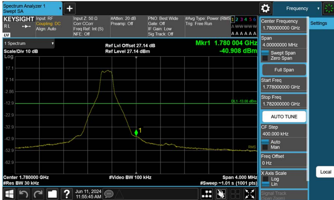
Sub6 n66_15 M_Band Edge_High_BPSK_1RB
