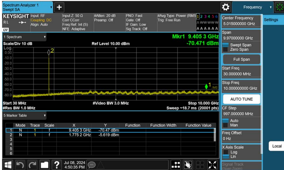
Sub6 n66_5 M_Conducted Spurious(30 M-10 G)_High_BPSK_1RB
