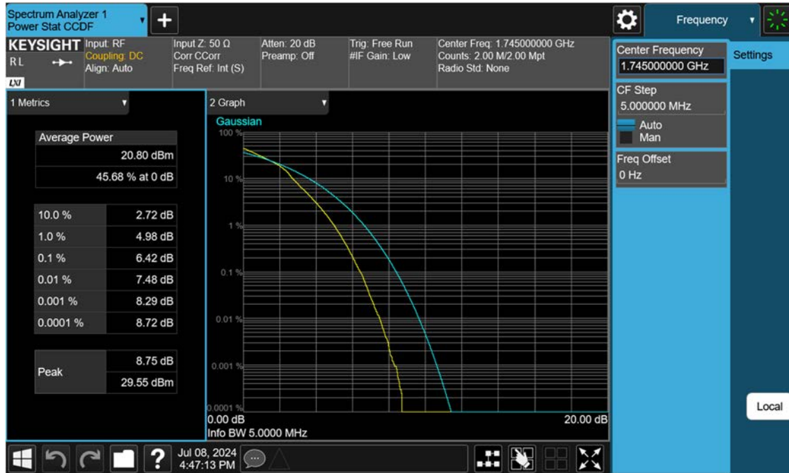
Sub6 n66_5 M_PAR_Mid_16QAM_FullRB
