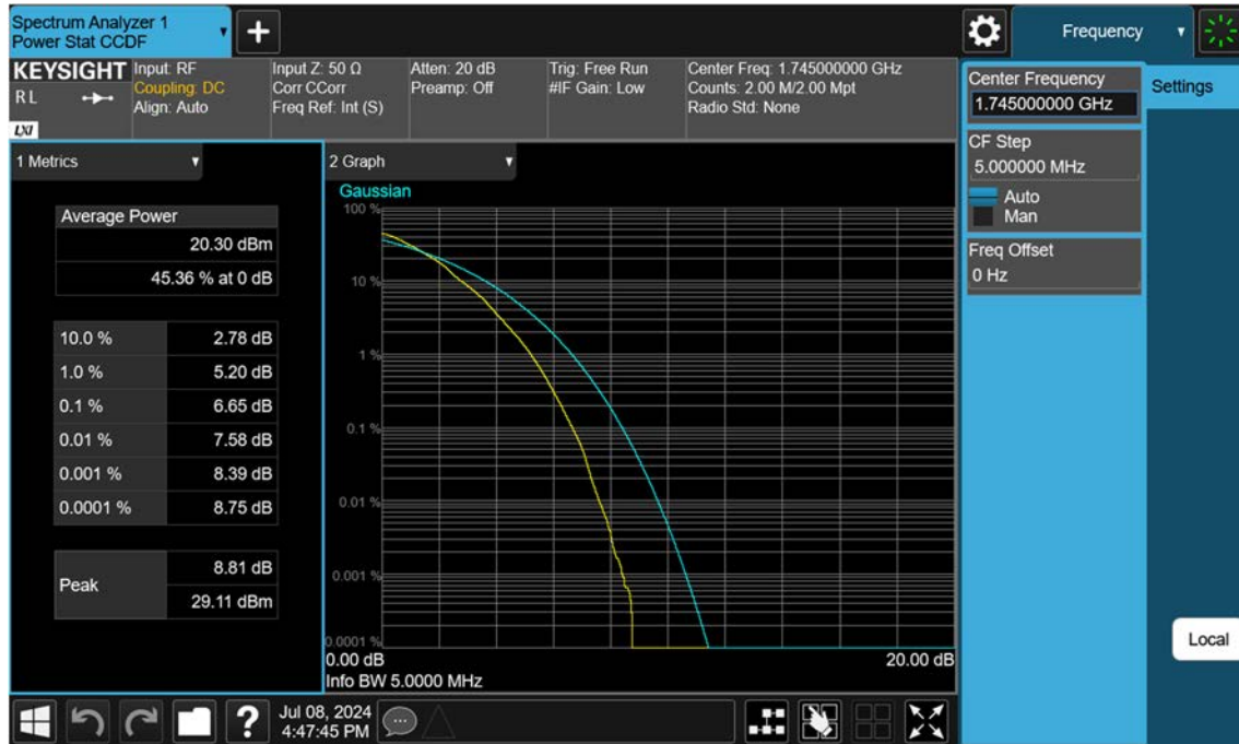
Sub6 n66_5 M_PAR_Mid_64QAM_FullRB
