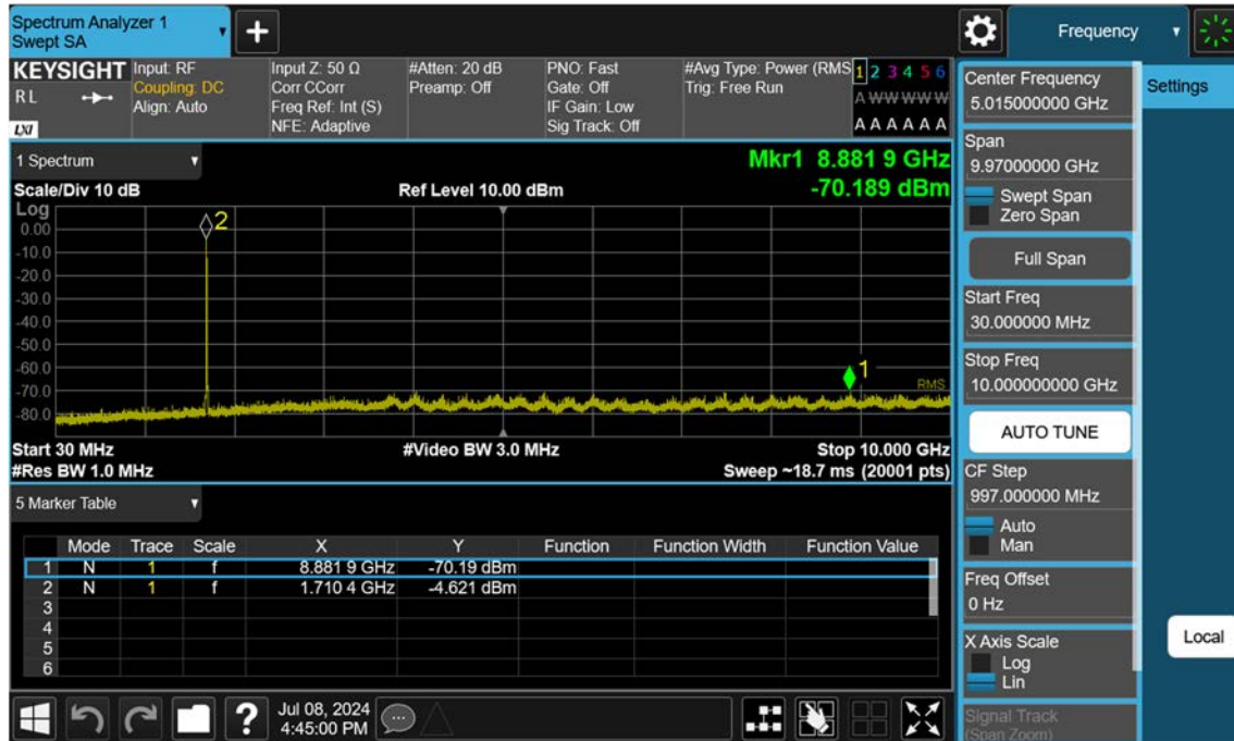
Sub6 n66_5 M_Conducted Spurious(30 M-10 G)_Low_BPSK_1RB
