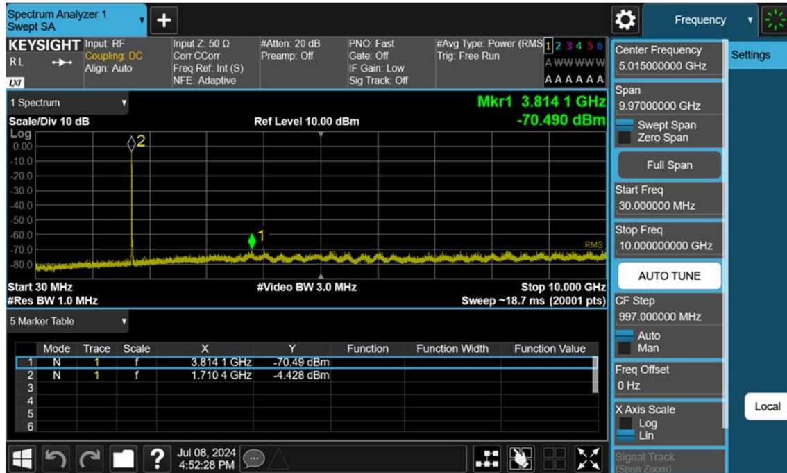
Sub6 n66_10 M_Conducted Spurious(30 M-10 G)_Low_BPSK_1RB
