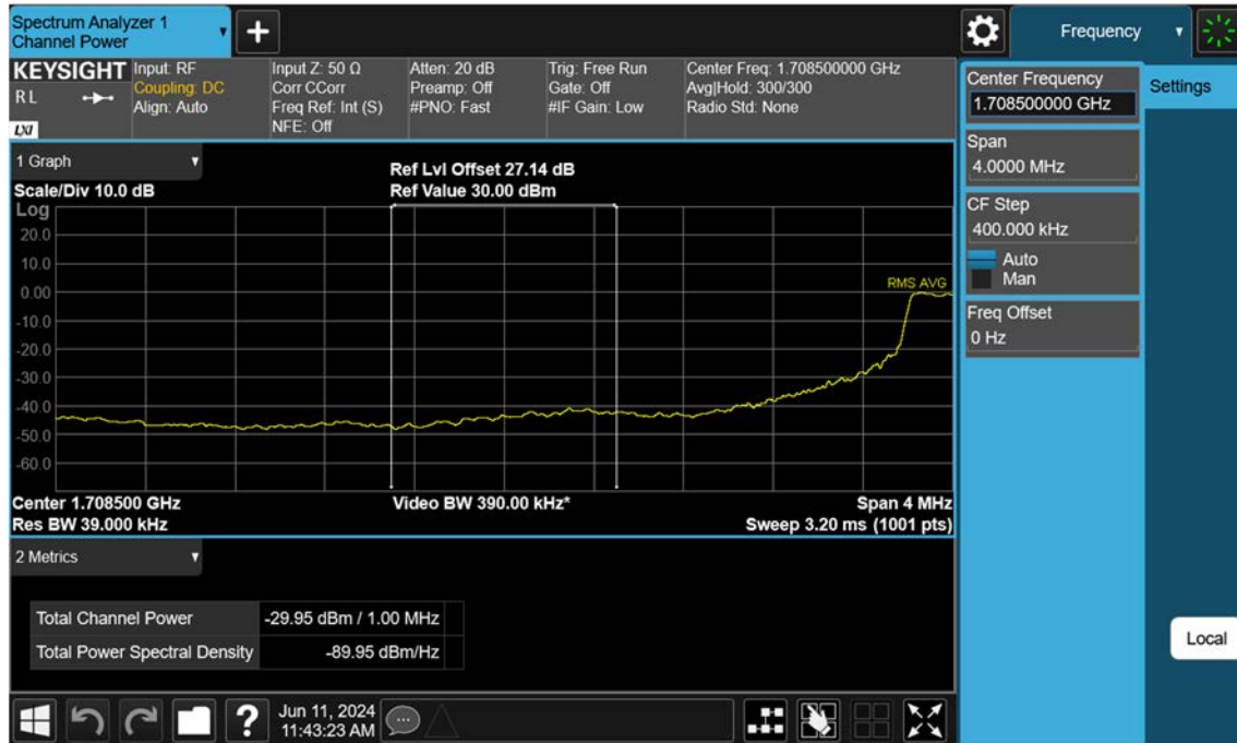
Sub6 n66_10 M_Extended Band Edge_Low_BPSK_FullRB
