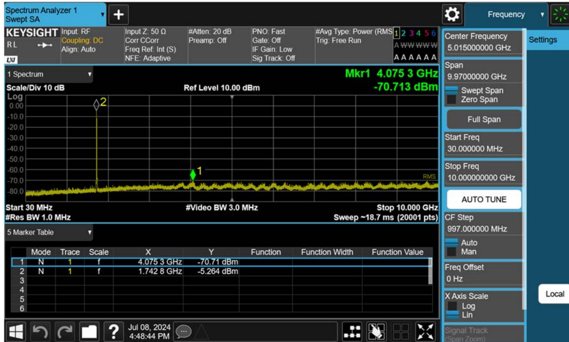
Sub6 n66_5 M_Conducted Spurious(30 M-10 G)_Mid_BPSK_FullRB
