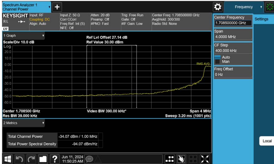
Sub6 n66_15 M_Extended Band Edge_Low_BPSK_FullRB
