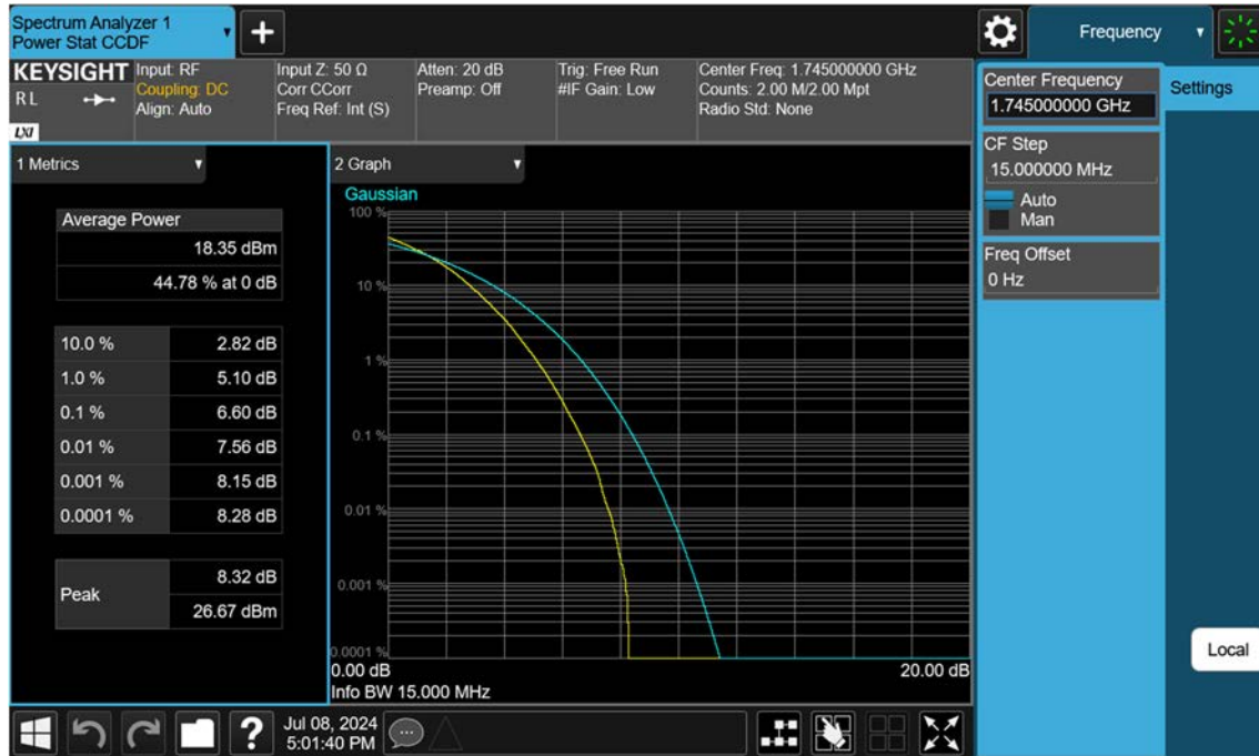
Sub6 n66_15 M_PAR_Mid_256QAM_FullRB
