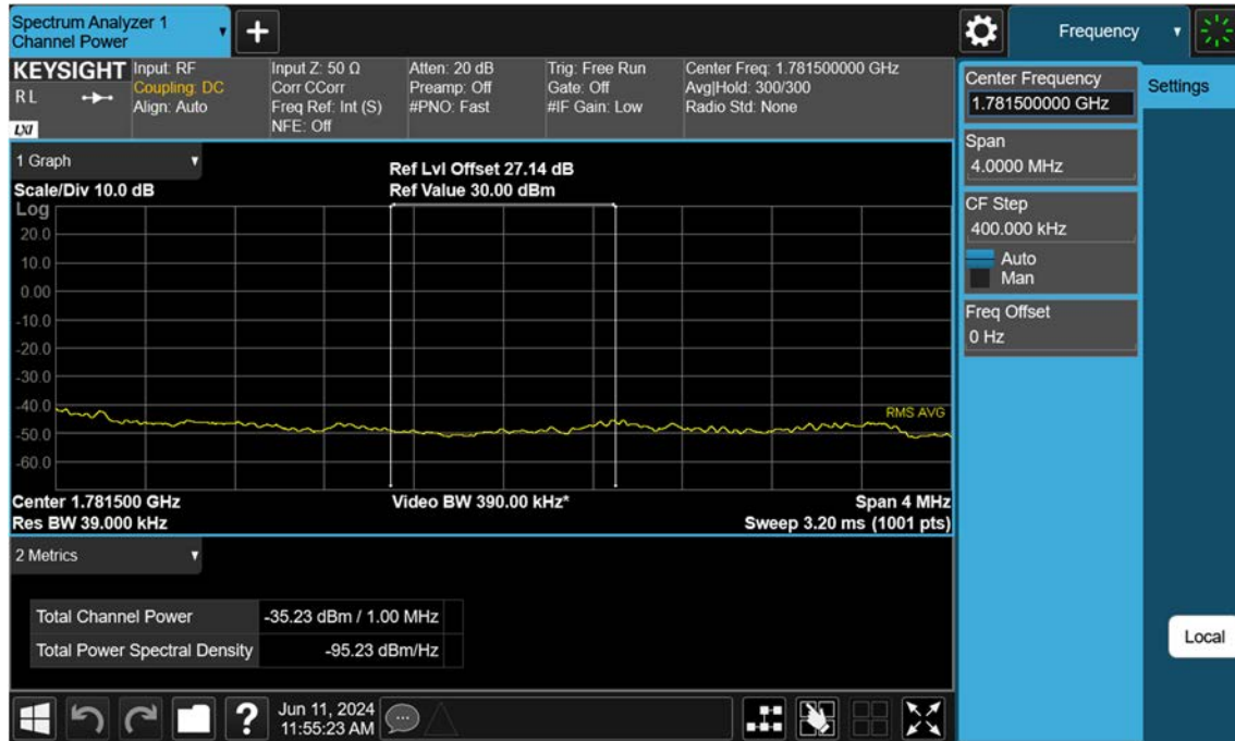
Sub6 n66_15 M_Extended Band Edge_High_BPSK_FullRB
