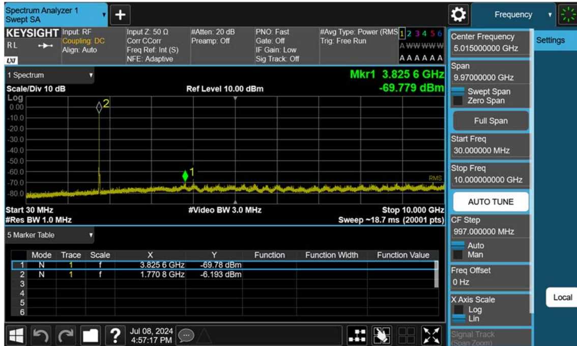
Sub6 n66_10 M_Conducted Spurious(30 M-10 G)_High_BPSK_1RB
