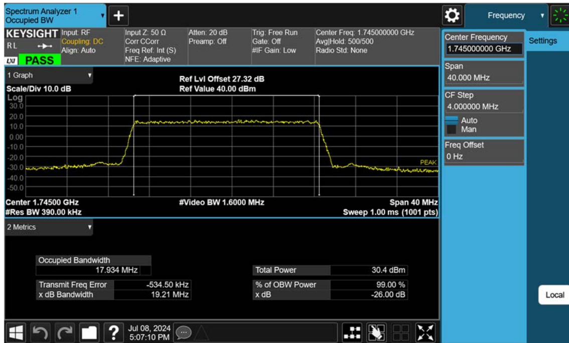
Sub6 n66_20 M_OBW_Mid_QPSK_FullRB
