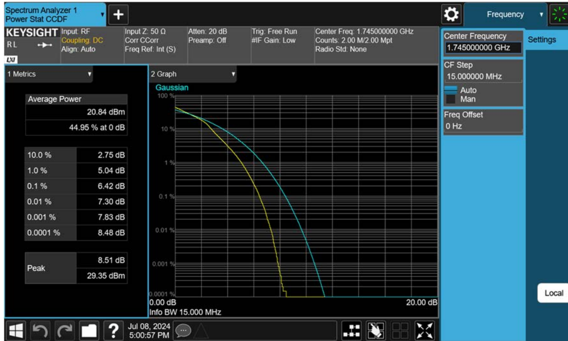
Sub6 n66_15 M_PAR_Mid_16QAM_FullRB
