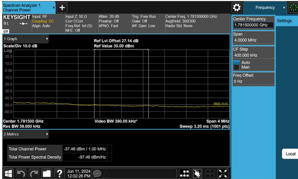
Sub6 n66_20 M_Extended Band Edge_High_BPSK_FullRB
