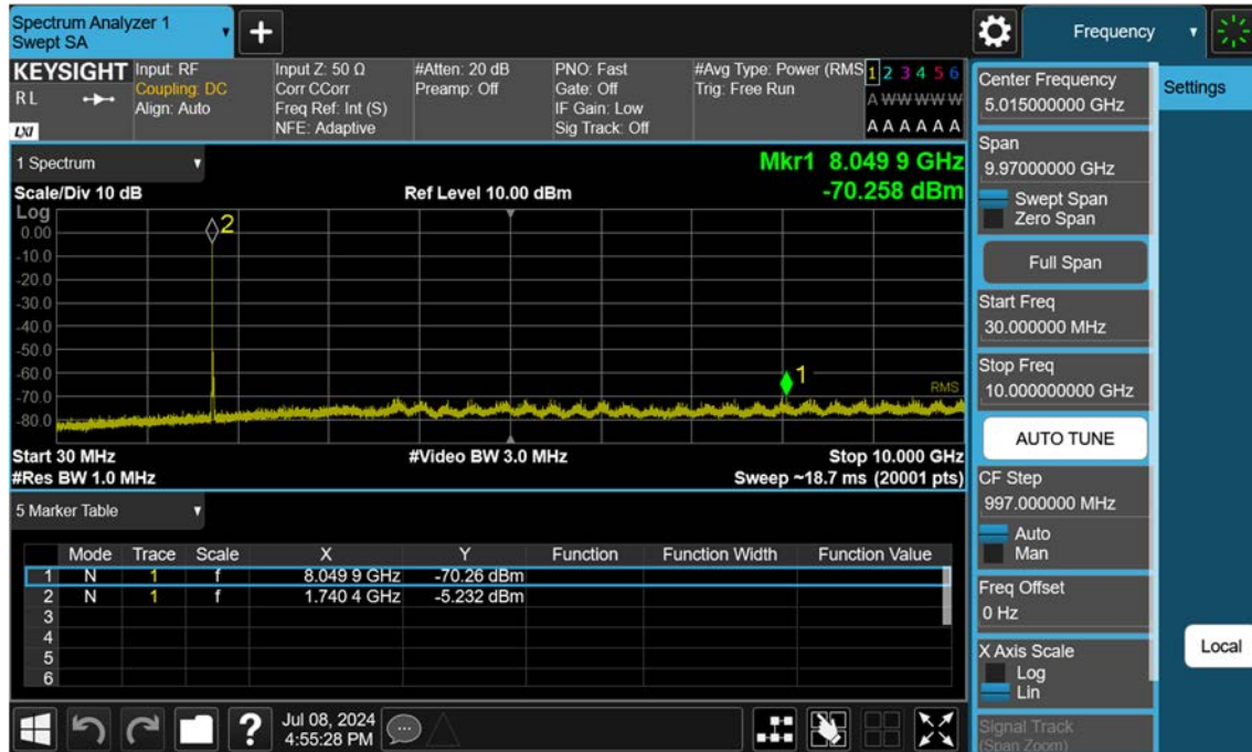
Sub6 n66_10 M_Conducted Spurious(30 M-10 G)_Mid_BPSK_FullRB
