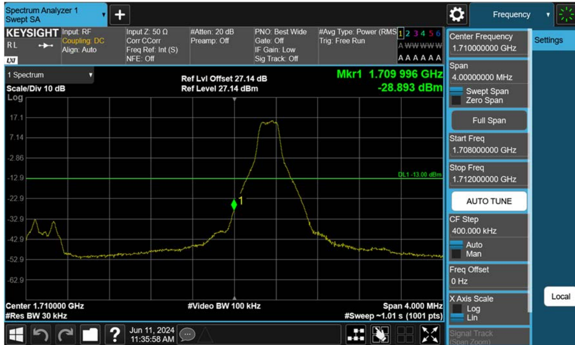
Sub6 n66_5 M_Band Edge_Low_BPSK_1RB
