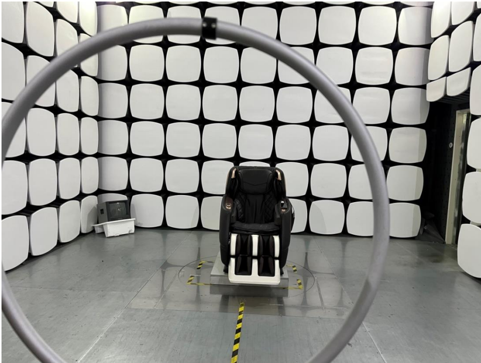
Below 30MHz Test setup
