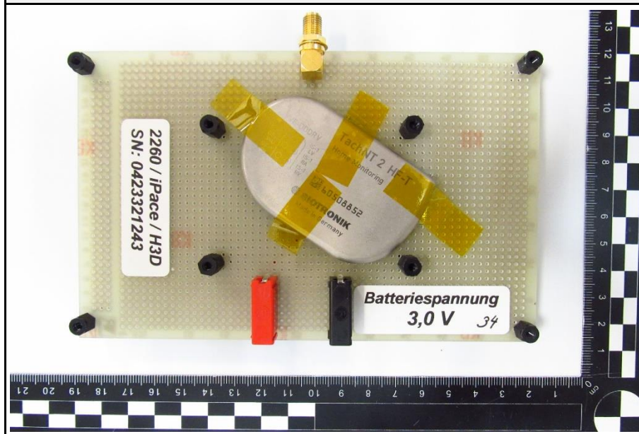
EUT Conducted
