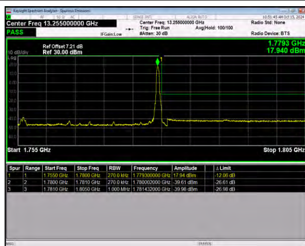
n66 SCS=15kHz DFT_256QAM BW=25MHz HighChannel=353500 RB=1@132
