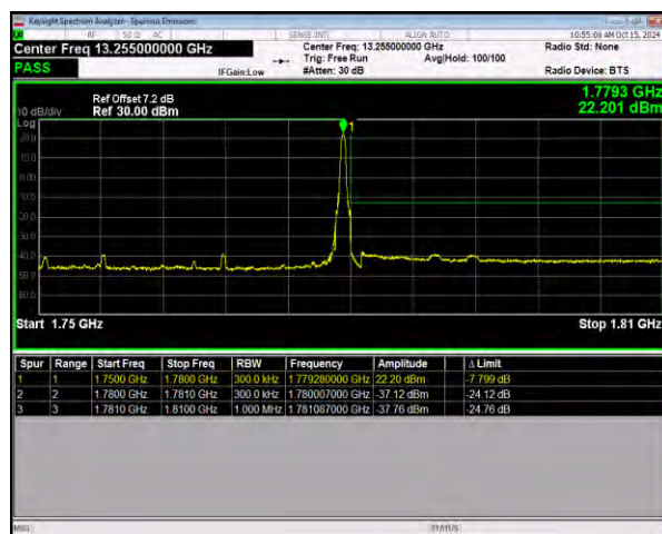
n66 SCS=15kHz DFT_BPSK BW=30MHz HighChannel=353000 RB=1@159
