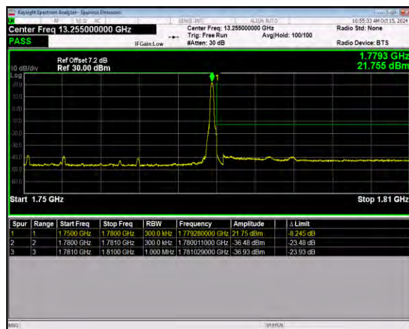
n66 SCS=15kHz DFT_QPSK BW=30MHz HighChannel=353000 RB=1@159
