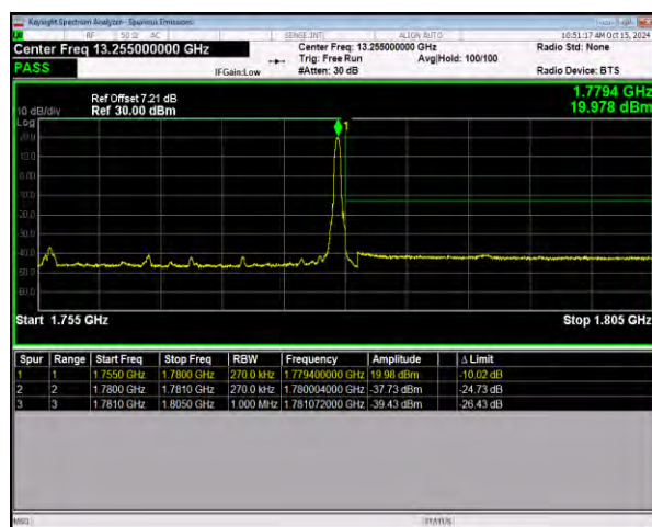
n66 SCS=15kHz DFT_64QAM BW=25MHz HighChannel=353500 RB=1@132
