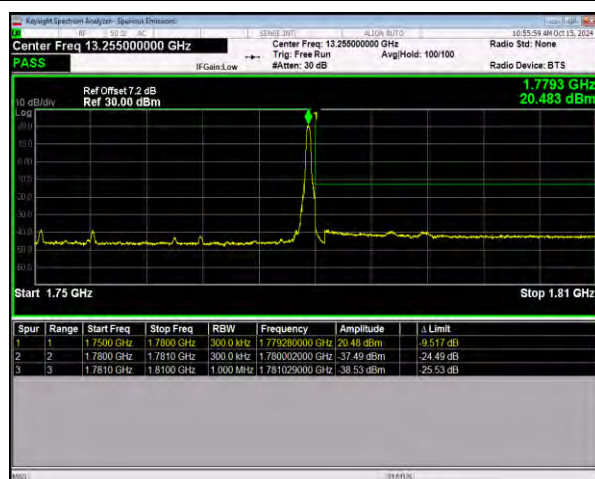
n66 SCS=15kHz DFT_16QAM BW=30MHz HighChannel=353000 RB=1@159
