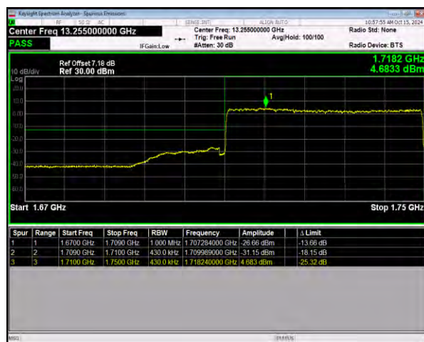
n66 SCS=15kHz DFT_BPSK BW=40MHz LowChannel=346000 RB=216@0
