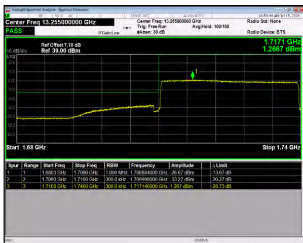
n66 SCS=15kHz CP_QPSK BW=30MHz LowChannel=345000 RB=160@0
