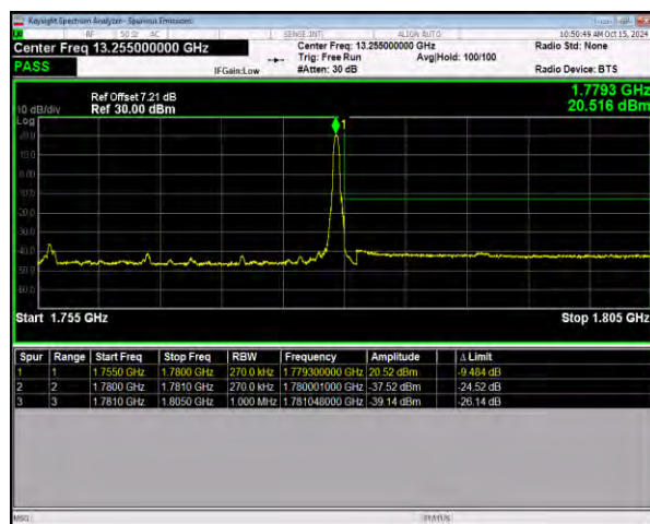
n66 SCS=15kHz DFT_16QAM BW=25MHz HighChannel=353500 RB=1@132
