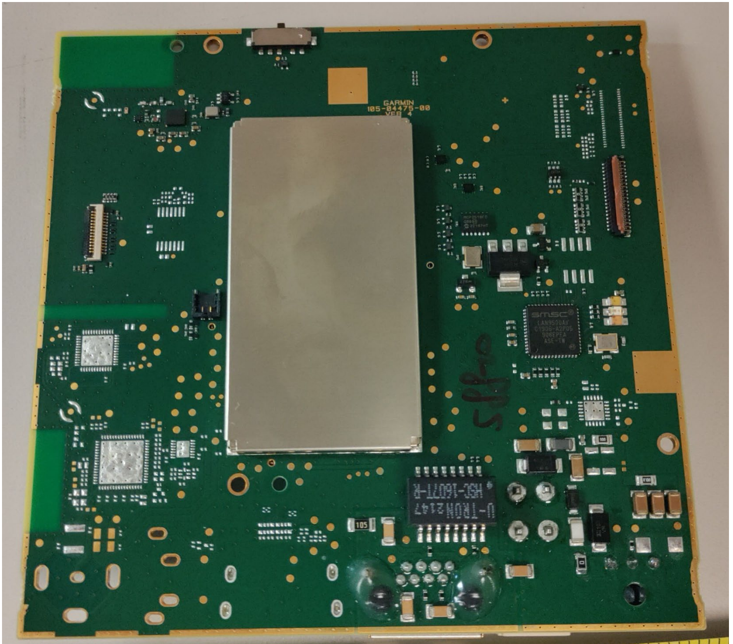
A04475 7" Digital Board – bottom side with cover
