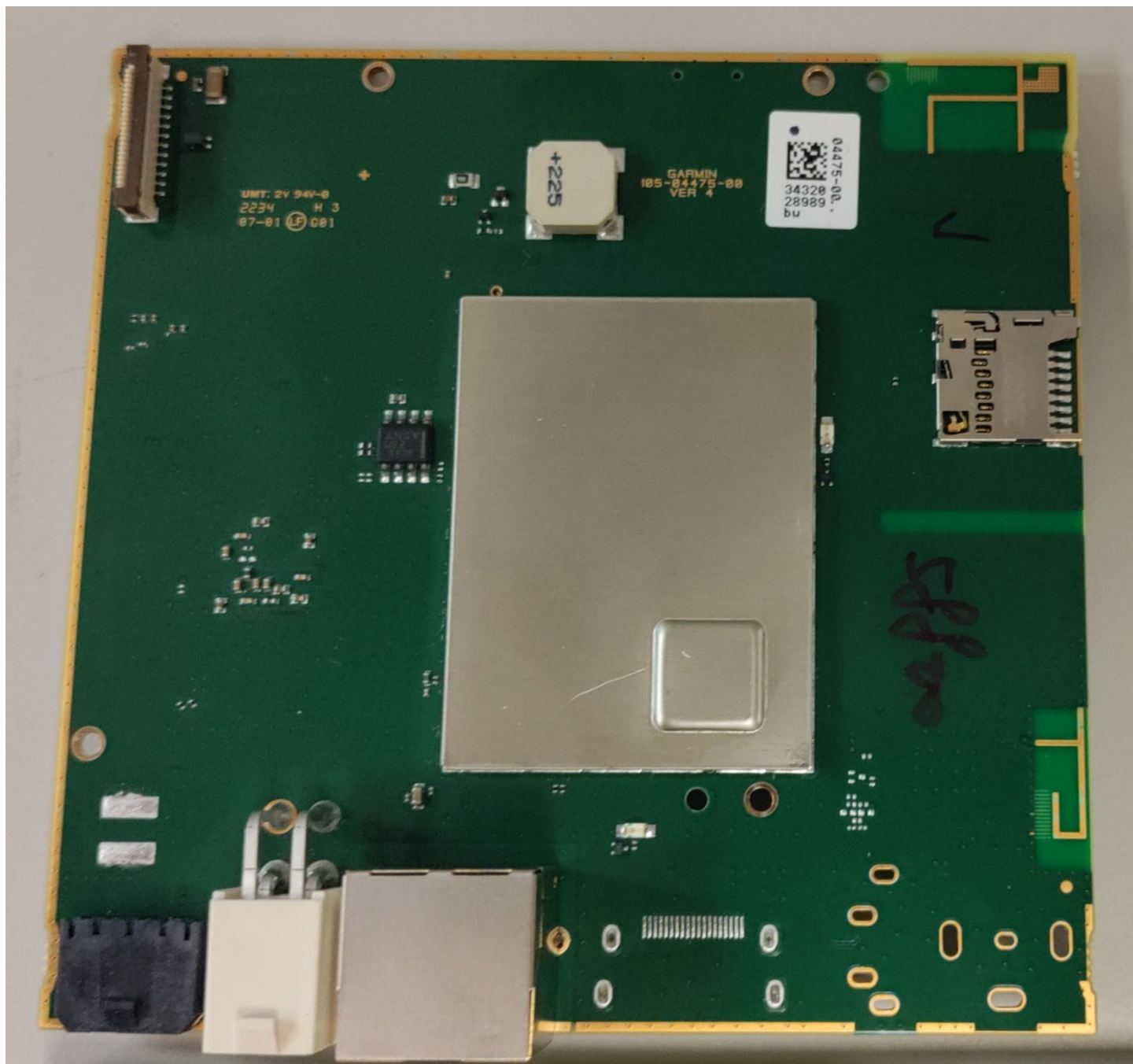
A04475 10" Digital Board – Top Side with cover
