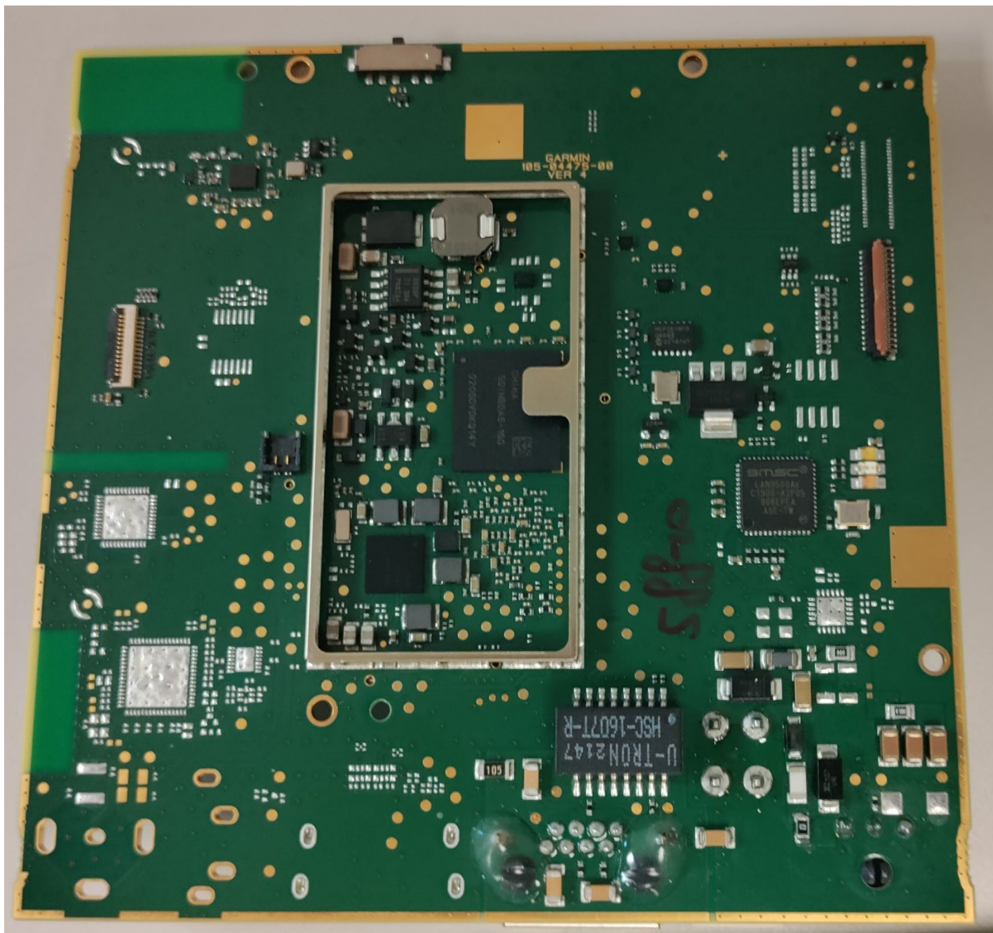
A04475 10" Digital Board – bottom side without cover
