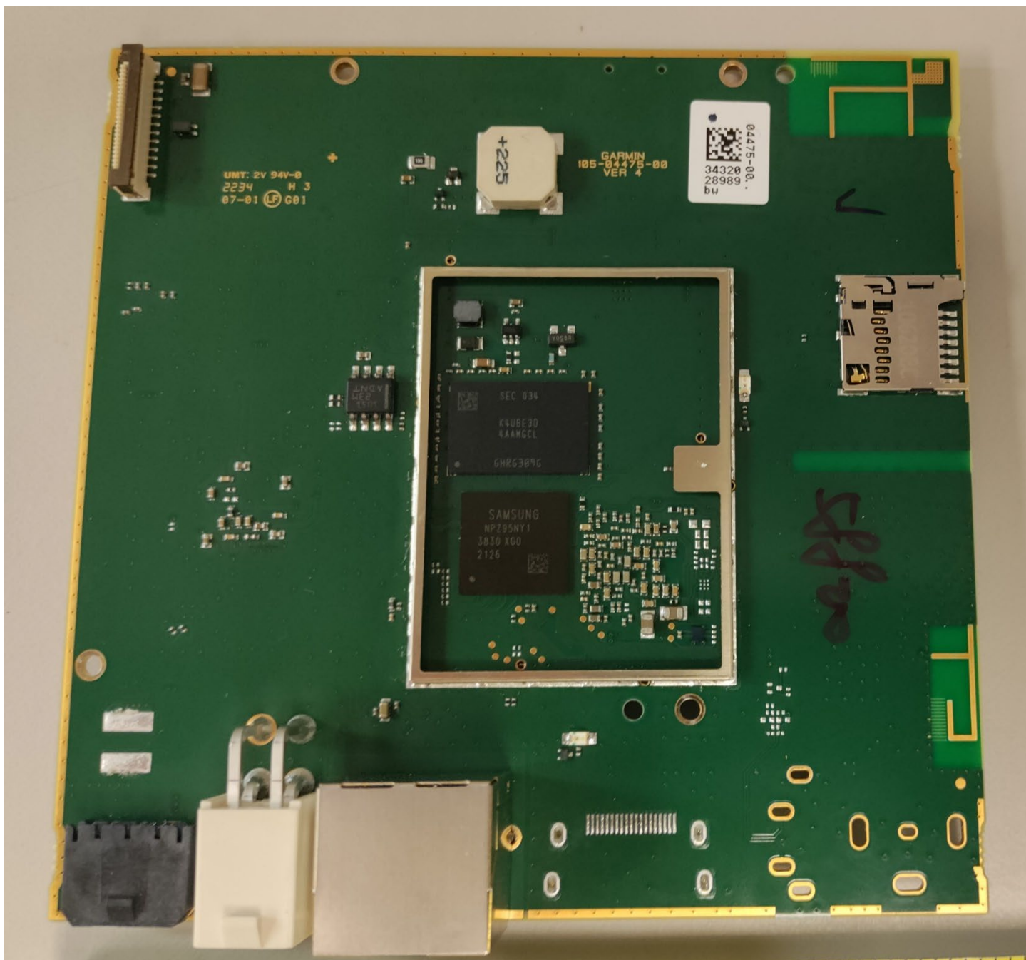
A04475 10" Digital Board – Top Side without cover
