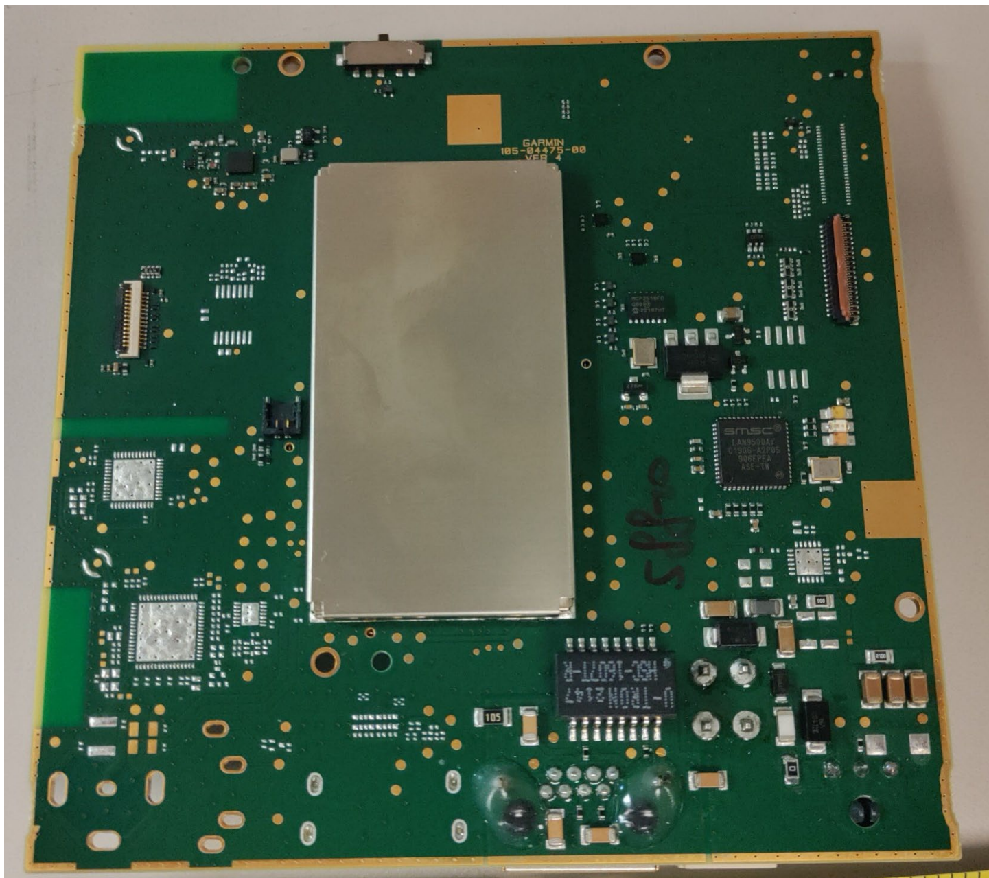
A04475 10" Digital Board – bottom side with cover
