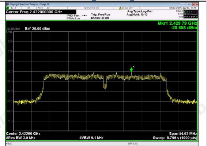
IEEE 802.11n_Channel 3_40MHz
