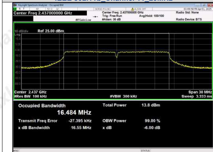
IEEE 802.11g Channel 6_20MHz
