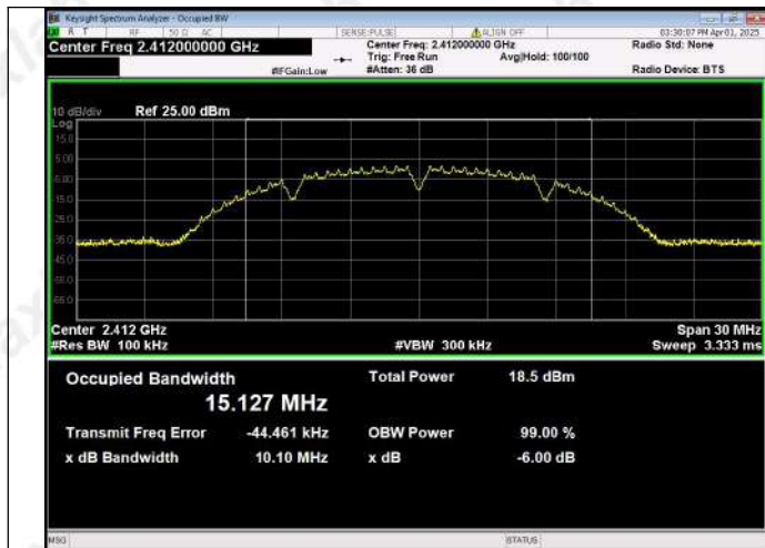
IEEE 802.11b Channel 1_20MHz
