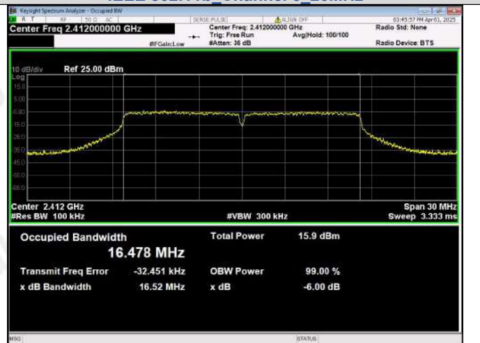
IEEE 802.11g Channel 1_20MHz
