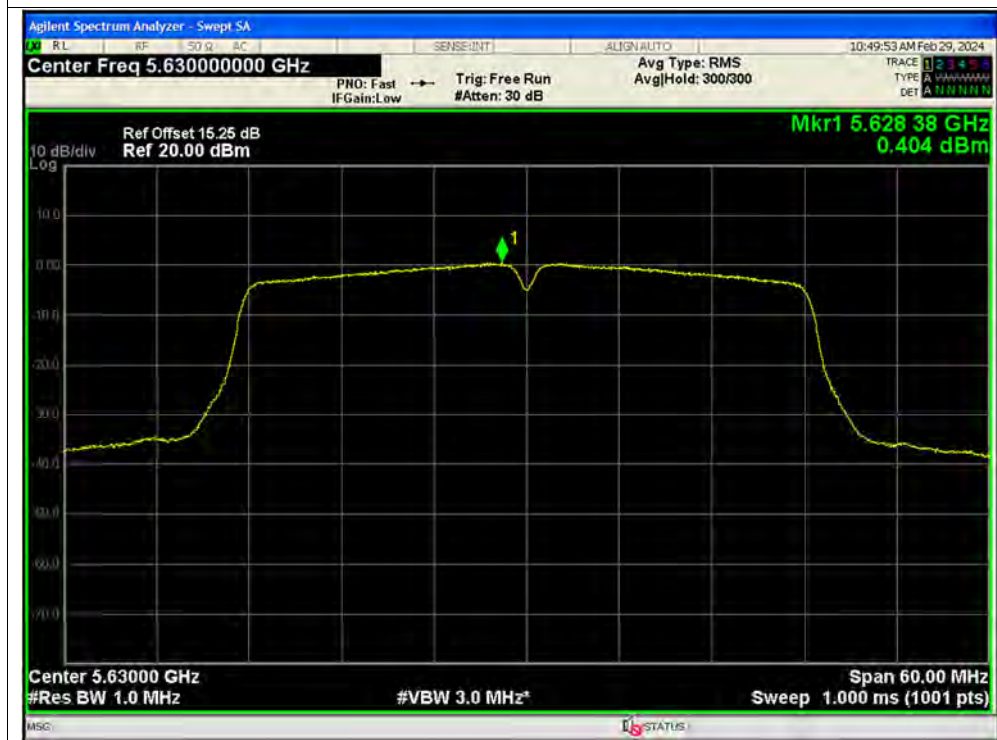
PSD NVNT n40 5630MHz Ant2 MIMO
