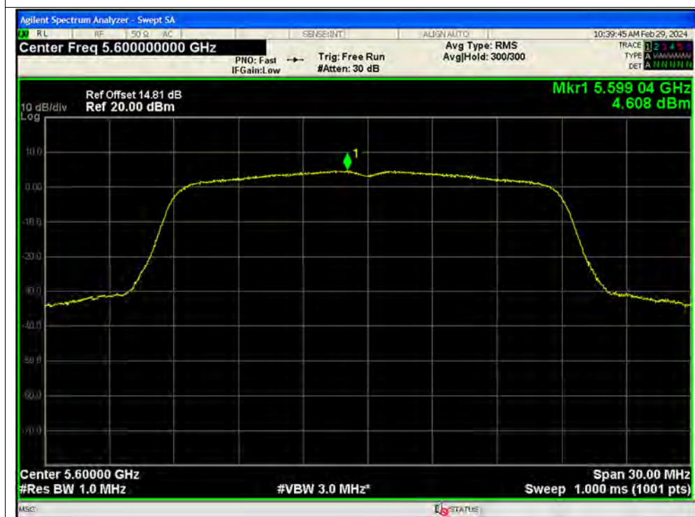
PSD NVNT n20 5600MHz Ant2 MIMO
