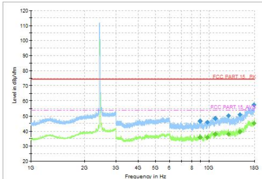
Fig.73 Radiated Spurious Emission (802.11ax-HE20, CH6, 1GHz-18GHz)
