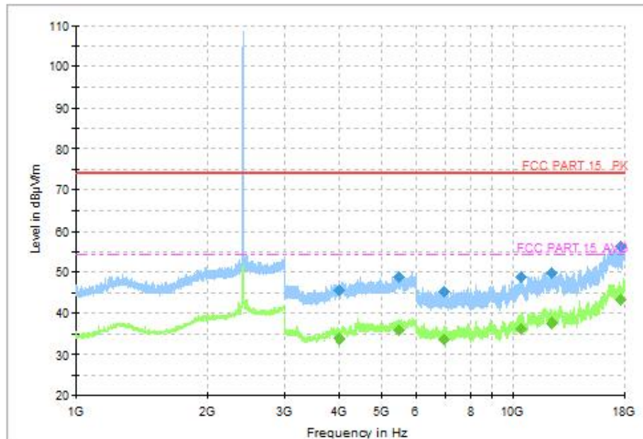
Fig.67 Radiated Spurious Emission (802.11n-HT20, CH1, 1GHz-18GHz)
