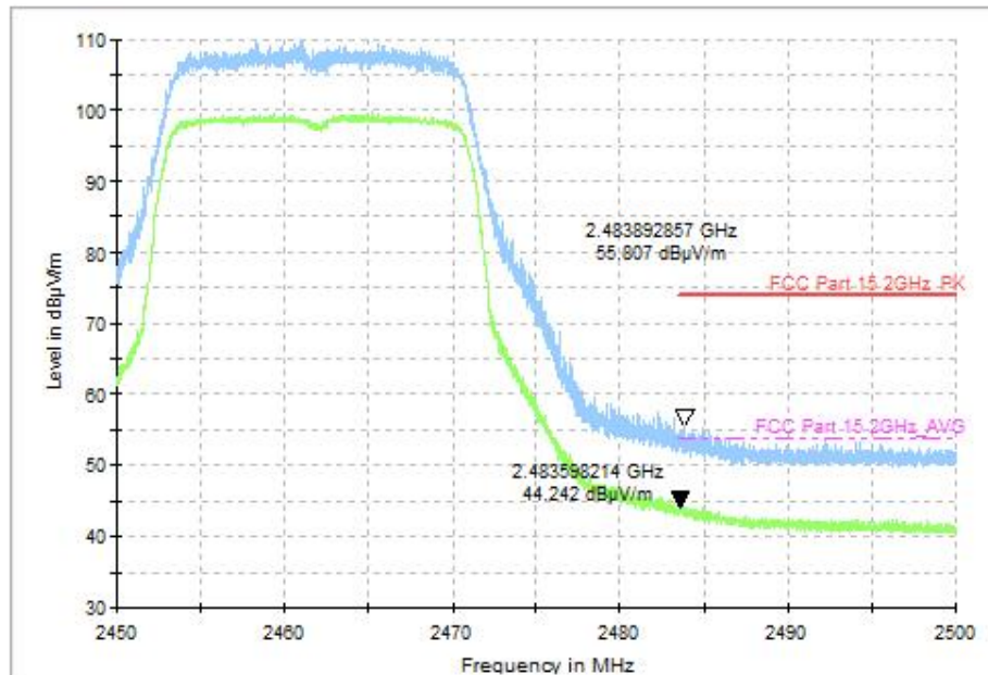
Fig.71 Radiated Spurious Emission (802.11n-HT20, CH11, 2.45GHz~2.50GHz)
