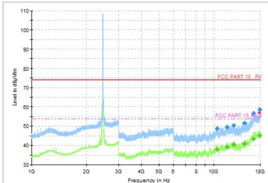
Fig.59 Radiated Spurious Emission (802.11b, CH11, 1GHz-18GHz)
