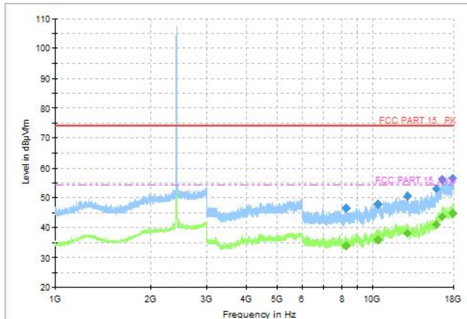
Fig.89 Radiated Spurious Emission (802.11ax-HE20, CH1, 1GHz-18GHz),MIMO
