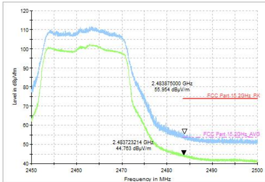
Fig.88 Radiated Spurious Emission (802.11n-HT20, CH11, 2.45GHz~2.50GHz),MIMO
