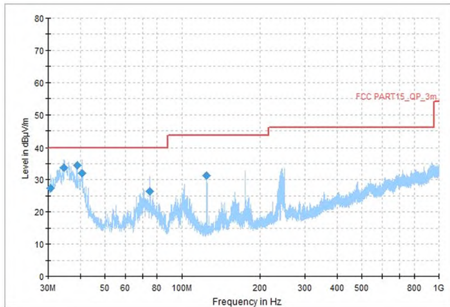
Fig.82 Radiated Spurious Emission (All channel, 30MHz~1GHz)
