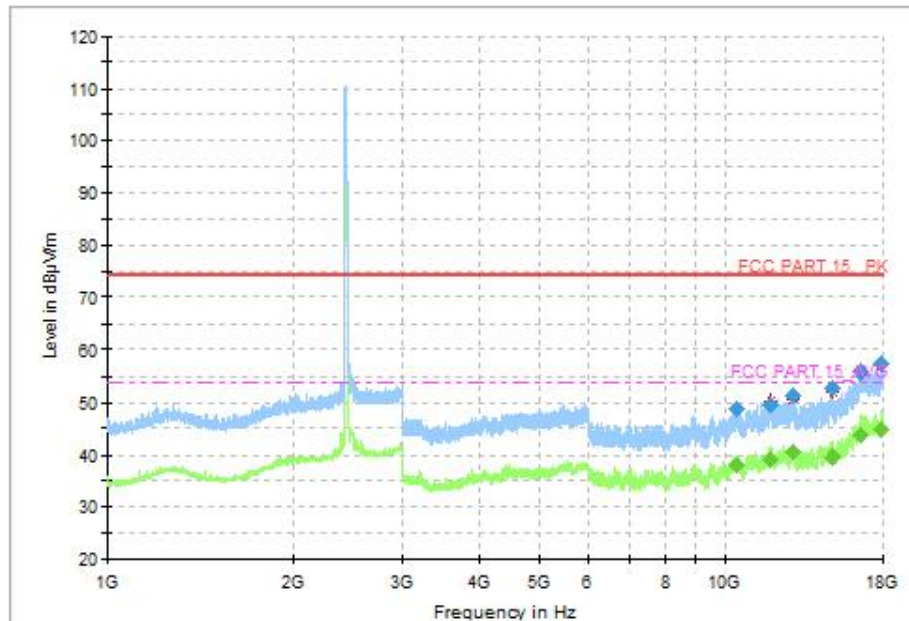
Fig.63 Radiated Spurious Emission (802.11g, CH6, 1GHz-18GHz)
