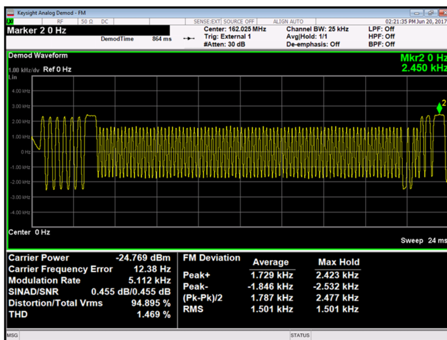
Figure 22 - 162.025 MHz - 01010101
