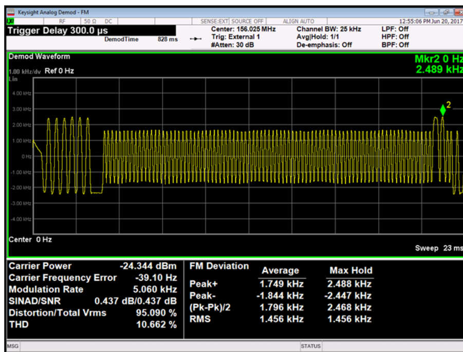
Figure 19 - 156.025 MHz - 01010101
