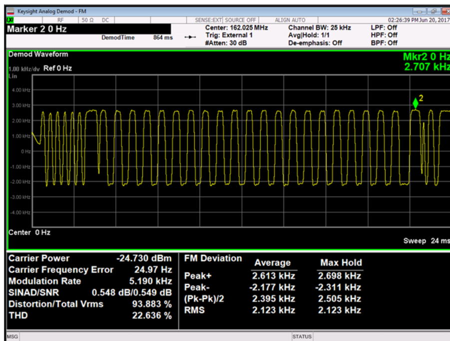
Figure 23- 162.025 MHz - 00001111
