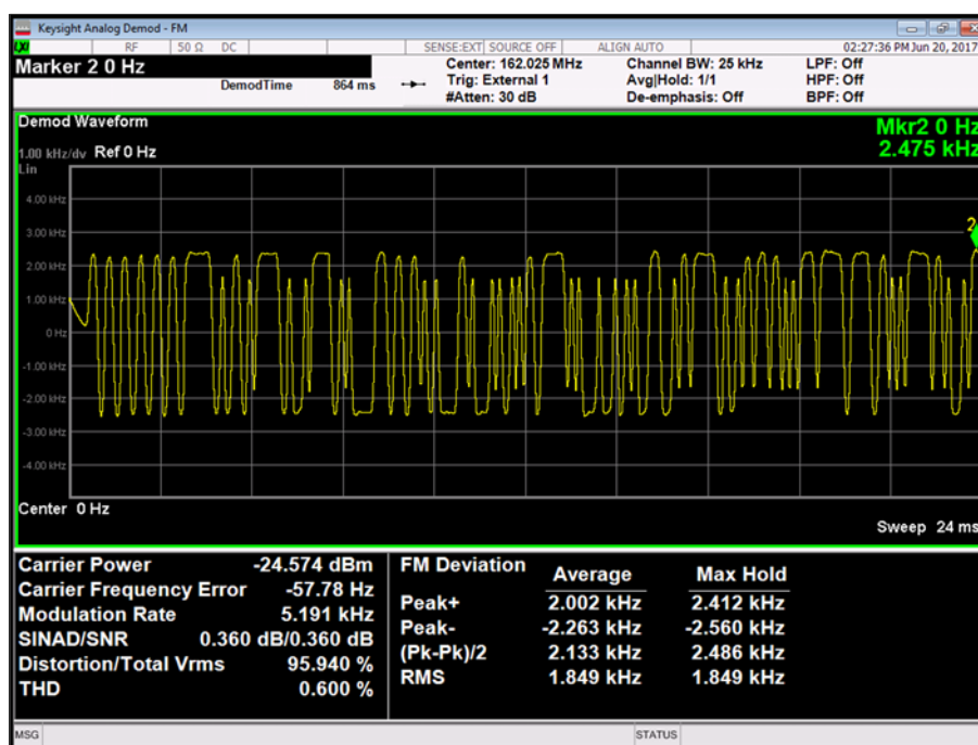
Figure 24- 162.025 MHz - PRBS
