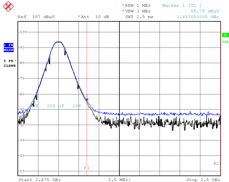
Radiated Restricted Band Edges plot –Peak Result (GFSK, Ch.78, X-V)
