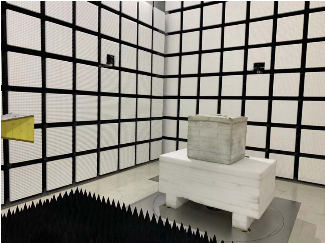
Radiated Emission Above 1GHz View- VS341-915M
