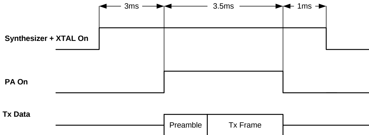
Figure 4: Transmit Timing
