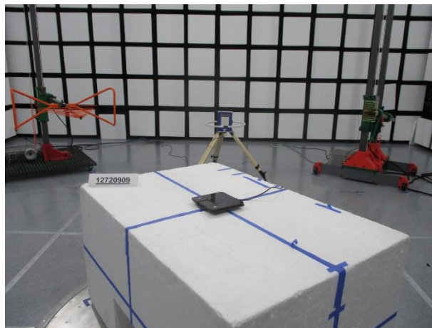
GROUND-PARALLEL
