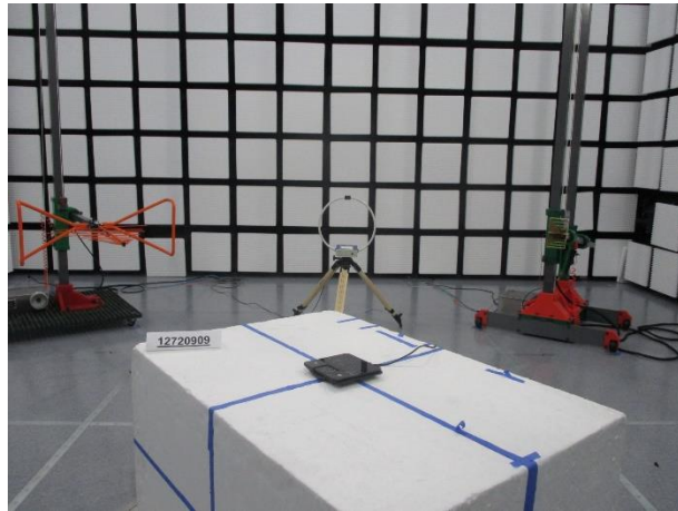
PARALLEL
