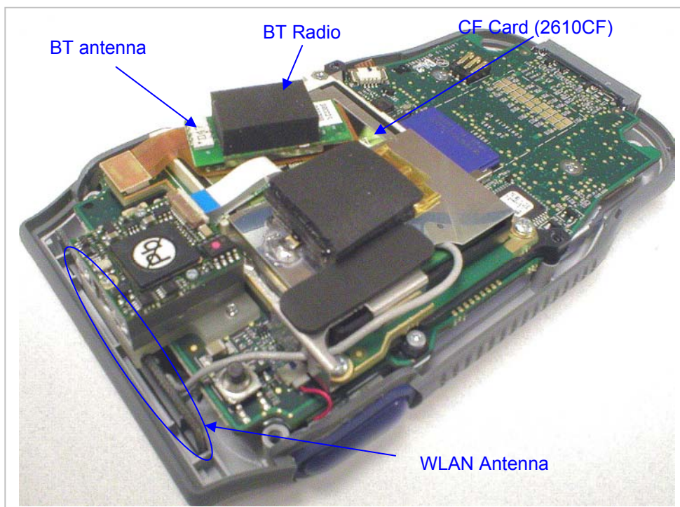
Radio module &amp; Antenna locations
