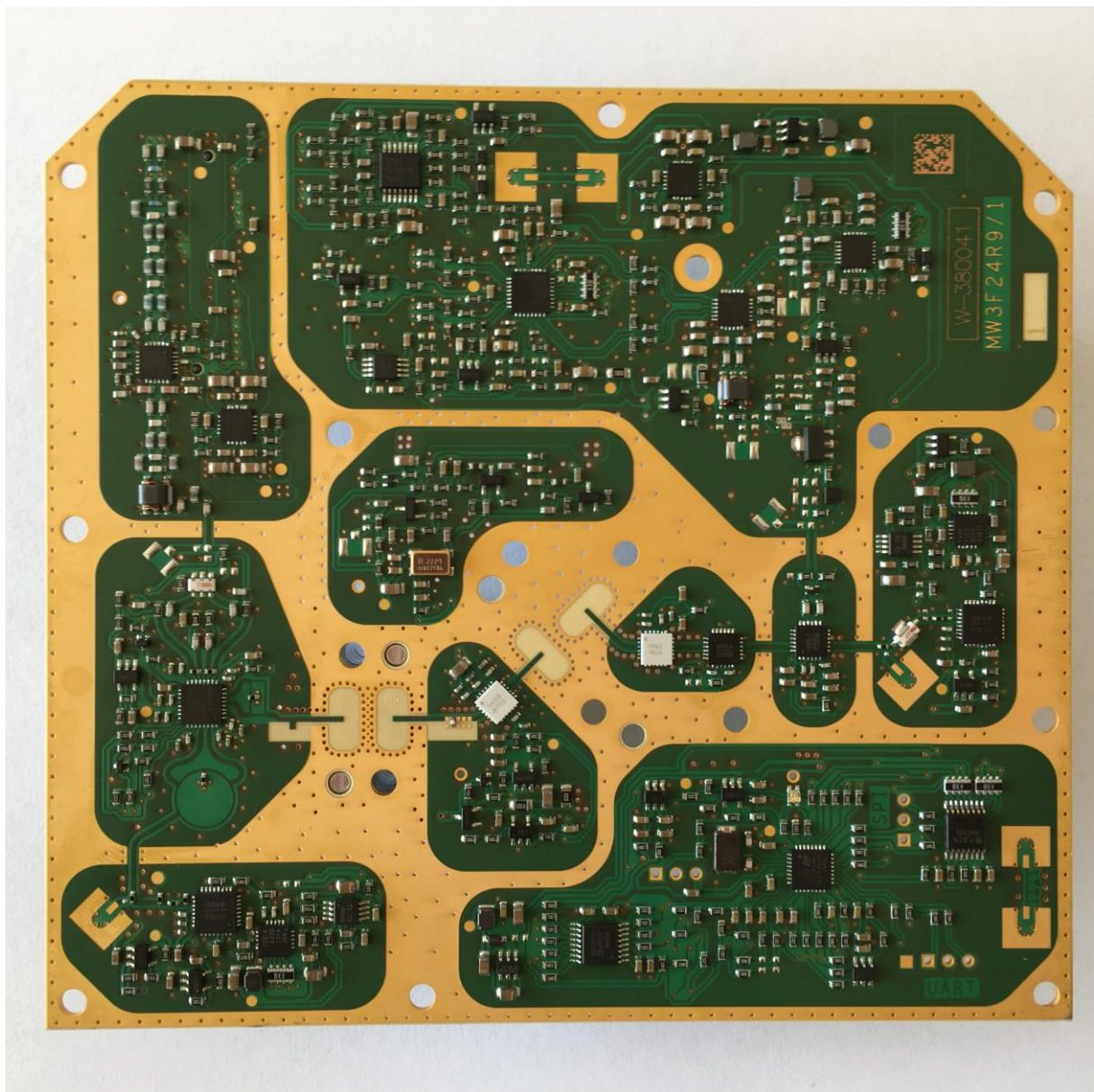
RF Board, Top
