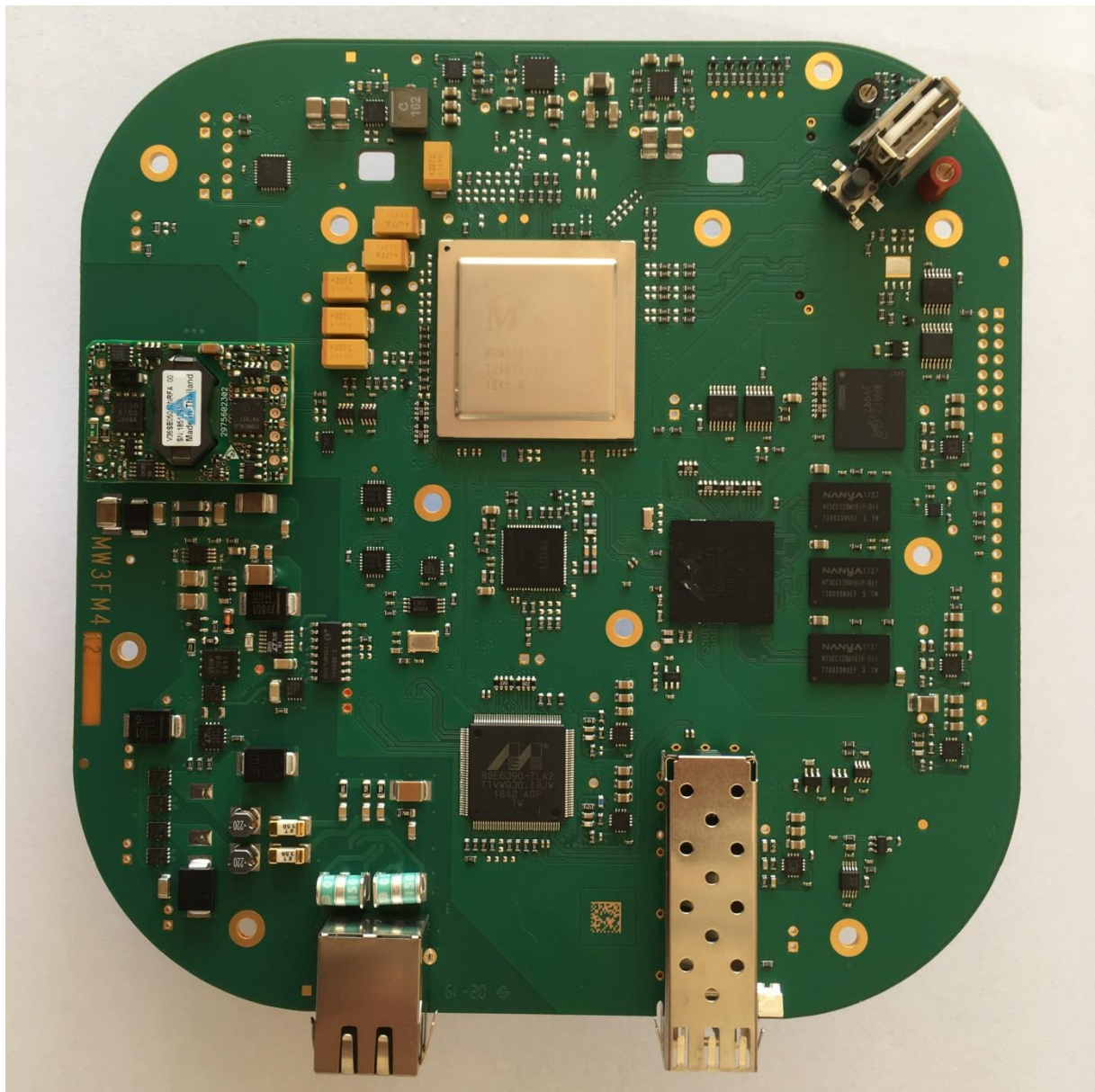
Logic Board, Top
