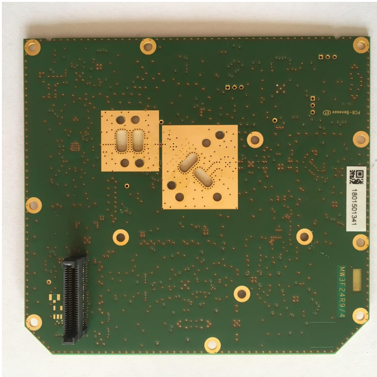
RF Board, Bottom unscrewed
