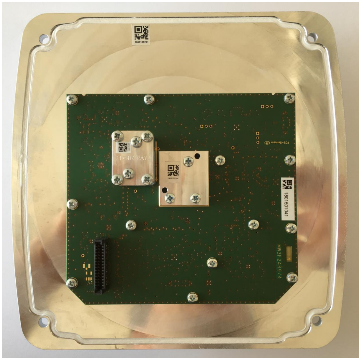
RF Board Installed To Wave Guide Assembly
