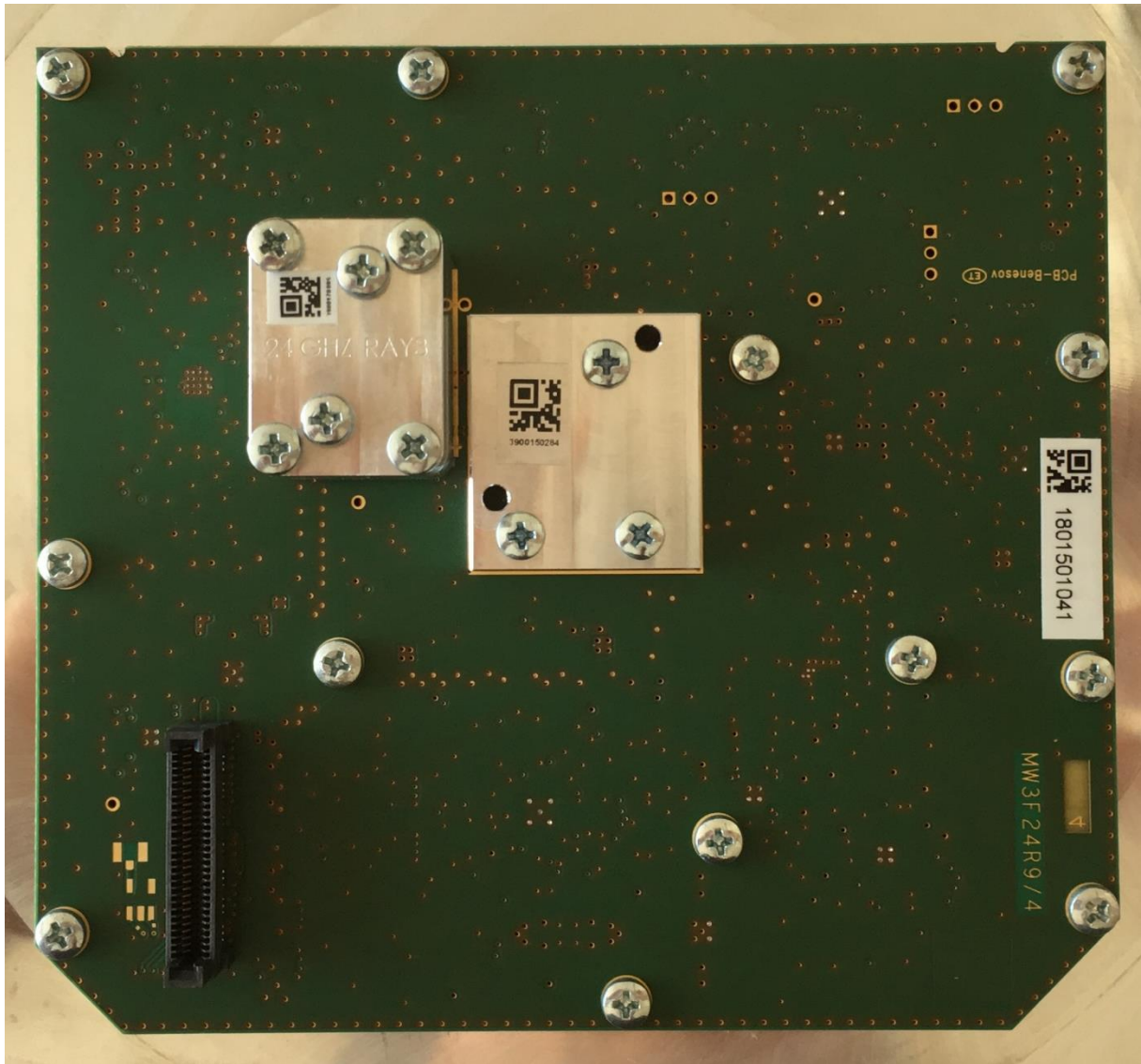
RF Board, Bottom
