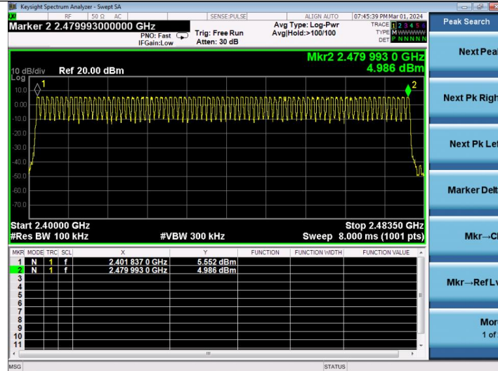
GFSK Modulation
