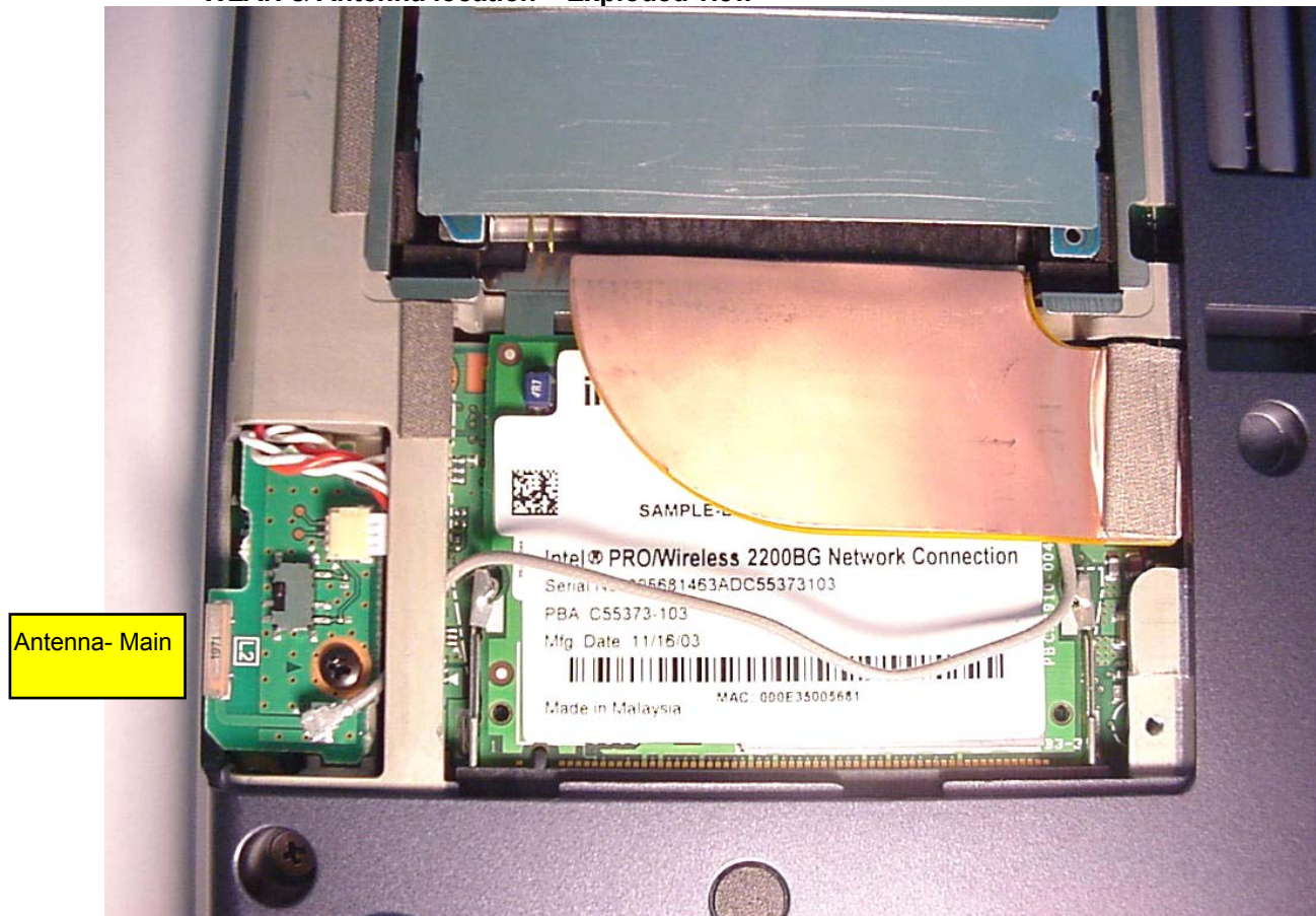
WLAN & Antenna location – Exploded view
