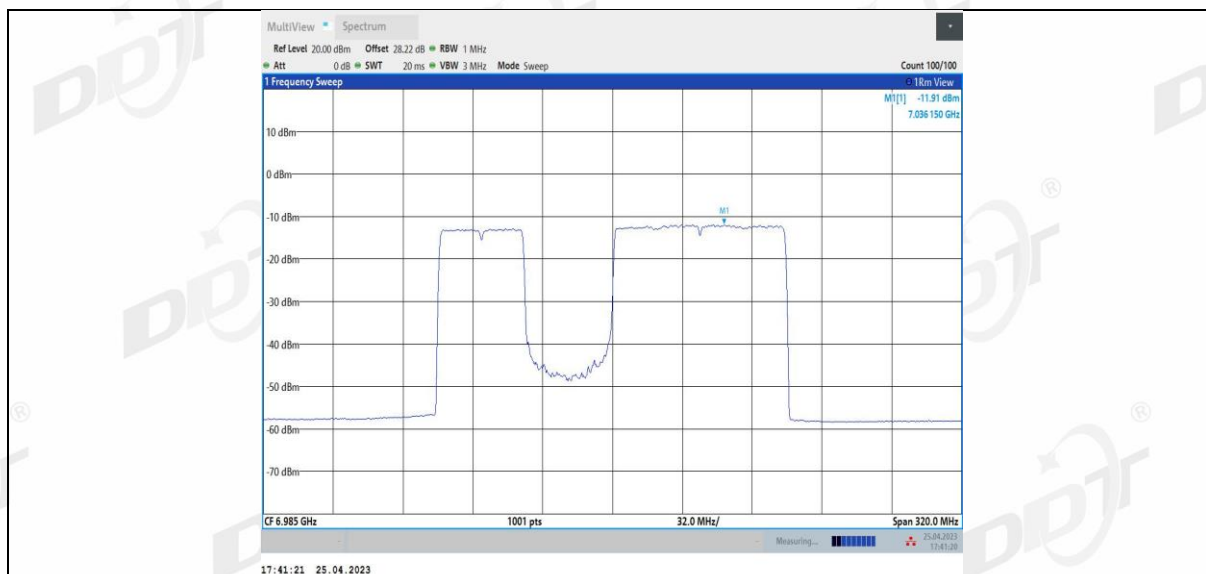
11BE160MIMO Ant2_6985_996+484_3
