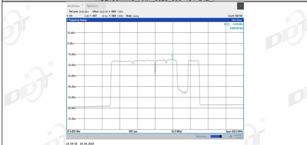
11BE160MIMO Ant4 6825_996+484+242_8
