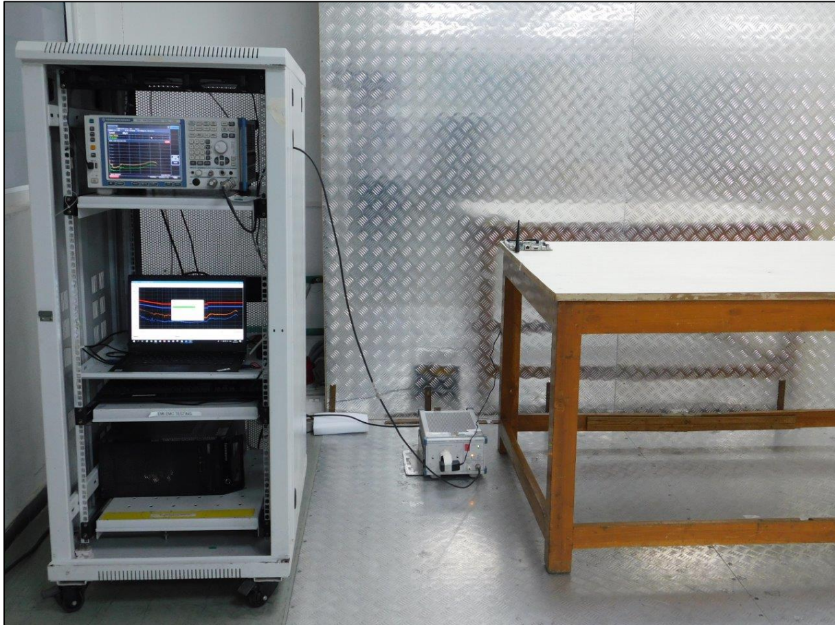
Conducted AC Power Lines test setup photo
