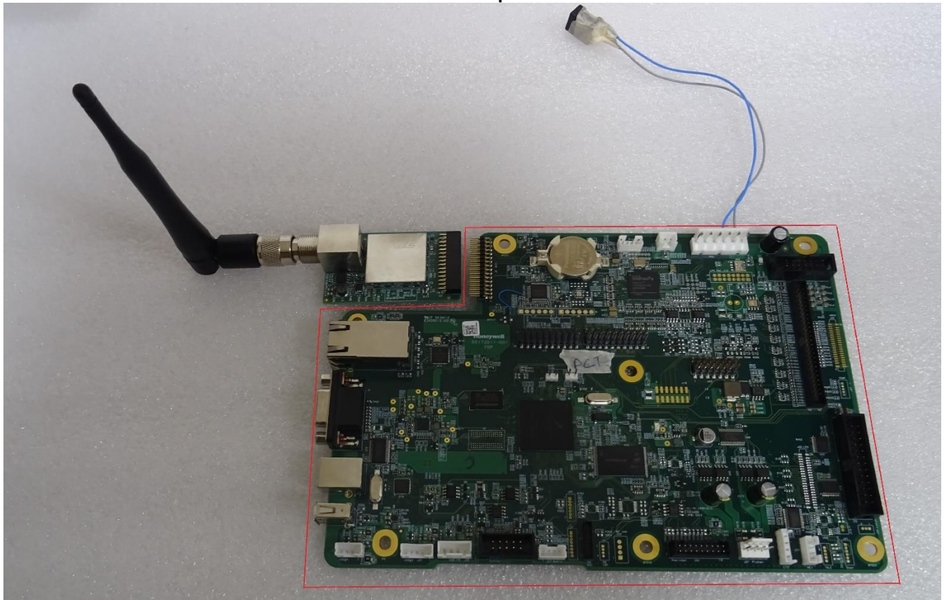
Carrier board used for configuration
