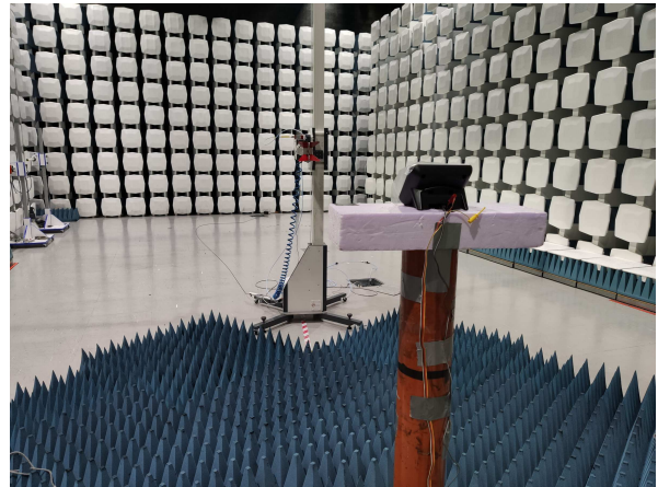
Radiated Emissions 1 – 18 GHz
