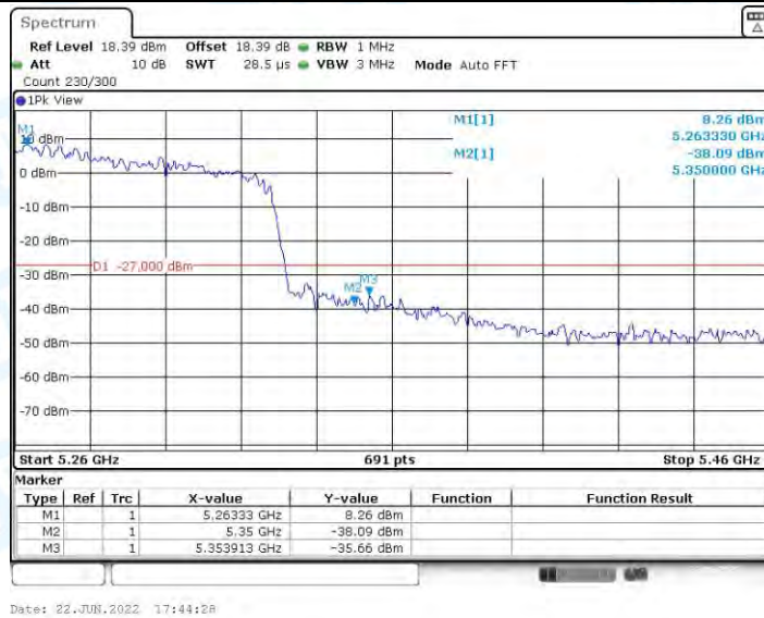
11AC80MIMO_Ant2_High_5290
