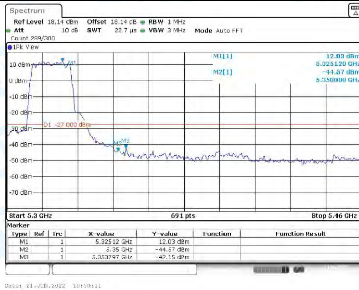
11N20MIMO_Ant1_High_5320
