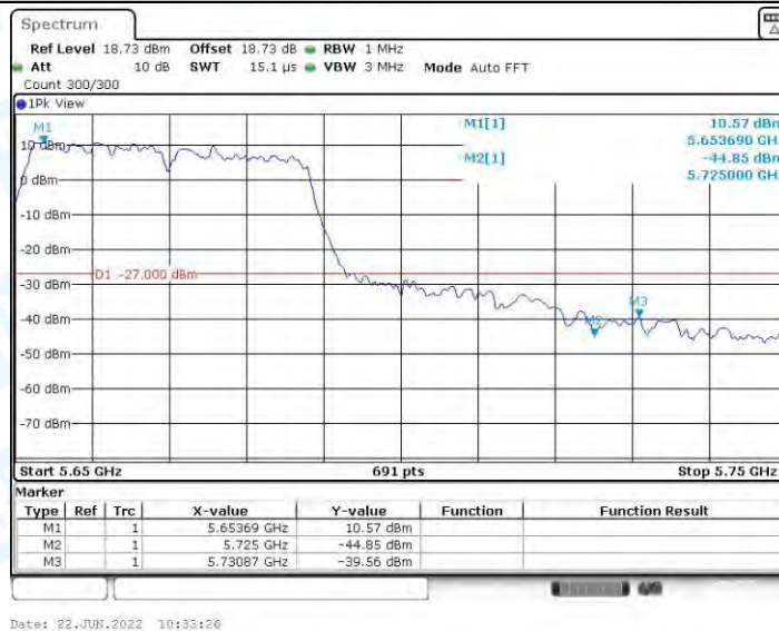
11N40MIMO_Ant2_High_5670
