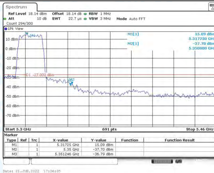
11A_Ant1_High_5320
