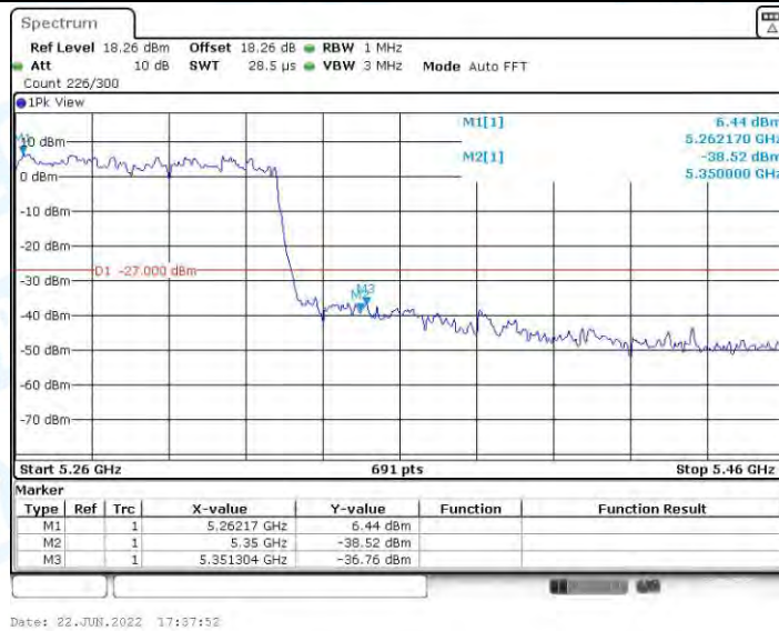
11AC80MIMO_Ant1_High_5290
