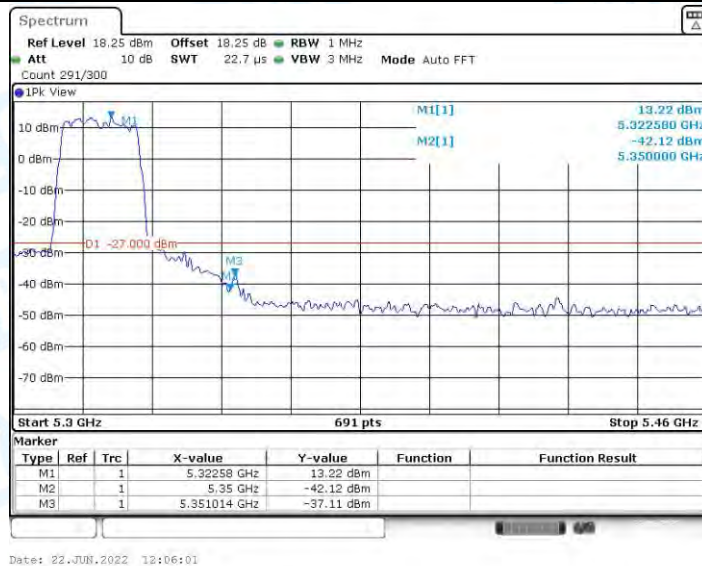
11AC20MIMO_Ant2_High_5320
