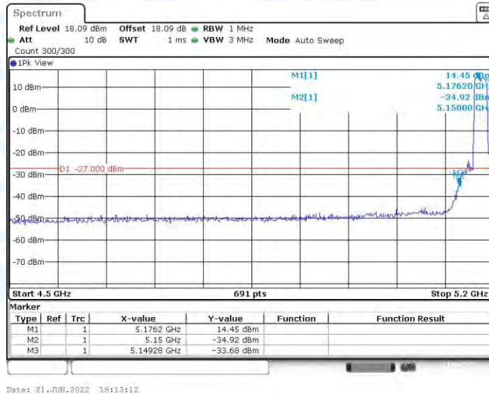
11A_Ant2_Low_5180
