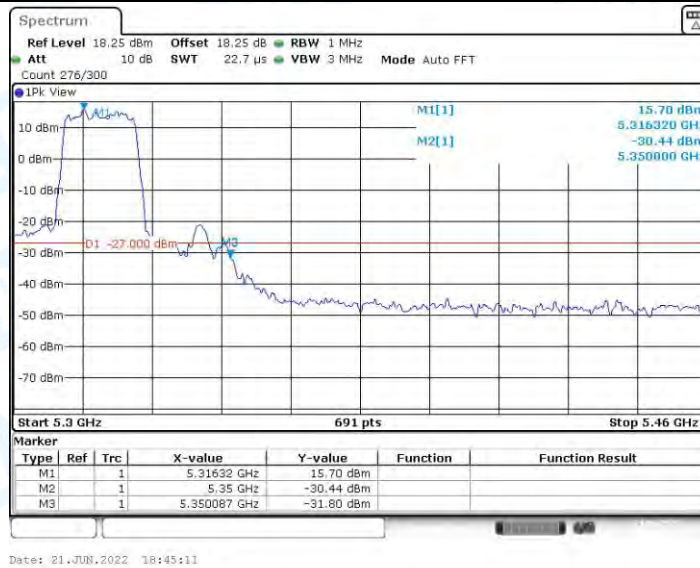
11A_Ant2_High_5320
