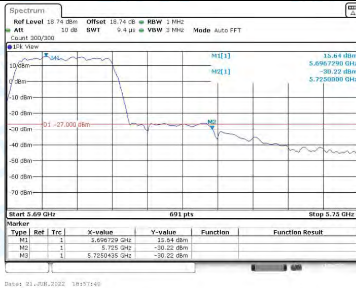
11A_Ant2_High_5700
