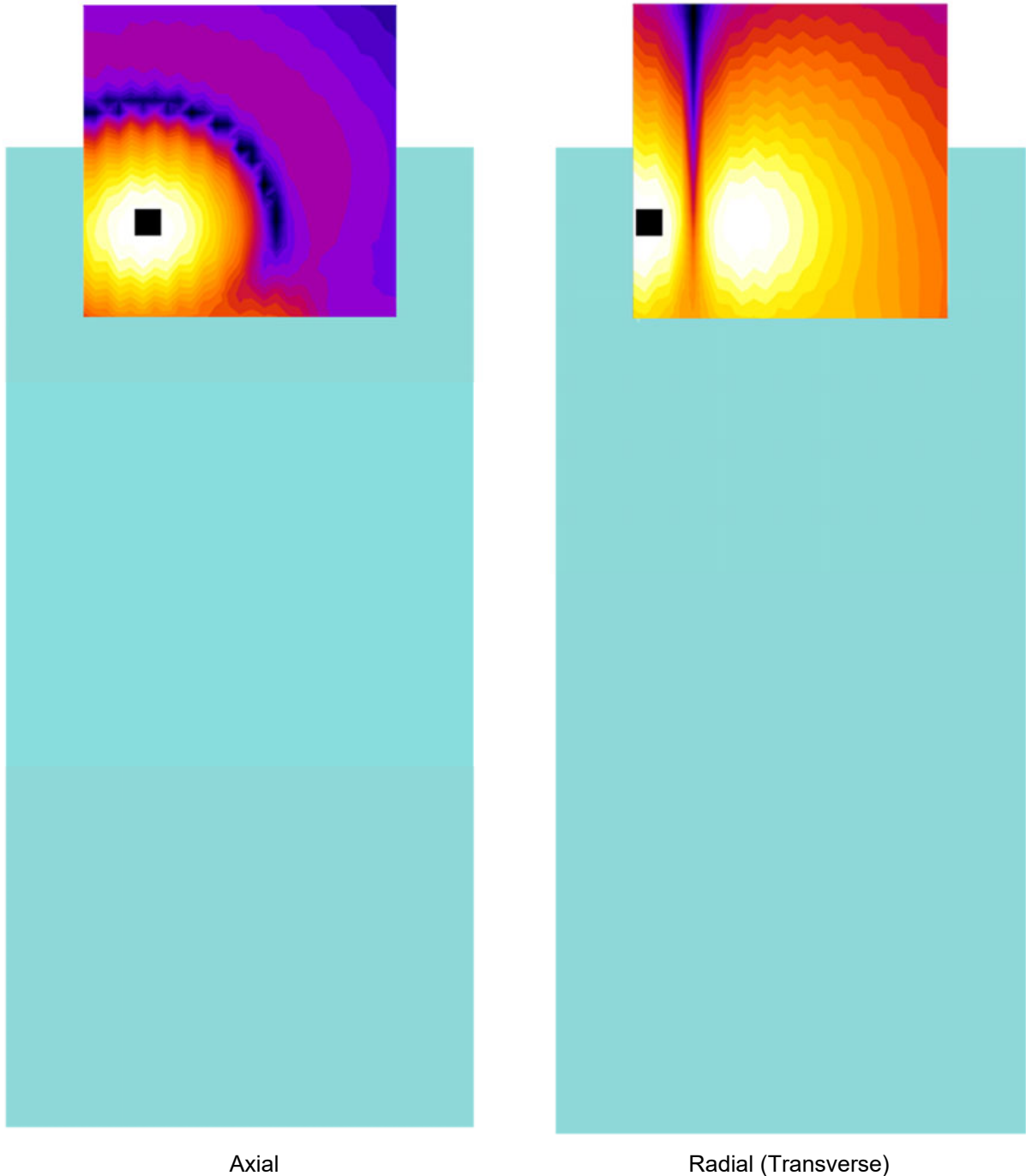
Figure 10-1 T-Coil Scan Overlay Magnetic Field Distributions
