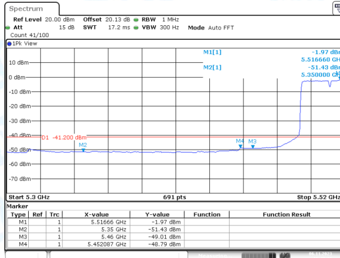
11AC40SISO_Ant1_Low_5510_Peak
