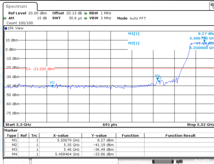
11AC40SISO_Ant1_Low_5510_Peak
