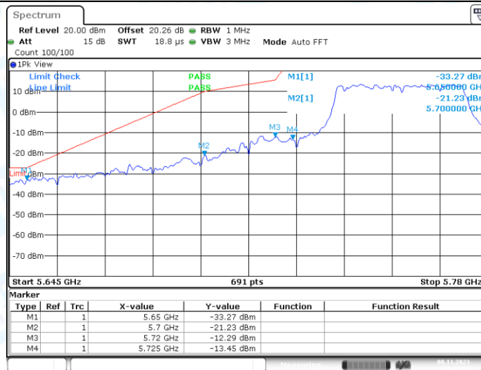
11AC40SISO_Ant1_Low_5755_Peak
