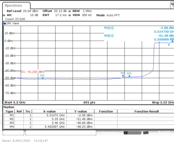
11N40SISO_Ant1_Low_5510_Peak
