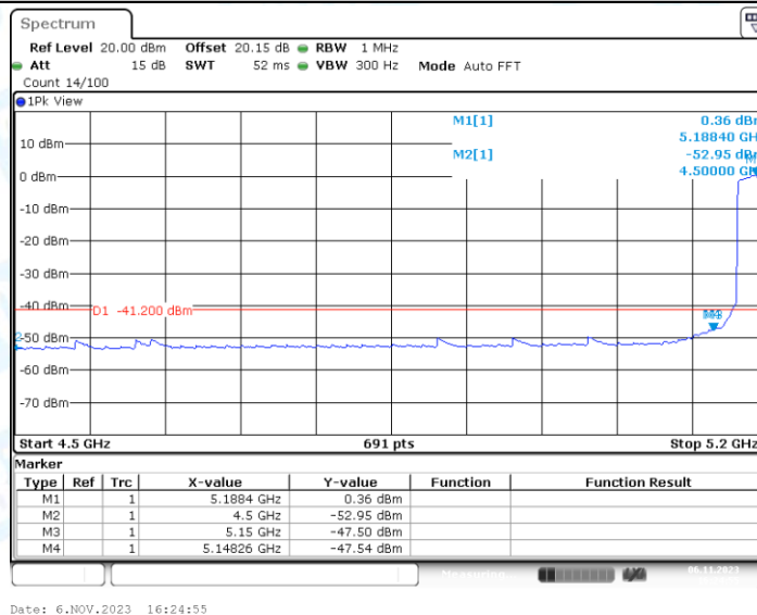
11AC40SISO_Ant1_Low_5190_Peak
