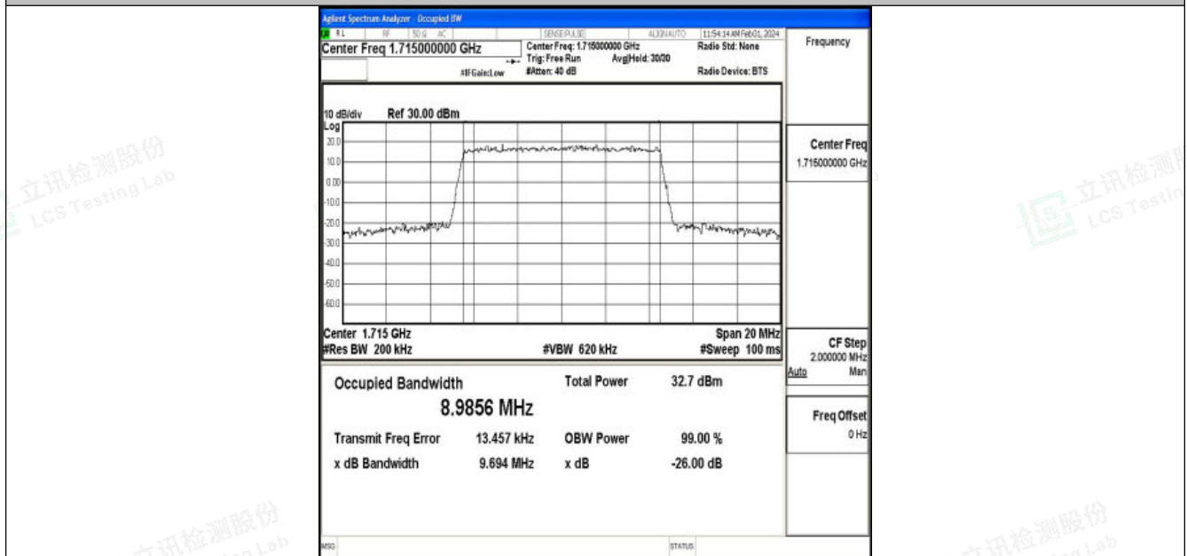
Band4-10MHz-16QAM-20000-50RB#0-PASS
