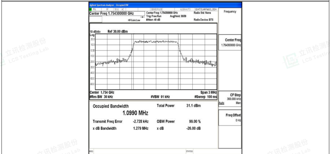
Band4-1.4MHz-16QAM-20393-6RB#0-PASS
