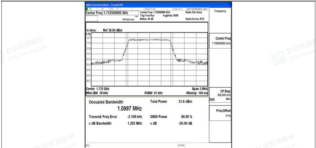
Band4-1.4MHz-16QAM-20175-6RB#0-PASS
