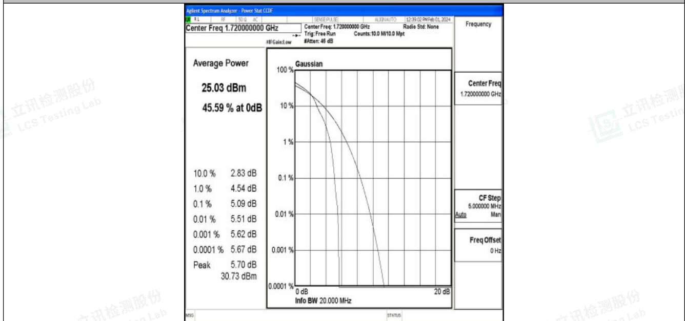
Band4-20MHz-16QAM-20050-1RB#0-PASS
