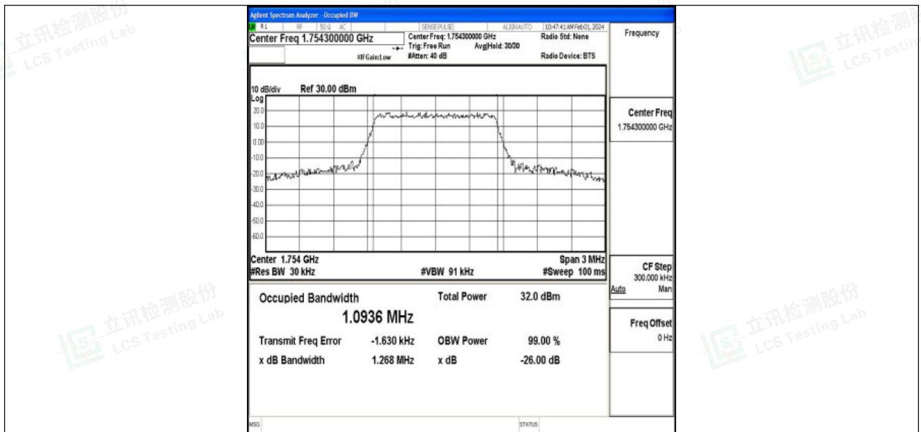
Band4-1.4MHz-QPSK-20393-6RB#0-PASS
