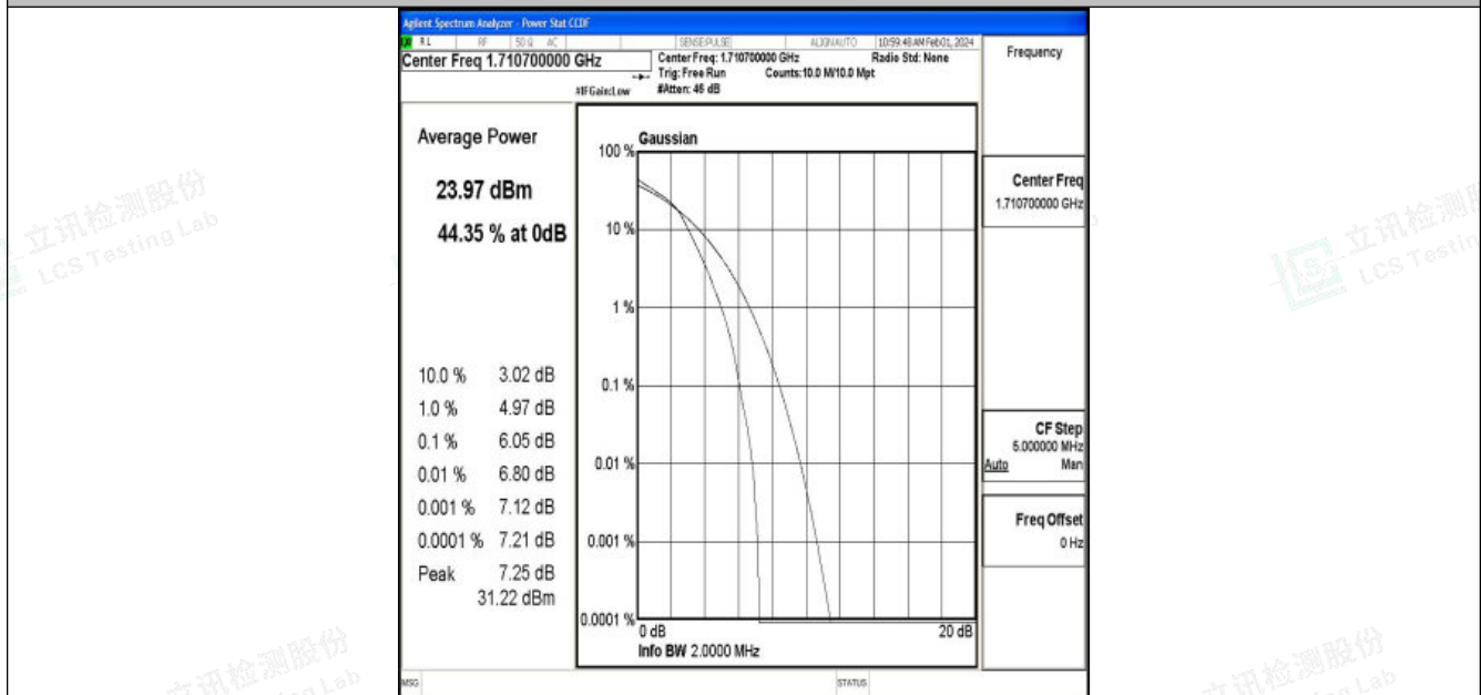
Band4-1.4MHz-16QAM-19957-6RB#0-PASS
