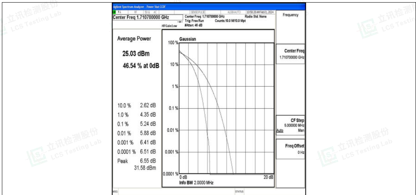
Band4-1.4MHz-QPSK-19957-6RB#0-PASS
