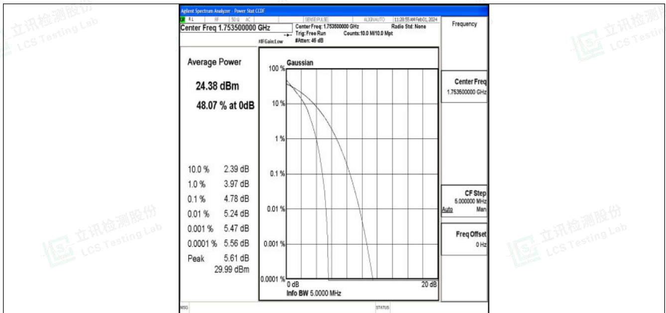
Band4-3MHz-QPSK-20385-15RB#0-PASS
