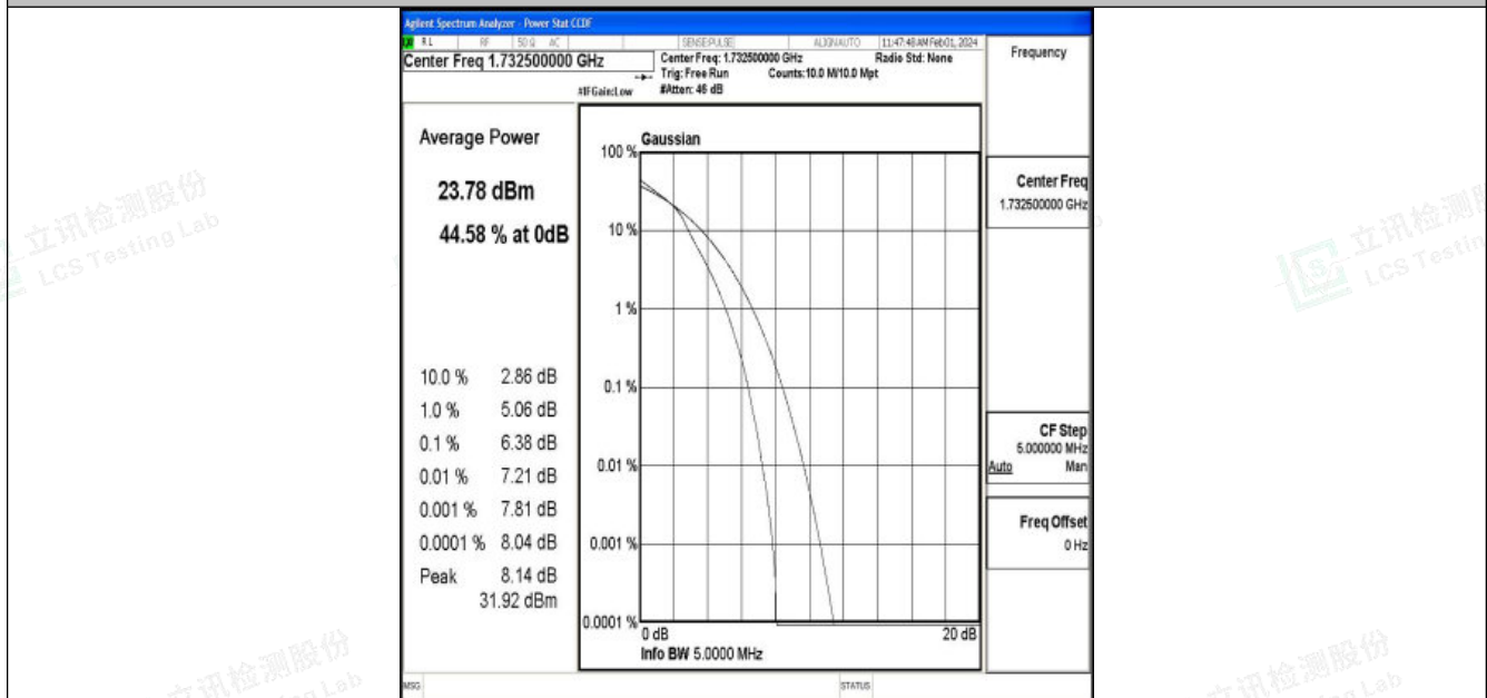
Band4-5MHz-16QAM-20175-25RB#0-PASS
