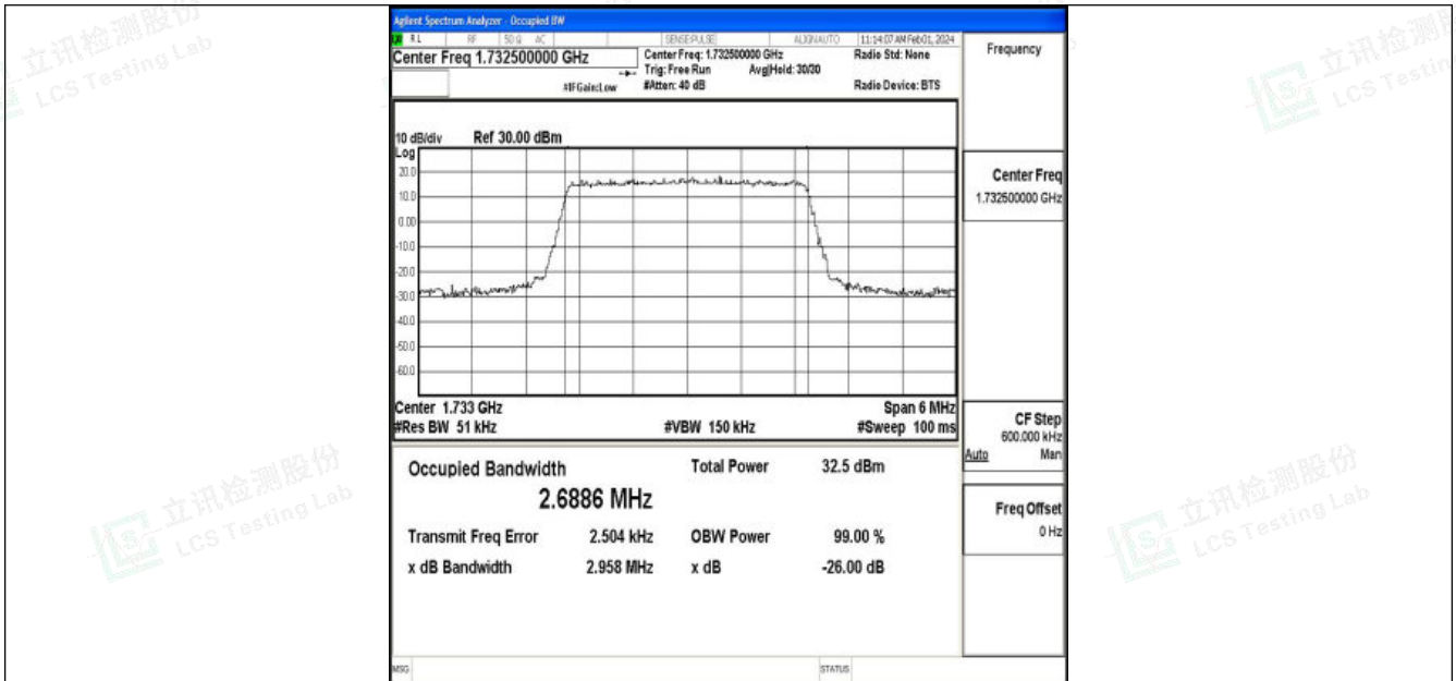
Band4-3MHz-QPSK-20175-15RB#0-PASS
