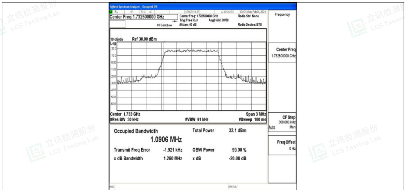
Band4-1.4MHz-QPSK-20175-6RB#0-PASS
