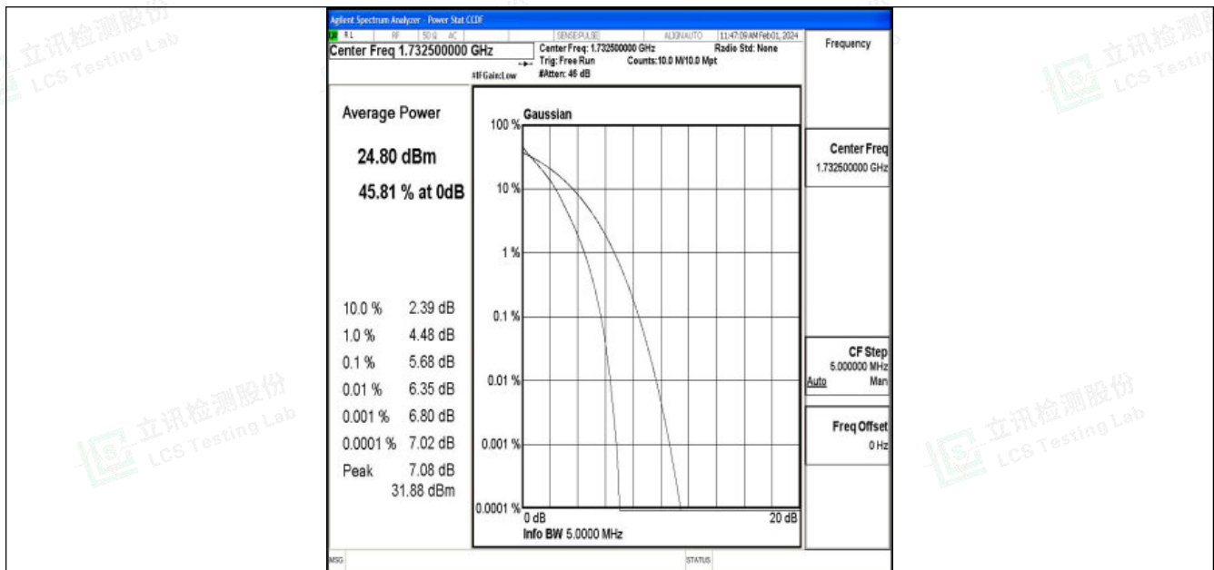
Band4-5MHz-QPSK-20175-25RB#0-PASS
