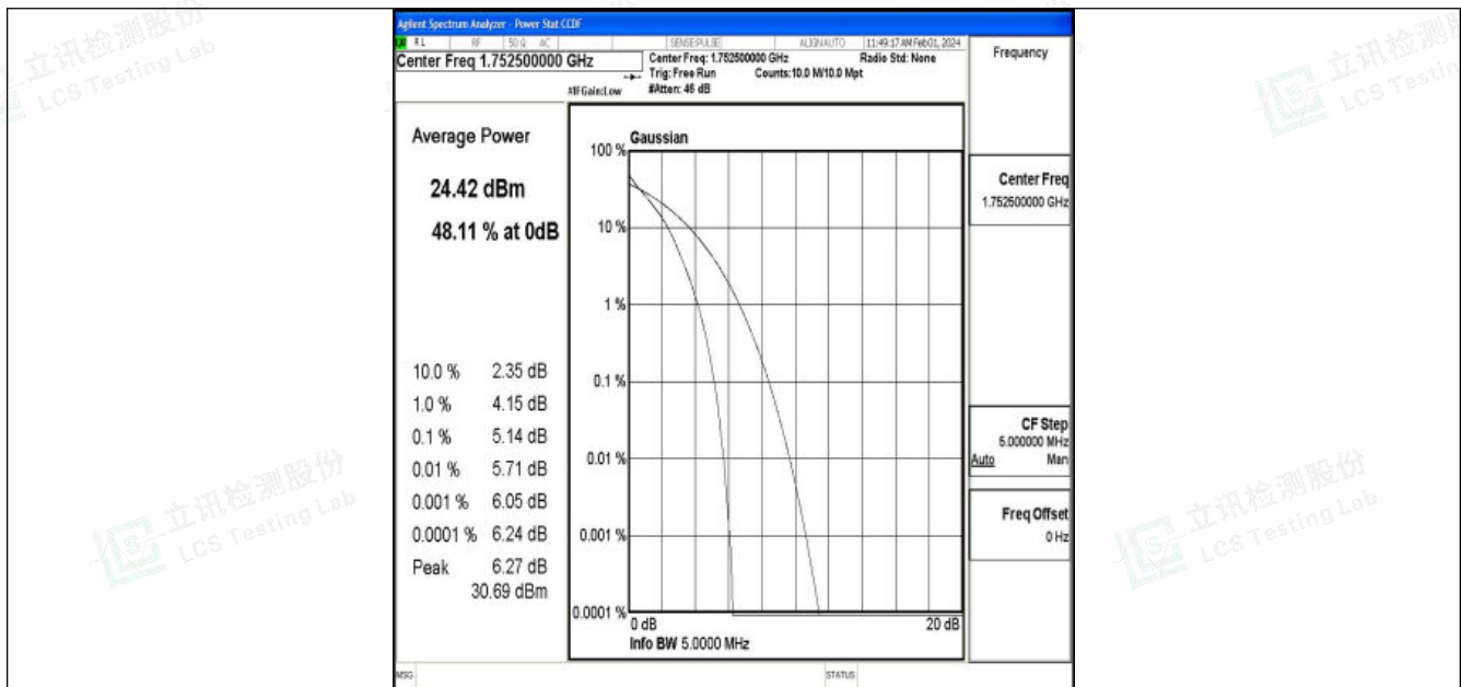
Band4-5MHz-QPSK-20375-25RB#0-PASS
