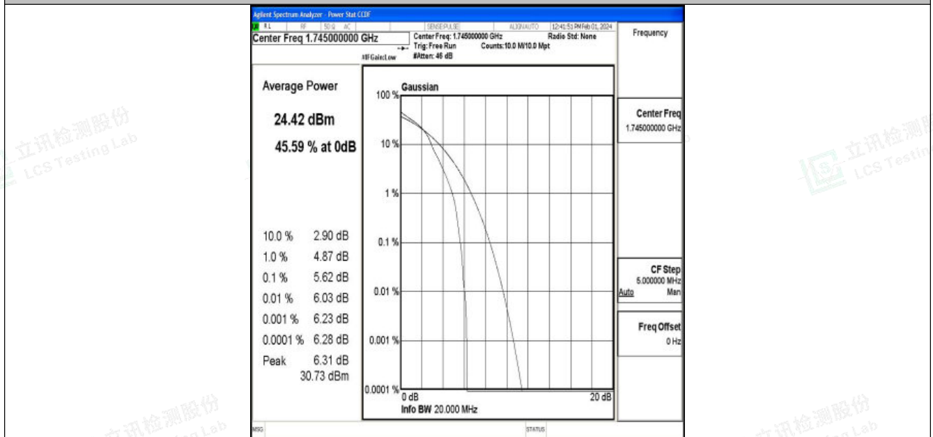
Band4-20MHz-16QAM-20300-1RB#0-PASS
