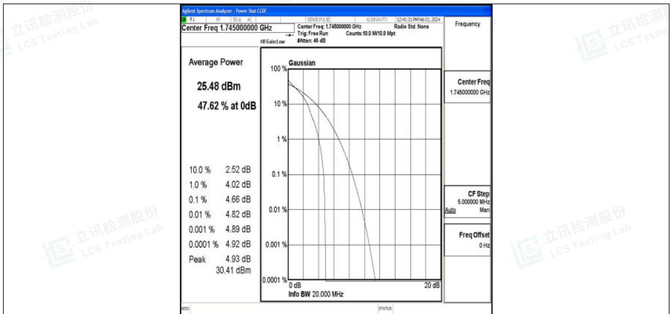
Band4-20MHz-QPSK-20300-1RB#0-PASS
