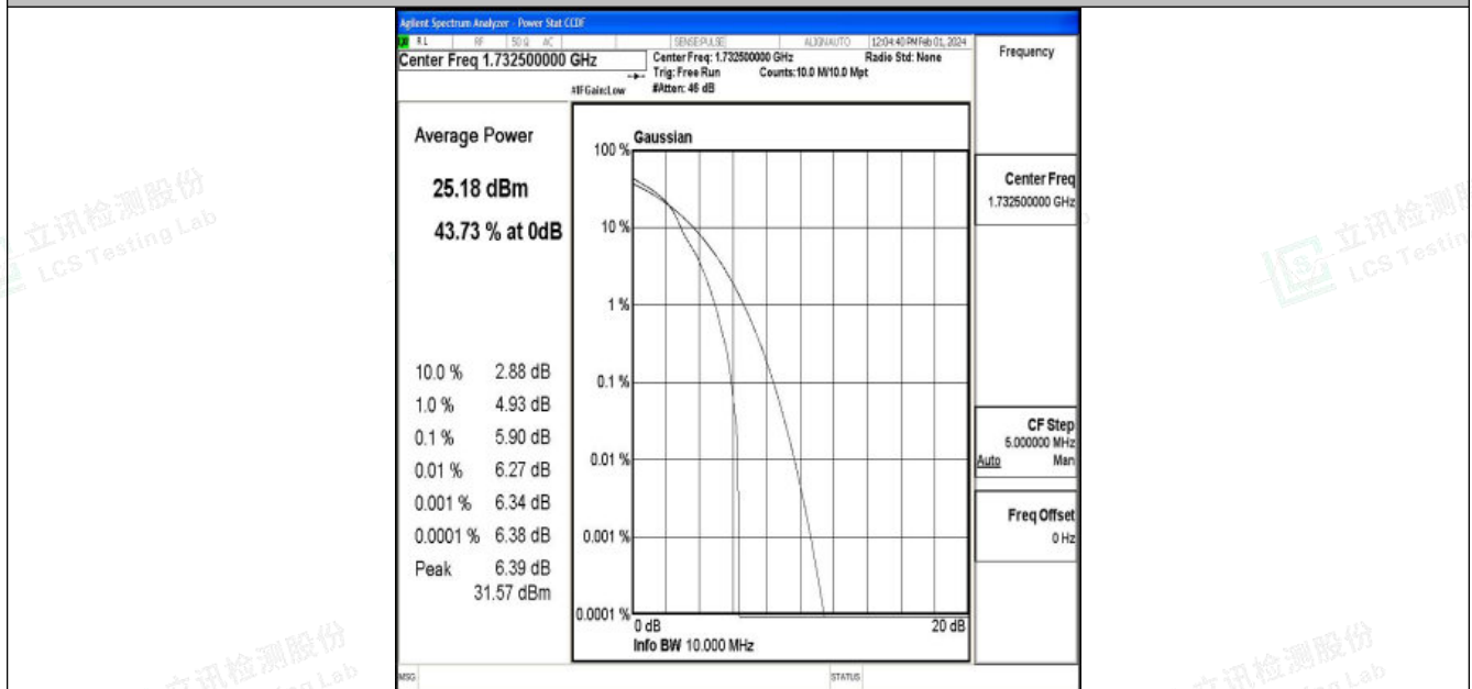
Band4-10MHz-16QAM-20175-1RB#0-PASS
