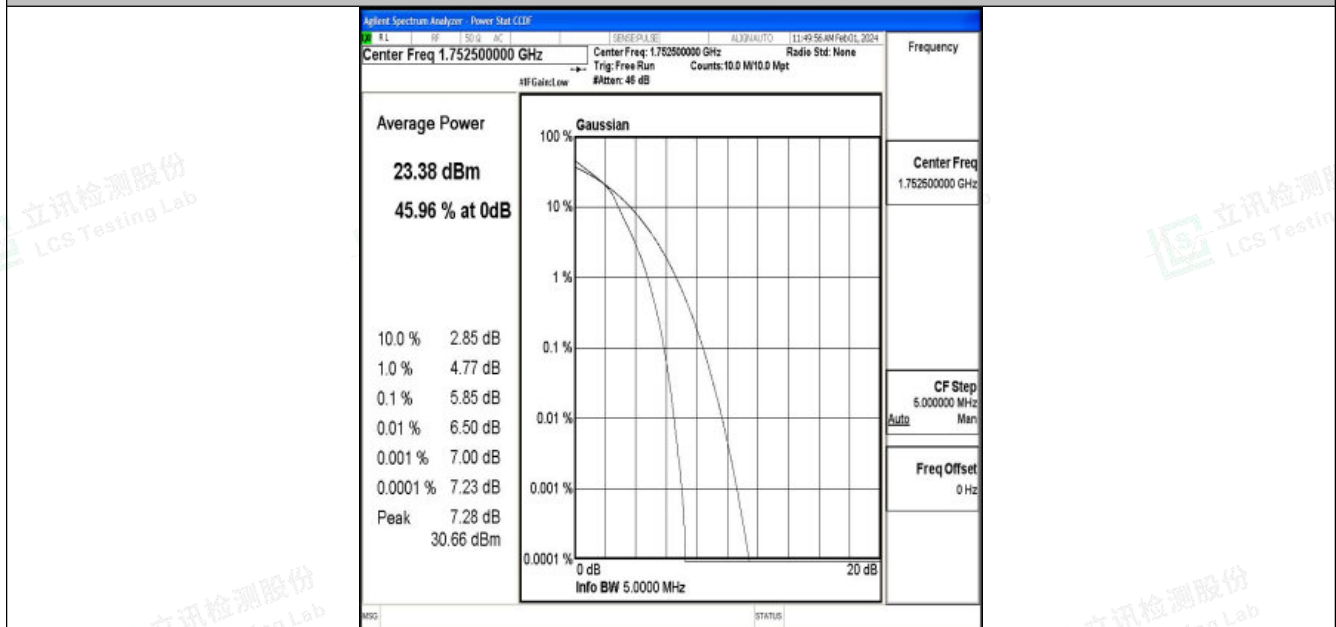
Band4-5MHz-16QAM-20375-25RB#0-PASS
