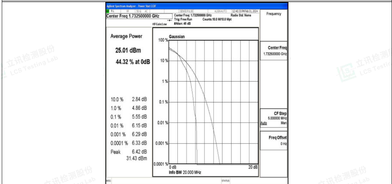
Band4-20MHz-16QAM-20175-1RB#0-PASS
