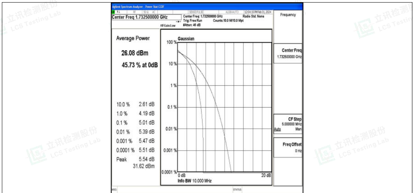
Band4-10MHz-QPSK-20175-1RB#0-PASS
