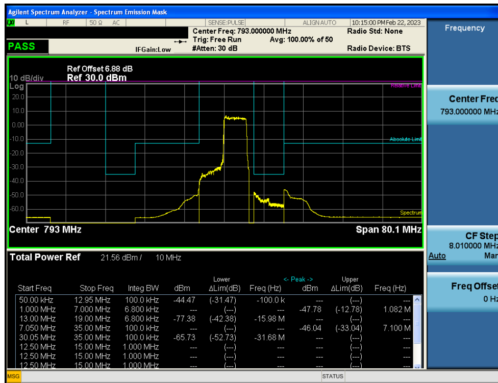
LTE Band 14 / 10MHz / QPSK - RB Size/Offset (25/25)
