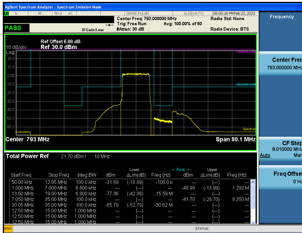
LTE Band 14 / 10MHz / QPSK - RB Size/Offset (50/0)
