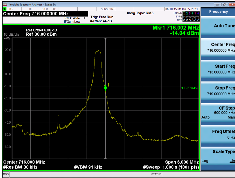
LTE Band 12 / 3MHz / QPSK - RB Size/Offset (1/14)
