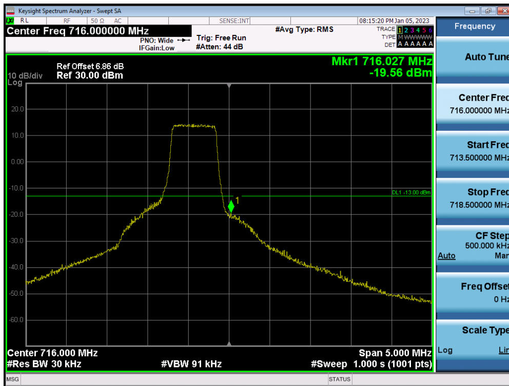
LTE Band 12 / 1.4MHz / 16QAM - RB Size/Offset (3/3)
