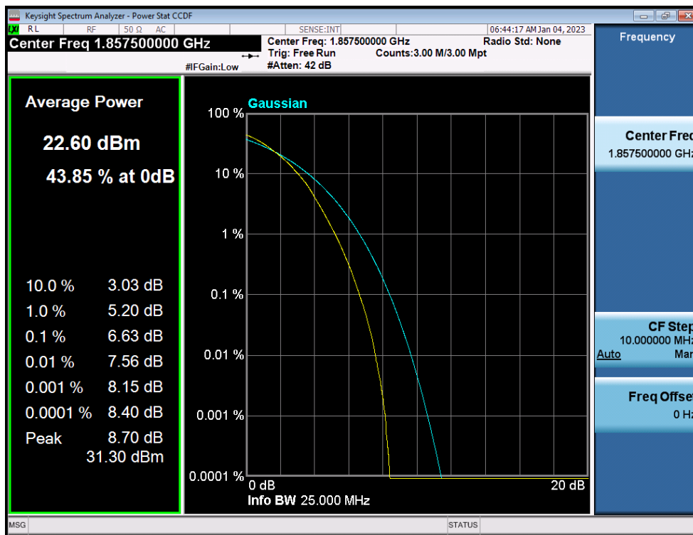
LTE Band 2 / 15MHz / 64QAM - RB Size 75
