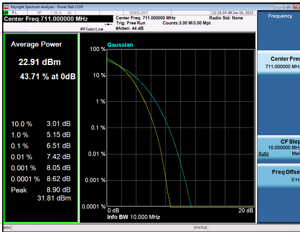
LTE Band 12 / 10MHz / 64QAM - RB Size 50
