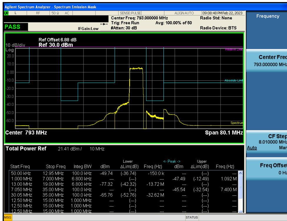
LTE Band 14 / 5MHz / QPSK - RB Size/Offset (25/0)
