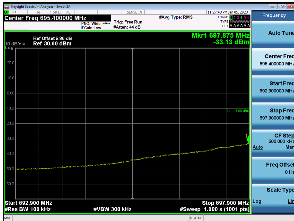
LTE Band 12 / 5MHz / 64QAM - RB Size/Offset (12/0)
