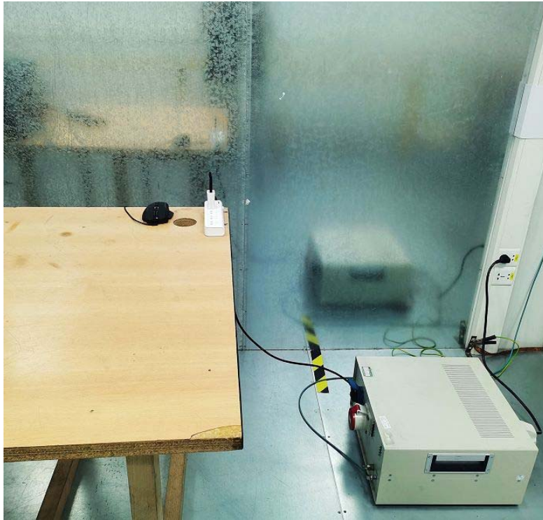
Conducted Emission Test Setup:
