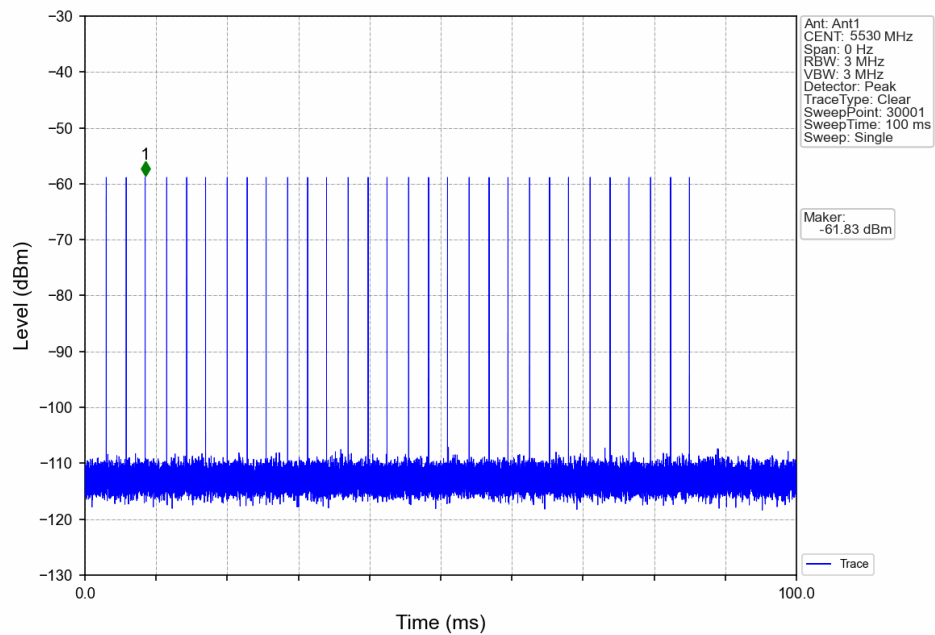
Signal Calibration_802.11 ac_2C_5530MHz_RadarType5_Trial0
