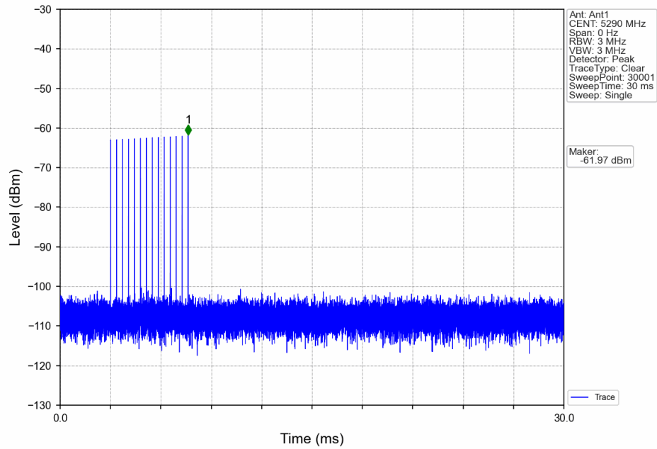
Signal Calibration_802.11 ac_2A_5290MHz_RadarType5_Trial0
