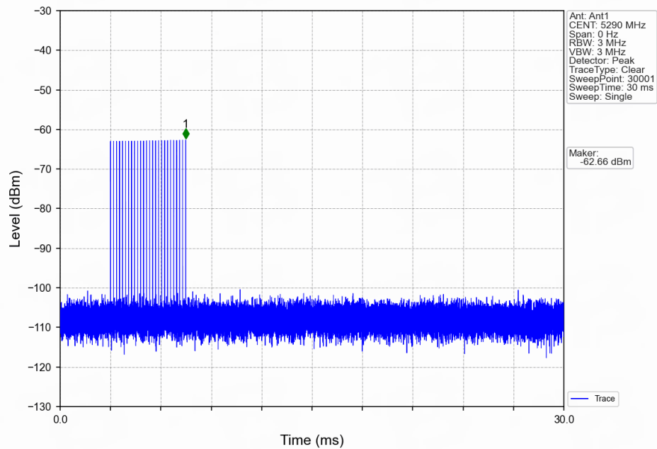
Signal Calibration_802.11 ac_2A_5290MHz_RadarType3_Trial0
