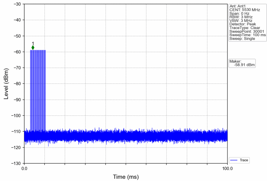
Signal Calibration_802.11 ac_2C_5530MHz_RadarType3_Trial0
