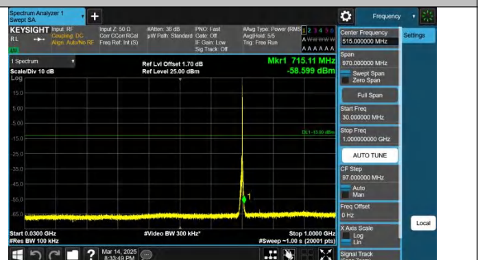
Band12-3MHz-QPSK-23095-1RB#14-30~1000-PASS
