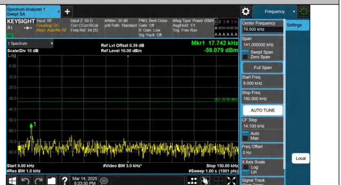
Band12-3MHz-QPSK-23095-1RB#14-0.009~0.15-PASS
