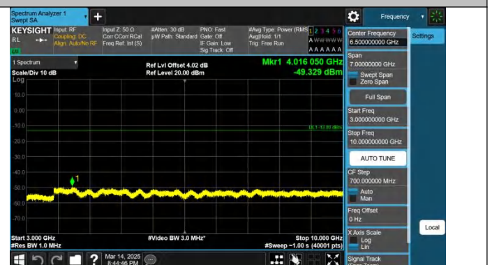
Band12-5MHz-QPSK-23095-1RB#24-3000~10000-PASS
