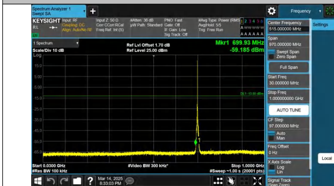
Band12-3MHz-QPSK-23095-1RB#0-30~1000-PASS
