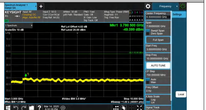
Band12-3MHz-QPSK-23025-1RB#14-3000~10000-PASS
