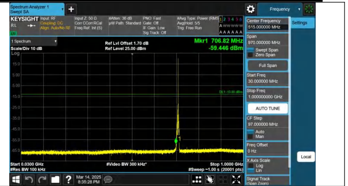
Band12-3MHz-QPSK-23165-1RB#14-30~1000-PASS
