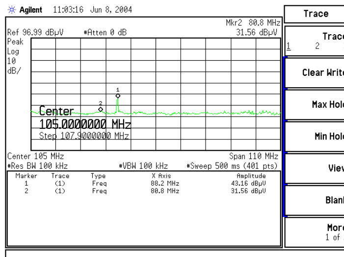
Figure 88.1 MHz: (Vertical)
