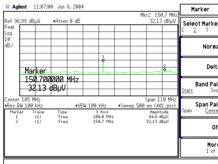
Figure 107.9 MHz: (Vertical)
