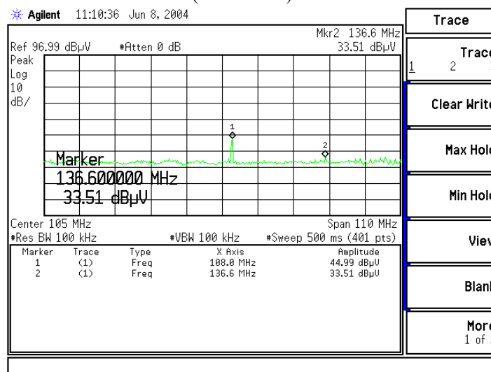
Figure 107.9 MHz: (Horizontal)
