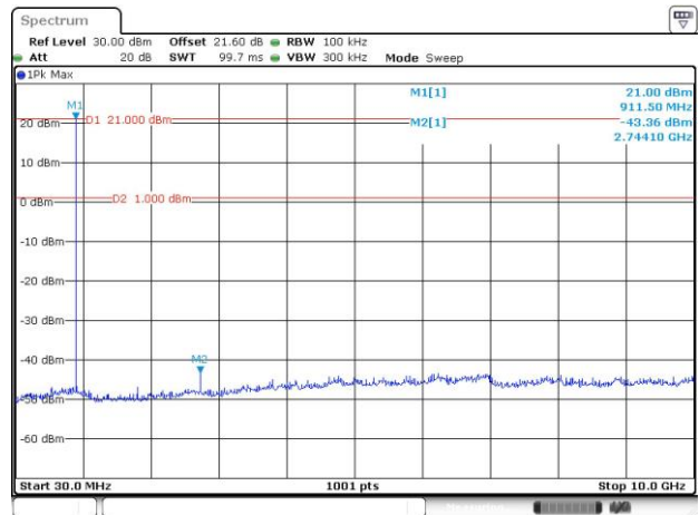
CSE Plot on Ch 32 between 30MHz ~ 10 GHz
