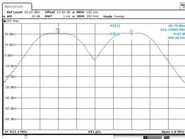
Channel Separation Plot on Channel 31 - 32
