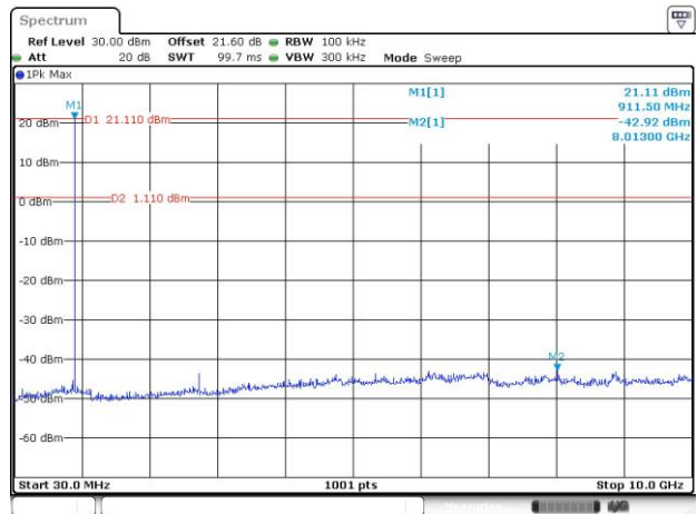
CSE Plot on Ch 26 between 30MHz ~ 10 GHz
