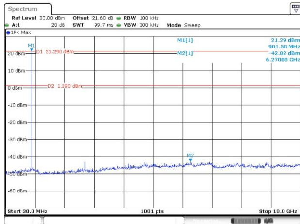
CSE Plot on Ch 01 between 30MHz ~ 10 GHz
