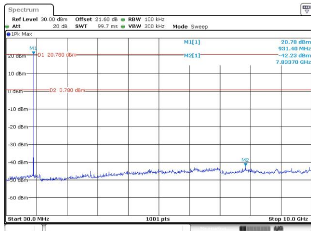
CSE Plot on Ch 51 between 30MHz ~ 10 GHz
