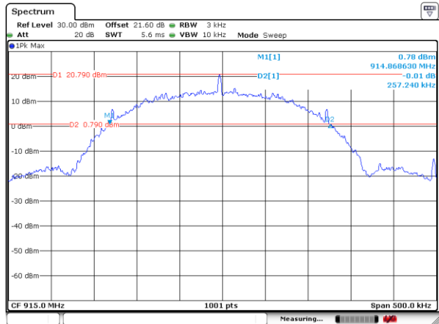
20 dB Bandwidth Plot on Channel 26
