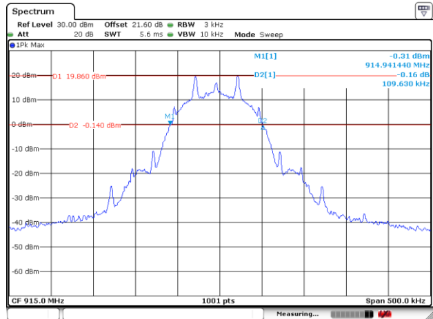
20 dB Bandwidth Plot on Channel 65
