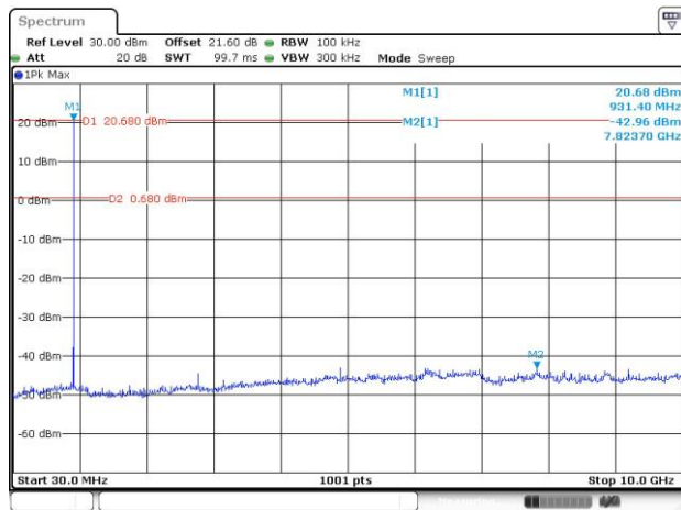
CSE Plot on Ch 64 between 30MHz ~ 10 GHz
