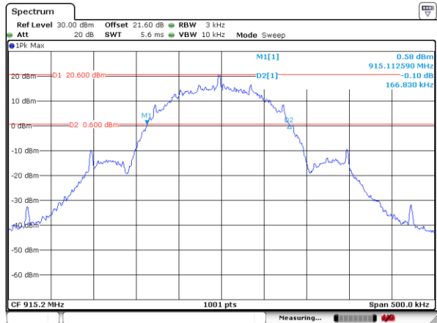
20 dB Bandwidth Plot on Channel 32
