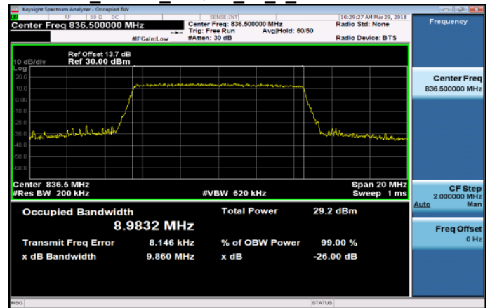
Band5_10MHz_16QAM_50_0_MidCH20525-836.5
