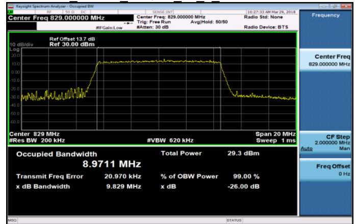
Band5_10MHz_16QAM_50_0_LowCH20450-829
