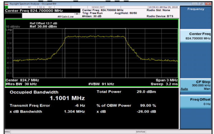
Band5_1_4MHz_16QAM_6_0_LowCH20407-824.7
