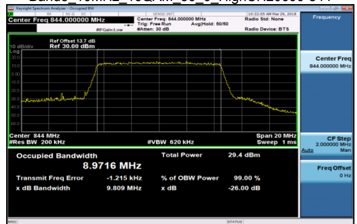
Band5_10MHz_16QAM_50_0_HighCH20600-844
