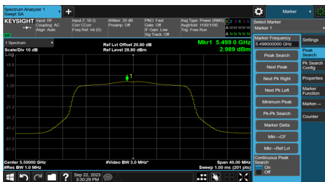
Channel 100 (5500MHz)
