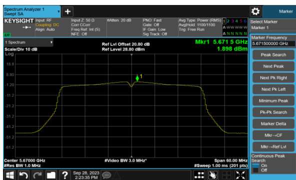
Channel 134 (5670MHz)
