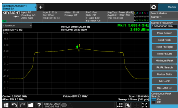
Channel 138 (5690MHz)
