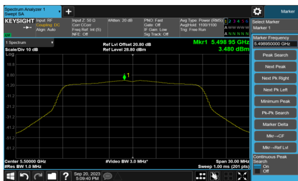
Channel 100 (5500MHz)
