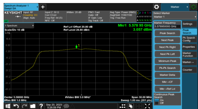
Channel 116 (5580MHz)
