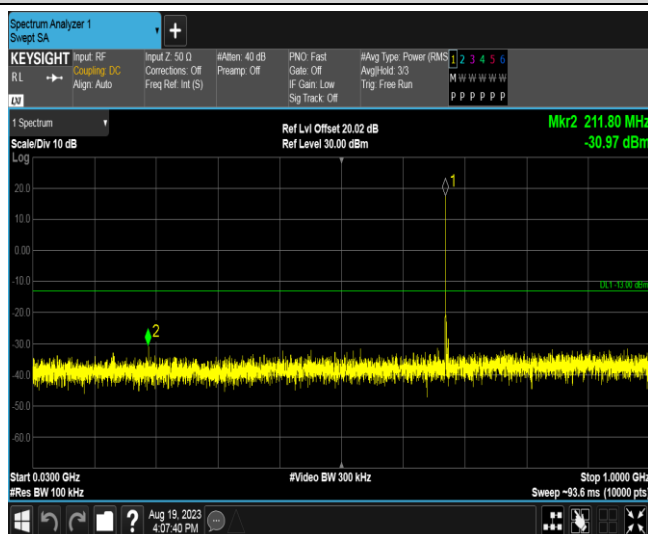
Band71-5MHz-16QAM-133297-1RB#0-Range1:30~1000MHz
