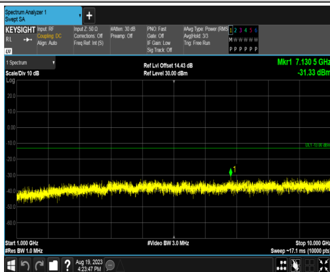
Band71-10MHz-16QAM-133422-1RB#0-Range2:1000~10000MHz
