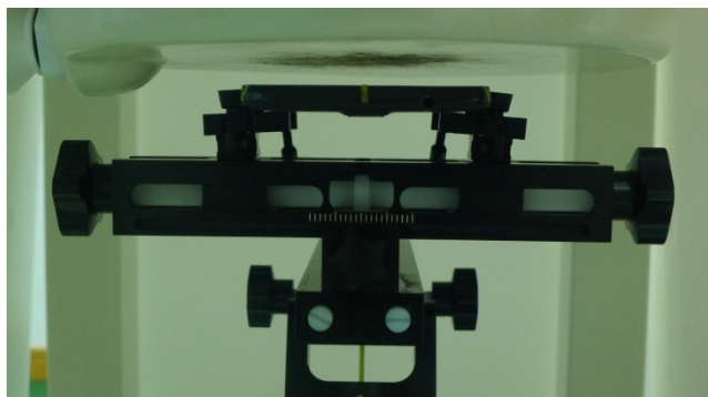
Front of the DUT with Phantom 1 cm Gap
