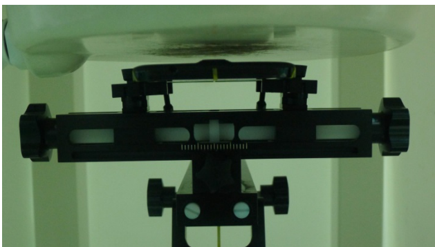
Back of the DUT with Phantom 1 cm Gap
