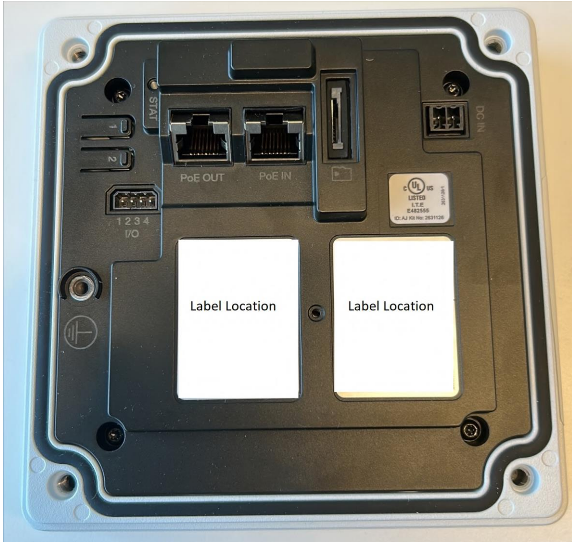
Back view of EUT with gasket and label location
