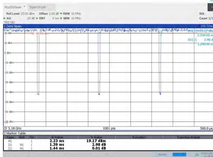
11N20SISO_Ant3_5180
