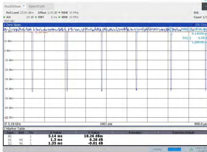
11N20SISO_Ant3_5180
