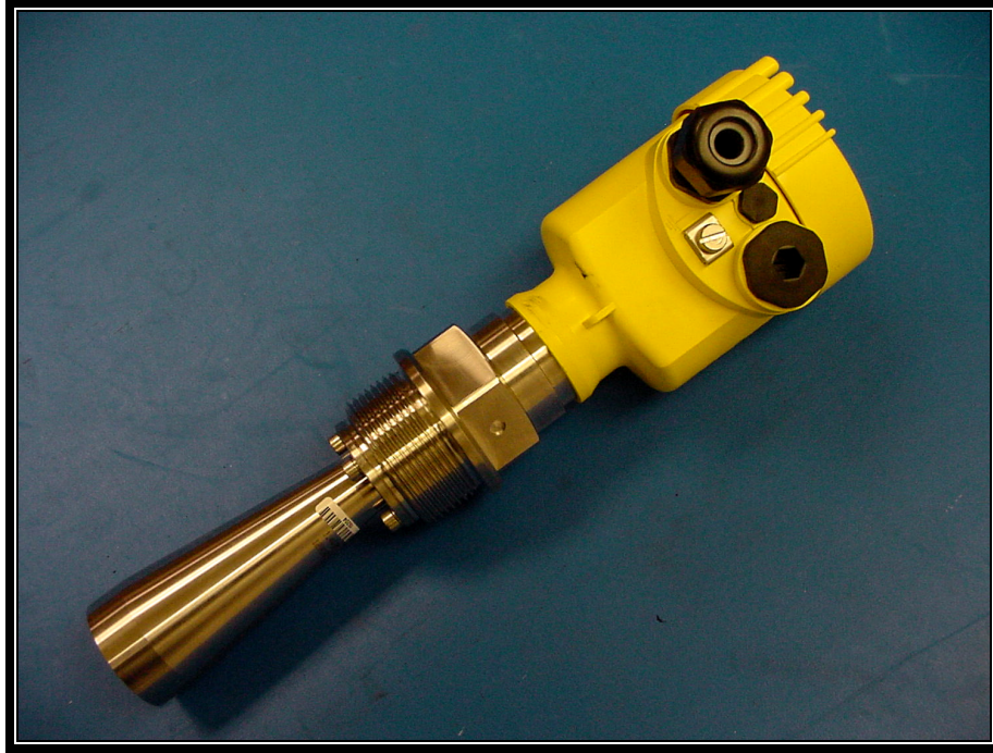
Photograph 28: EUT with 19 dBi Horn Antenna
