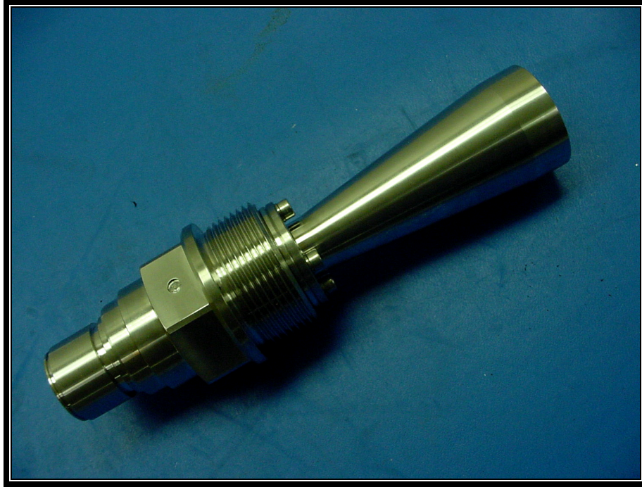
Photograph 29: 19 dBi Horn Antenna
