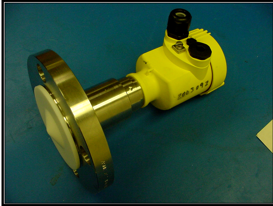
Photograph 30: EUT with 21.2 dBi Rod Antenna
