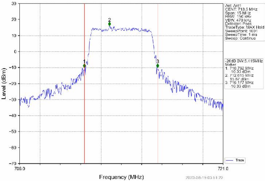
Band17_5MHz_16QAM_HCH_713.5MHz_RB_25_0_NTNV
