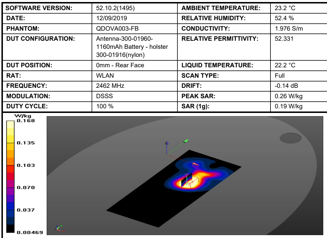
Figure 50: SAR Body Testing Results for the SC2124 at 2462 MHz.
