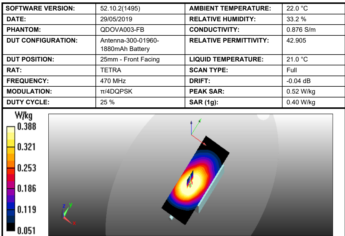
Figure 6: SAR Front Of Face Testing Results for the SC2124 at 470 MHz.
