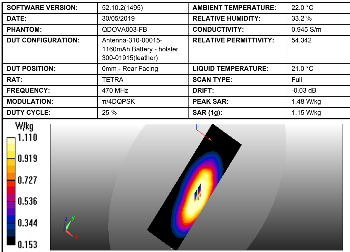
Figure 44: SAR Body Testing Results for the SC2124 at 470 MHz.
