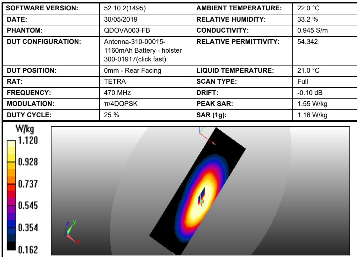
Figure 43: SAR Body Testing Results for the SC2124 at 470 MHz.
