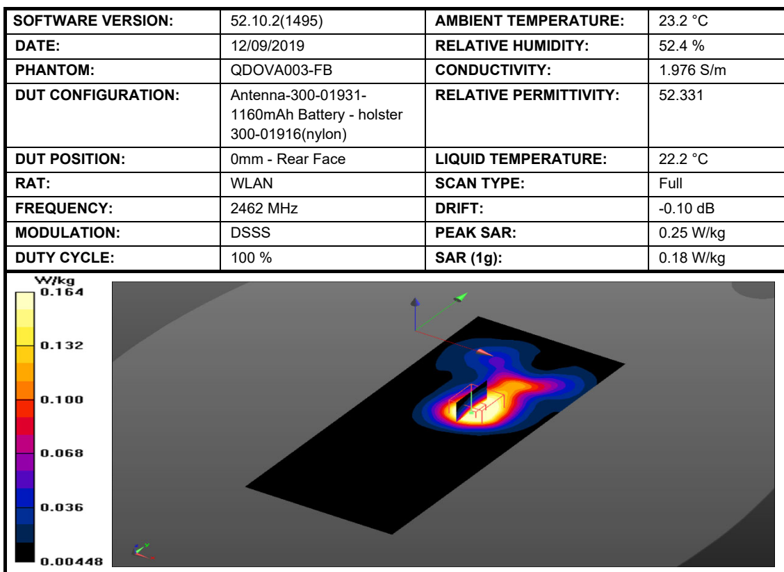
Figure 51: SAR Body Testing Results for the SC2124 at 2462 MHz.
