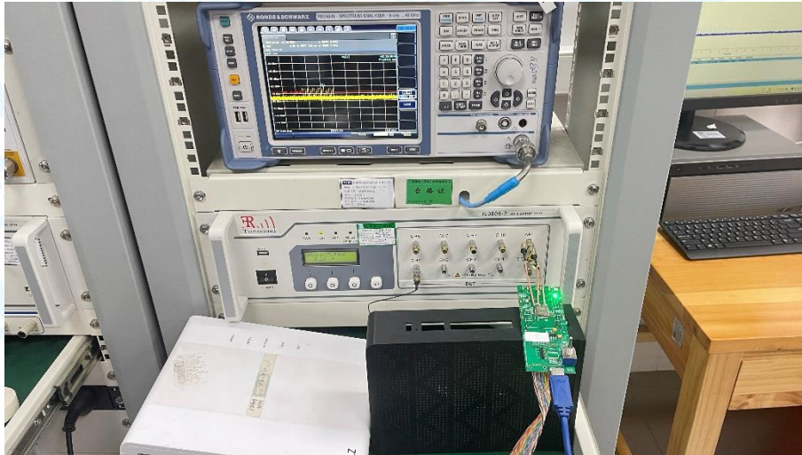
Photo of Setup for DFS Test
