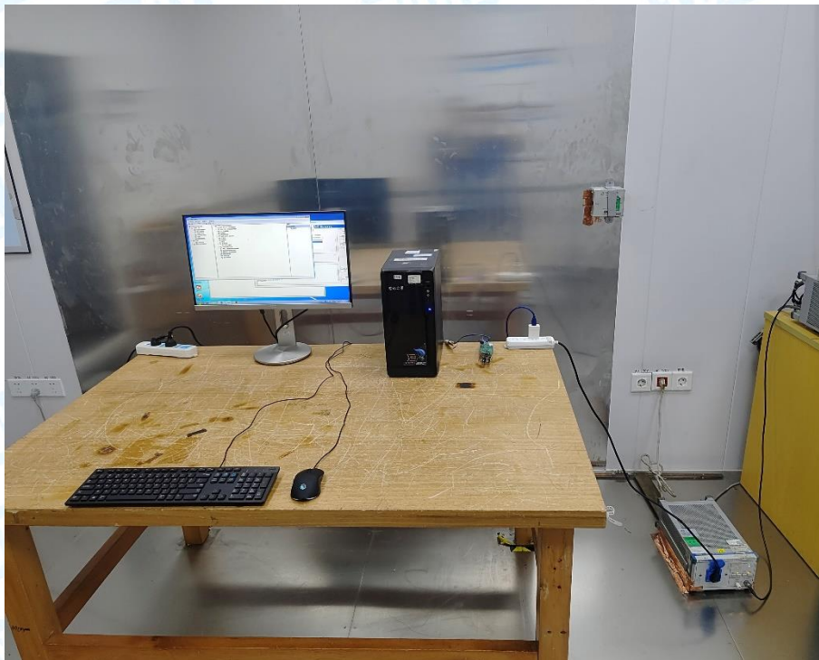
Photo of Setup for Radiated Emission (Below 1 GHz)
